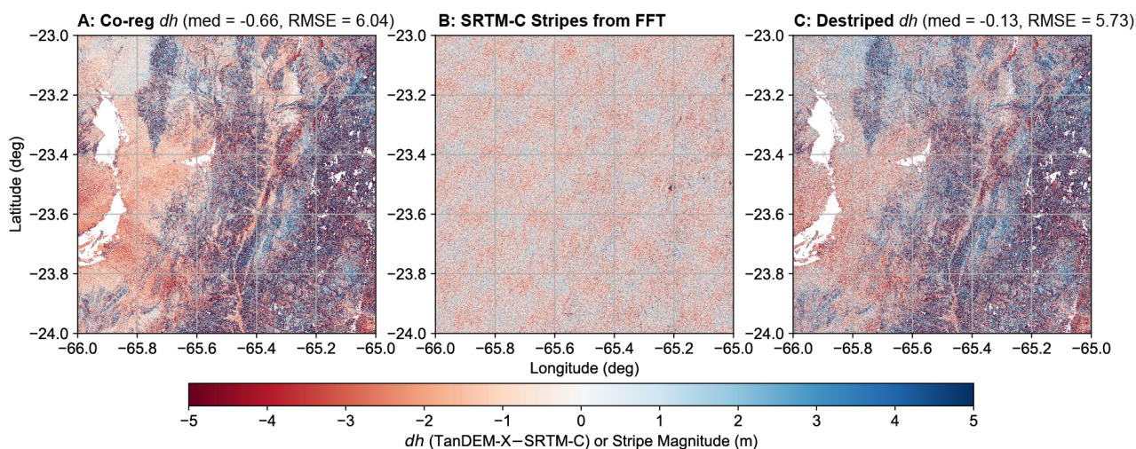
Figure 3. One iteration of FFT destriping from one tile (S 24°, W 66°). Both median and RMSE improve from (A) the co-registered map to (C) the destriped map. Stripes removed by FFT are shown in (B). Note that (C) is not the final corrected map as iteration was run twice more before RMSE began to converge at 5% tolerance level. Voids (white space) are untrustworthy pixels removed by TanDEM-X WAM cutoff prior to destriping.
