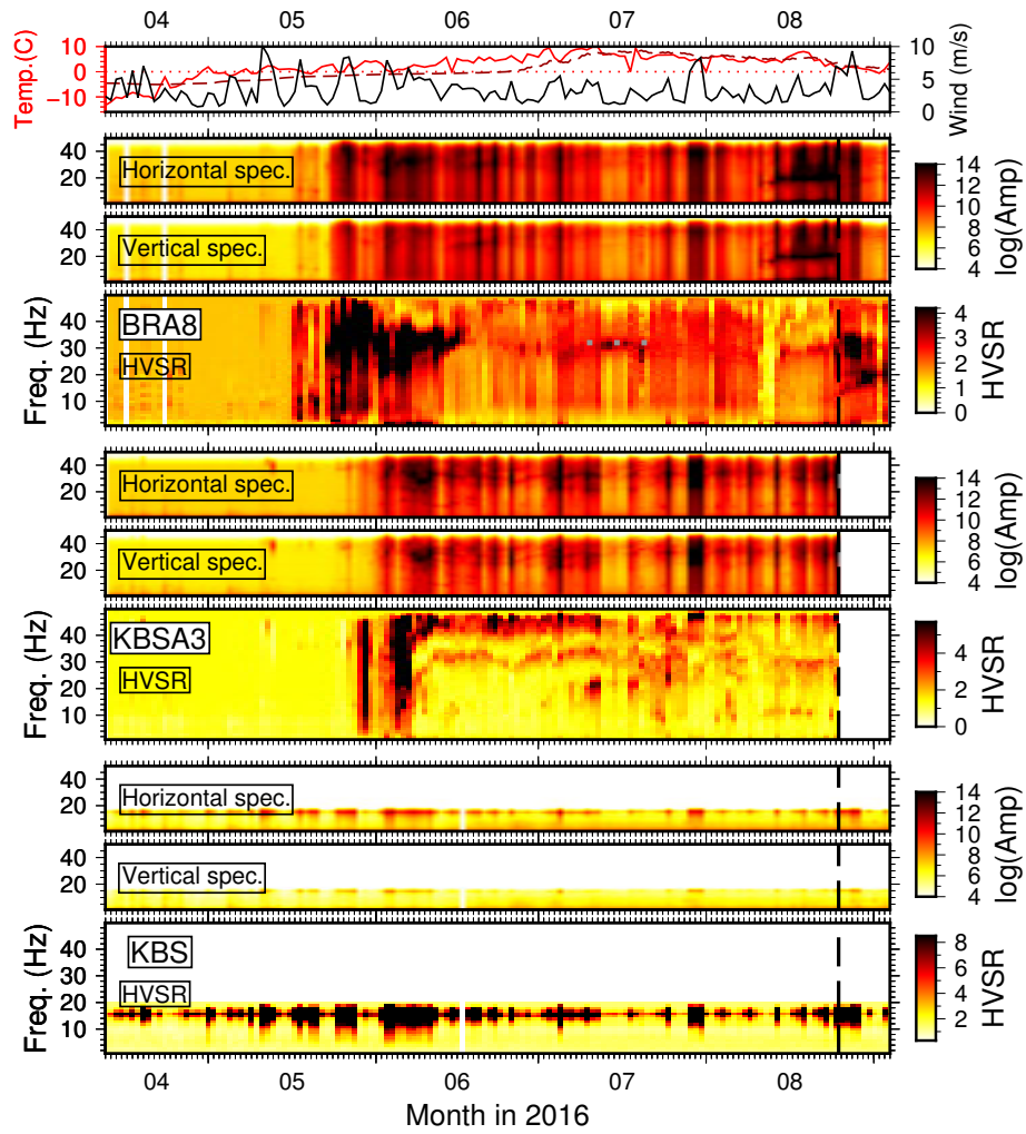
Figure A3. Same as Fig. 2 for three more stations.
