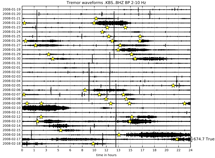
Figure A4. Example of repeating seismic tremor waveforms recorded at KBS. Detected tremor onsets are indicated by yellow stars. Waveform data of the tremor on 2008-01-22 are provided in the supplement S01.
