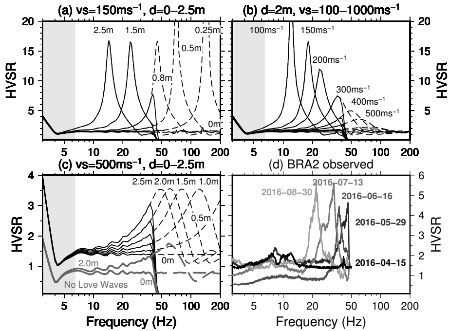
Figure 4. (a)–(c) Theoretical Horizontal-To-Vertical Spectral Ratios (HVSRs) modeled using the diffuse wavefield method and sub-surface models of increasing thaw depth d or S-wave velocity vs in the active layer. Reference model in Table 1 is modified accordingly. Black models include Rayleigh, Love and body waves. Gray models in (c) include no Love waves. Gray area indicates tremor frequency band (see Section 5). Dashed curves are modeled HVSRs above Nyquist frequency without using anti-aliasing filter of field instruments. (d) Measured HVSRs at station BRA2 at four different days showing a peak gliding to lower frequencies.
