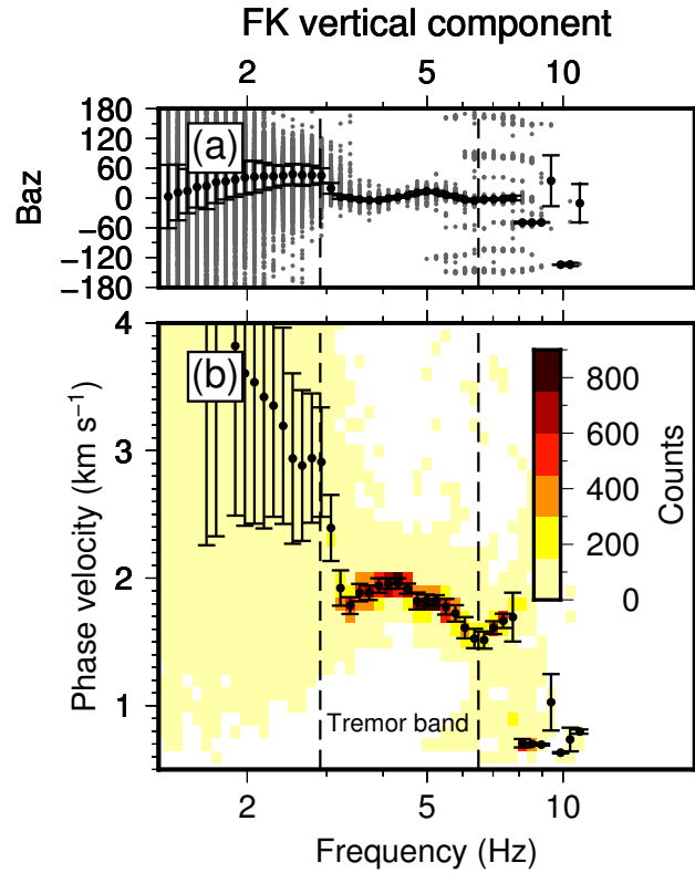
Figure A6. Example of frequency-wavenumber (FK) analysis of vertical components of KBS array for tremor occurring between 2016-05-12T03:02:00 and 2016-05-12T06:17:00. (a) All back-azimuth (Baz) measurements at maximum beampower and with coherency (normalized beampower) > 0.7 for 600 s long time windows during tremor occurrence (gray symbols) and median with median deviation (black). (b) Color-coded histogram (counts) of phase velocity measurements for same time windows as in (a) and median with median deviation.
