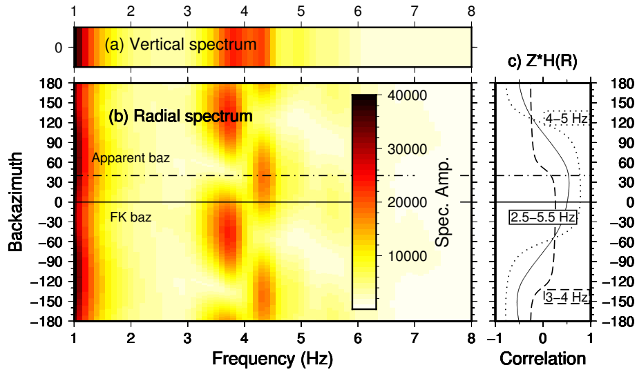
Figure 6. (a) and (b) Example amplitude frequency spectra at KBS for tremor occurring between 2016-05-12T03:02:00 and 2016-05-12T06:17:00 for vertical and radial component assuming different back-azimuth values. (c) Correlation coefficient between vertical and Hilbert-transformed radial component assuming different back-azimuth values in different frequency bands. High values are expected in case of Rayleigh waves on the radial component. Tremor backazimuth from vertical FK analysis (FK baz) and apparent backazimuth corresponding to maximum correlation between 4 and 5 Hz (Apparent baz) are indicated. Discrepancy is probably due to azimuthal anisotropy.
