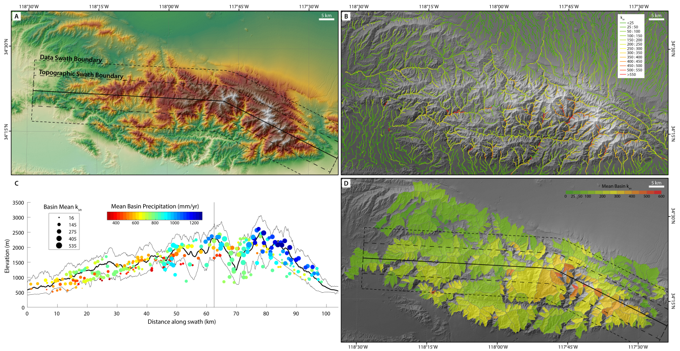
Figure 2 Example products output from TAK (with some compilation in ArcGIS and editing in a graphics program). A) Shaded elevation map of the San Gabriel Mountains in southern California with outlines of a combined swath profile. B) Normalized channel steepness map from KsnChiBatch. C) Swath profile with 10 km sampling width for the topography and 20 km sampling width for the basin data, basins are located based on their centroid location and mean elevation, colored by their mean annual precipitation averaged from 1981-2010 (data from PRISM Climate Group, Oregon State University, http://prism.oregonstate.edu , downloaded 1 June 2018), and scaled by their mean k_{sn} . D) Map of basin averaged k_{sn} using ProcessRiverBasins and SubDivideBigBasins (using the trunk division method and a max basin size of 25 km 2 )
