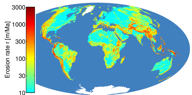
Figure 4. World map of the erosion rates obtained in this study.
