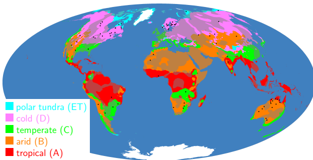
Figure 2. The primary Köppen-Geiger climate classes (Peel et al., 2007) considered in this study. Solid colors correspond to the predominantly erosive provinces (shield, orogen, igneous), while the respective pale colors mark those regions not considered in order to avoid a bias by sediment deposition. The black dots show the 77 craters with diameters D \geq 0.25 km located in the predominantly erosive provinces being the basis of our analysis.
