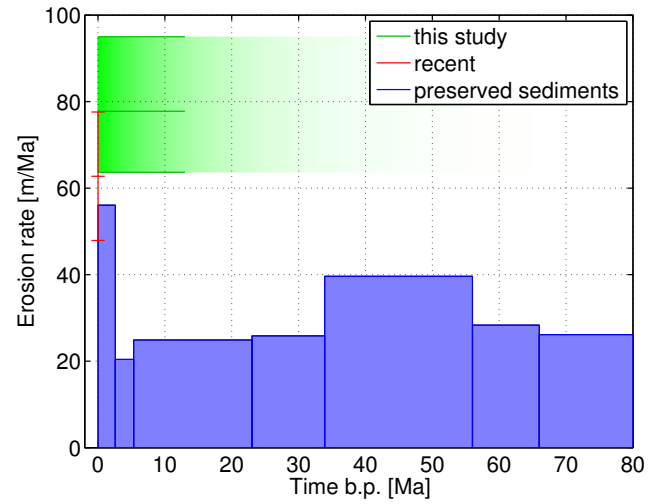
Figure 8. Comparison of our worldwide long-term mean erosion rate with estimates obtained from preserved sediments (Wilkinson and McElroy, 2007) and recent erosion rates compiled by Willenbring et al. (2013). The green area represents our result for the mean erosion rate of r = 78 m/Ma with 70 % confidence intervals. The decreasing opacity visualizes the exponentially decreasing sensitivity with \tau = 13 Ma.
