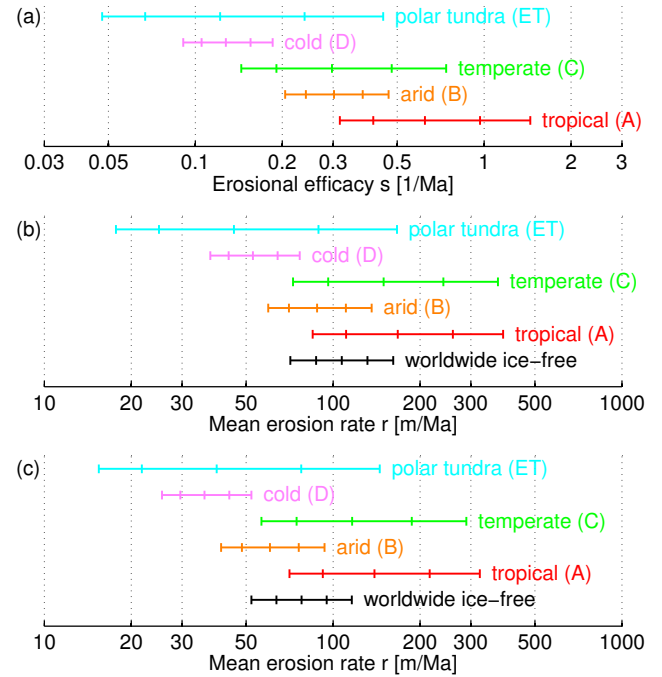
Figure 3. Erosion rates by climatic zones. (a) Mean erosional efficacies of the primary Köppen-Geiger classes. (b) Respective absolute mean erosion rates for the predominantly erosive provinces. (c) Absolute mean erosion rates extrapolated to the entire ice-free surface including the classes platform, basin, and extended crust. Error bars represent 70 % confidence intervals (corresponding to the standard deviation for a Gaussian distribution) and 95 % confidence intervals (see Appendix A).
