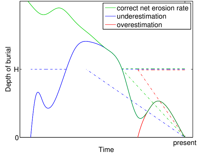
Figure 11. Three scenarios of intermittent phases of sedimentation. Solid curves: depth of burial of the present-day surface. Dashed lines: time intervals of crater production where a crater of a given depth H would be detectable at the present surface. Dotted lines: equivalent erosional histories (same expected number of craters) with constant erosion rates.
