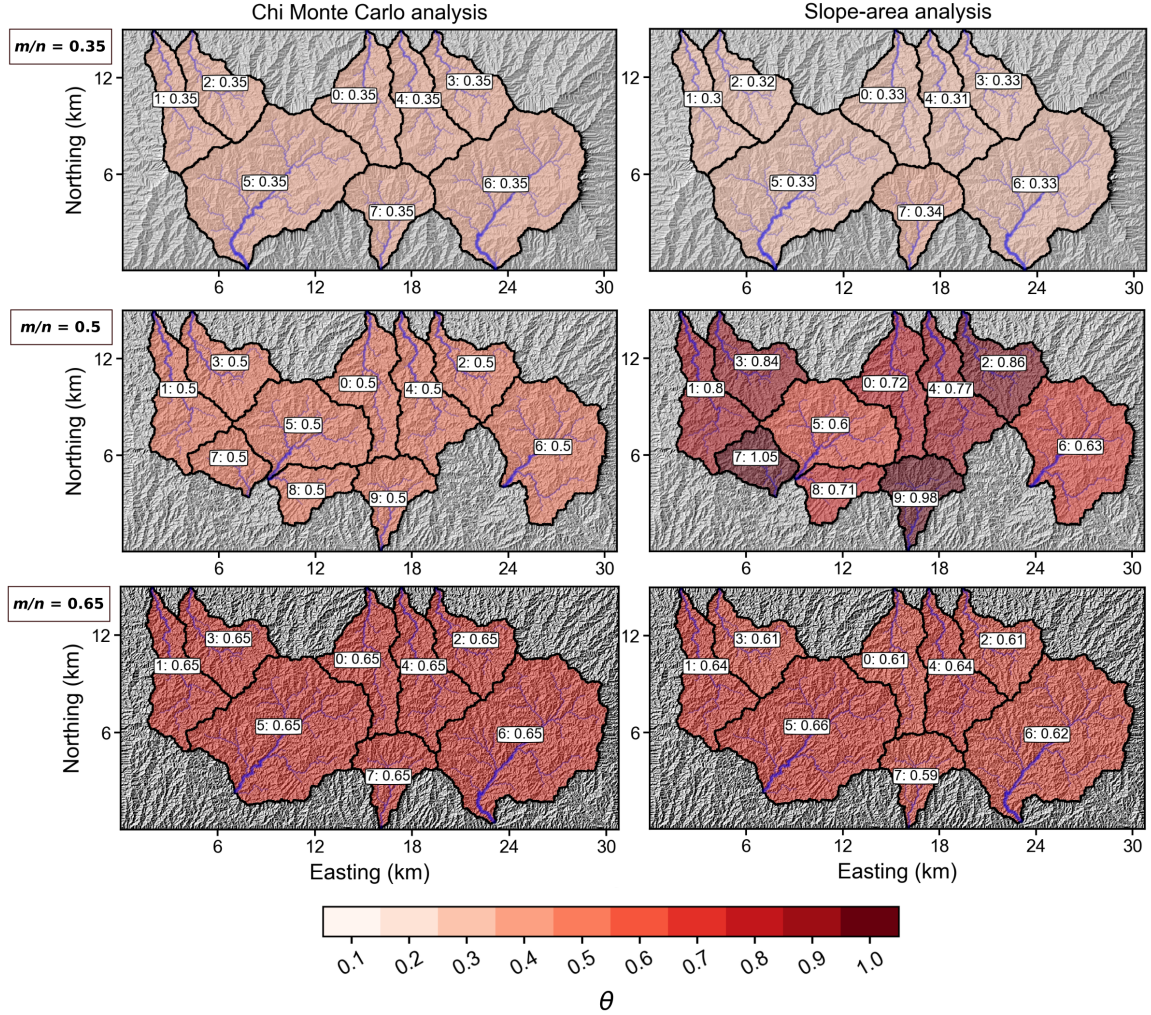
Figure 5. Shaded relief plots of the model runs with temporally varying uplift, with drainage basins plotted by the best fit \theta predicted from the \chi bootstrap analysis (first column), and slope–area analysis (second column). Each row represents a model run with a different m/n ratio. The basins are coloured by the predicted \theta , where darker colours indicate a higher concavity index. The extracted channel network for each basin is shown in blue.
