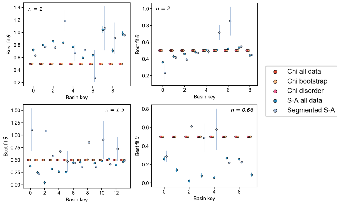
Figure 6. Plots showing the predicted best fit \theta for each basin and each method for m/n = 0.5 , where n = 1, n = 2, n = 1.5 , and n = 0.66 . The \chi methods are shown in reds and the slope–area methods are shown in blues.
