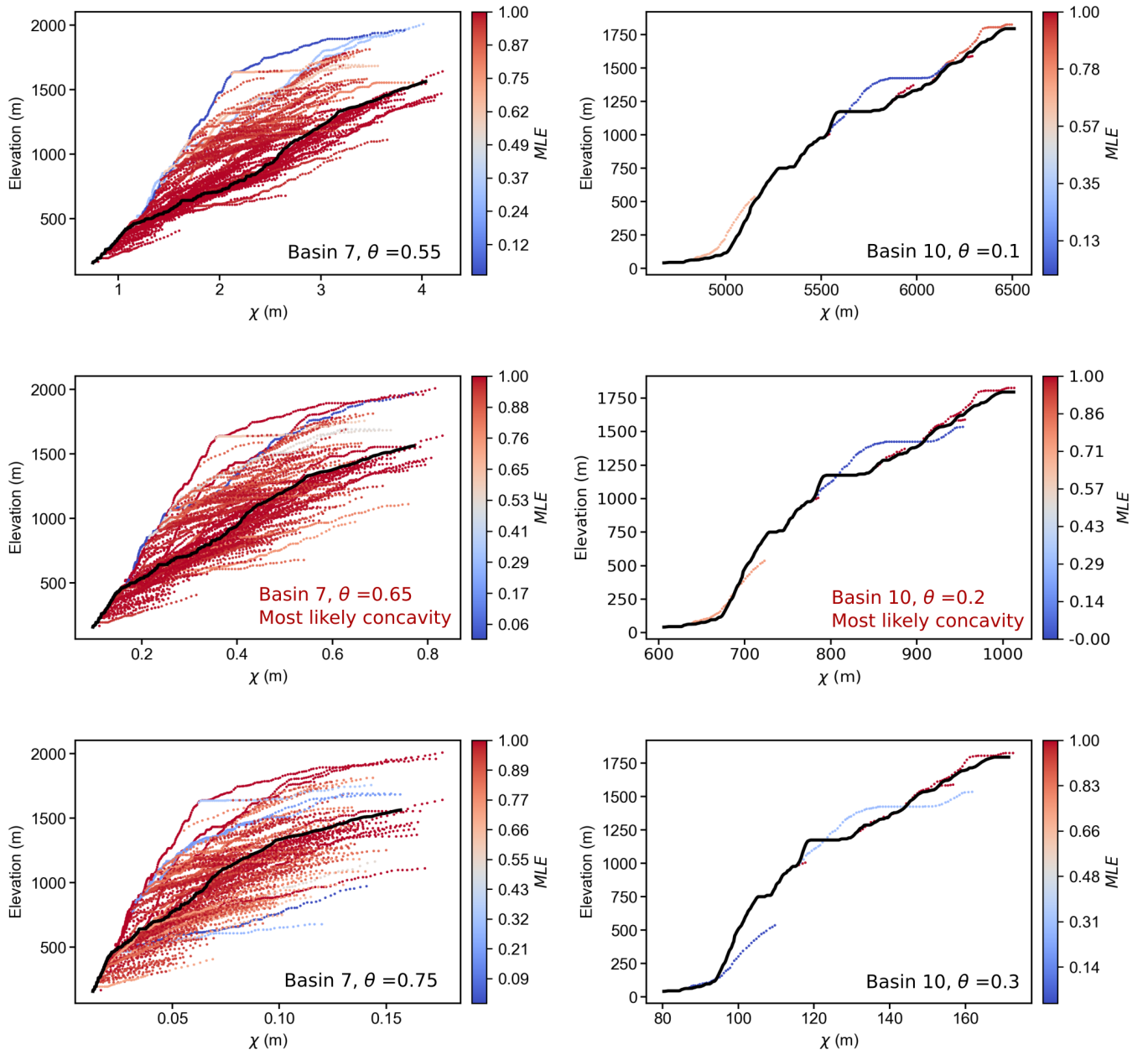
Figure 13. Profile \chi –elevation plots associated with best fit \theta for Basin 7, a large catchment with many tributaries draining across a relay zone between normal fault segments (left column), and Basin 10, a small, steep catchment draining directly across the footwall segment of a normal fault with few tributaries (right column). Note that MLE values depend on both the number of nodes and the vertical offset from the trunk channel.
