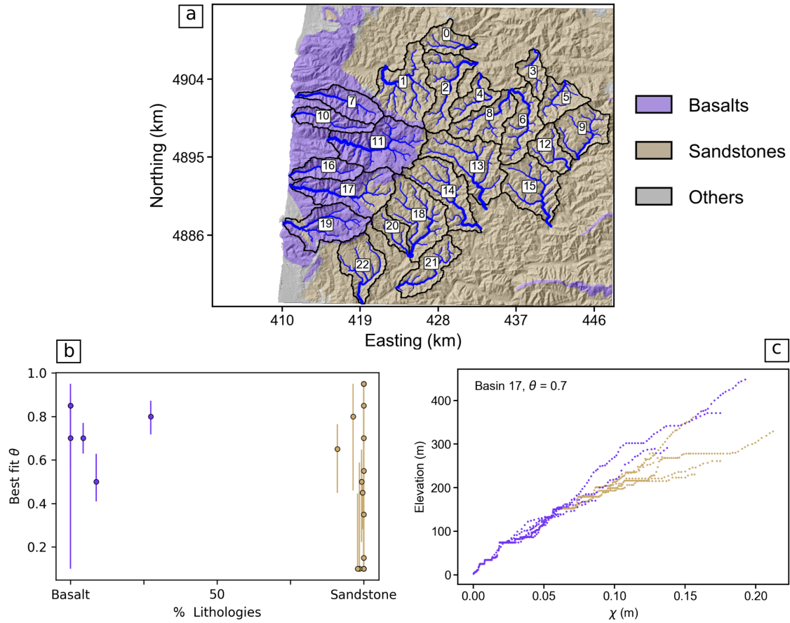
Figure 10. Exploration of the most likely concavity index near Waldport, Oregon, UTM Zone 10N. Basins numbers and the underlying lithology is displayed in panel a. . The most likely concavity index determined by the bootstrap method as a function of the percent of each basin in the different lithologies is shown in panel b. Panel c. shows the \chi -elevation plot for a basin that has two bedrock types; the channel pixels are coloured by lithology. The plot uses the typical concavity index for basalt (0.7).
