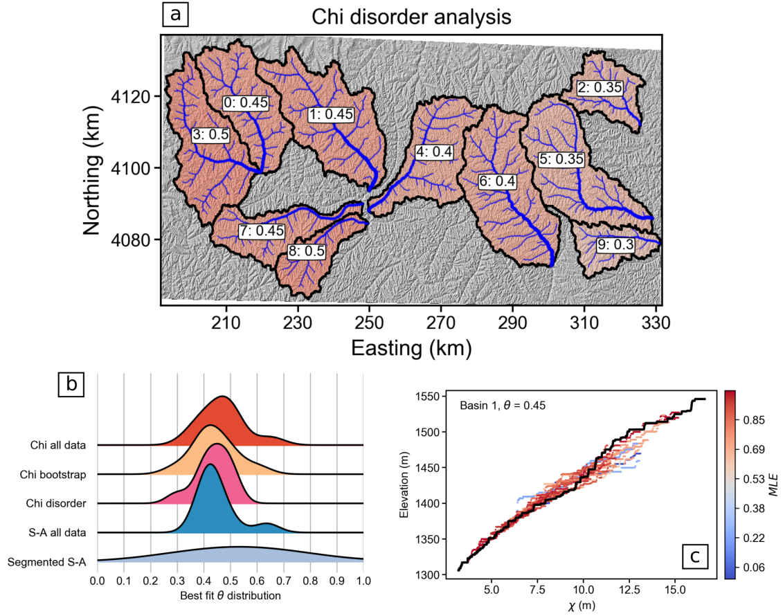
Figure 9. Exploration of the most likely concavity indices in the Loess Plateau, China, UTM Zone 49N. Basins with the most likely concavity index determined by the disorder method are displayed in panel a ; the basin number is followed by the most likely concavity index in the basin labels. The probability density of best fit concavity index for all the basins (i.e., not the uncertainty within individual basins but rather the probability distribution of the best fit concavity indices of all the basins) b . In basin 1, the most likely concavity index determined by the bootstrap and disorder methods is 0.45 and the \chi -elevation plot for this concavity index is shown in panel c .
