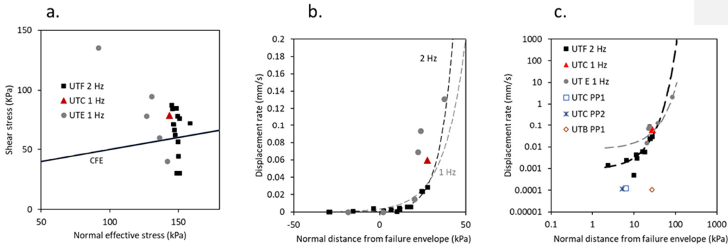
Figure 109: Results of dynamic shear experiments undertaken at 1 Hz and 2Hz (a) Average normal effective stress against maximum shear stress in relation to the conventional failure envelope (CFE) (b) Displacement rate against normal distance from the failure envelope (c) Displacement rate against normal distance from the failure envelope in log scale including pore pressure experiments.
