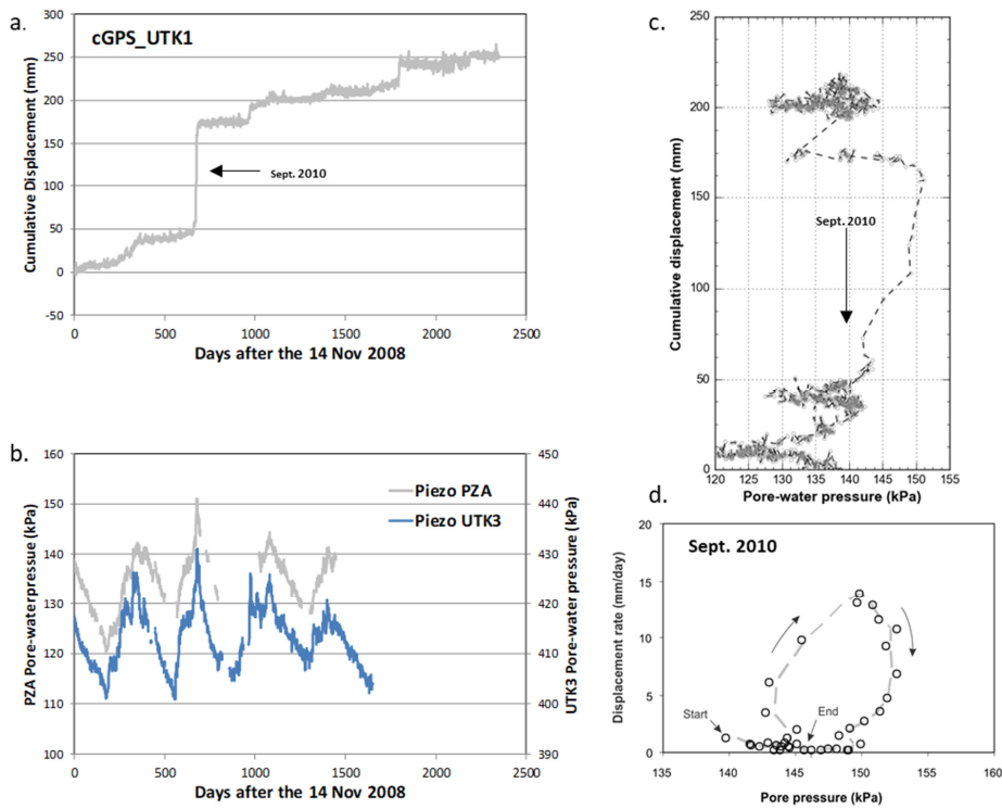
Figure 2: Utiku Landslide monitoring (a) Displacement of the continuous GPS (CGPS) UTK1 receiver, showing the cumulative displacement along bearing 154 degrees (the main direction of movement), from 14 November 2008 to 20 April 2015. Note all displacements are regionally filtered relative to the displacement of CGPS UTKU, which is located off the landslide. (b) Pore-water pressures recorded above the slide plane in piezometers PZA and UTK3. (c) Cumulative displacement of cGPS_UTK1 along bearing 154 degrees and the daily pore-water pressure recorded in piezometer PZA, plotted in chronological order. (d) Displacement rate estimated along the horizontal bearing 154 degrees for CGPS_UTK1 for the movement period in September 2010, and the corresponding pore-water pressures recorded at piezometer PZA. All figures are taken and modified from Massey (2010) and Massey et al. (2013).
