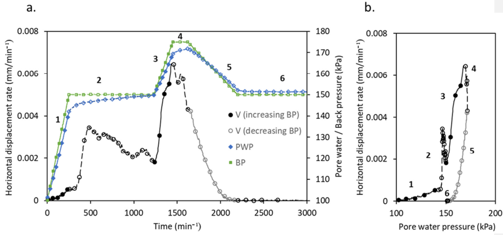
Figure 7: Relationship between shear surface displacement rate (V) and porewater pressure (PWP) during stepped pore pressure re-inflation (BP) experiment conducted at mean effective stresses of 150 kPa (UTC PP2) for periods of increasing back pressure (solid symbols), constant back pressure (hollow symbols) and decreasing back pressure (a) Horizontal displacement rate against time in relation to the applied back pressure (BP) and measured pore water pressure (PWP) experiment UTC PP2 (b) Horizontal displacement rate against pore water pressure experiment UTC PP2.
