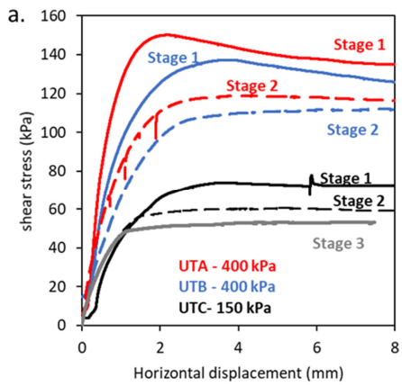
Figure 5: Conventional monotonic drained shear tests (a) stress strain behaviour. (b) monotonic drained failure envelope.
