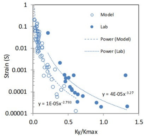
Figure 110: Strain versus K_y/k_{max} ratios from numerical simulations (hollow circles) and laboratory experiments (solid circles). a) strain at given ratios of the yield acceleration (KY) to the maximum of the average acceleration of the mass ( k_{max} ), in response to a given dynamic load adopting the piezometric “base levels” derived from field monitoring of piezometric head levels in the landslide.
