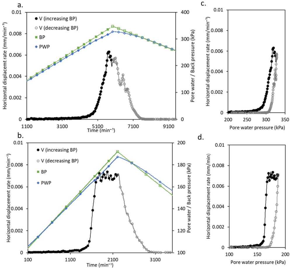
Figure 6: Relationship between shear surface displacement rate (V) and porewater pressure (PWP) during linear pore pressure reflation experiments conducted at mean effective stresses of 400 kPa (UTB PP1) and 150 kPa (UTC PP1) (a) Horizontal displacement rate against time in relation to the applied back pressure (BP) and measured pore water pressure (PWP, experiment UTC PP1) (b) Horizontal displacement rate against time in relation to the applied back pressure (BP) and measured pore water pressure (PWP, experiment UTB PP1) (c) Displacement rate against pore water pressure, experiment UTB PP1 (d) Displacement rate against pore water pressure, experiment UTC PP1.
