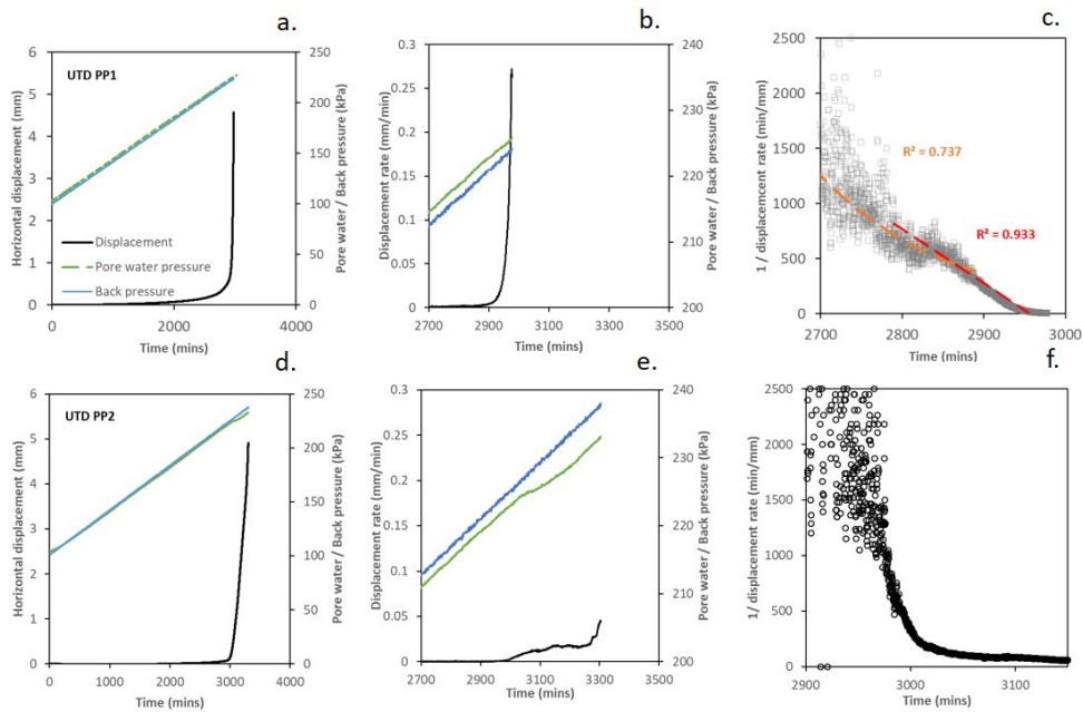
Figure 4: Shear surface displacement behaviour during linearly increase back pressure (applied pore water pressure) on intact (UTD PP1) and remobilised (UTD PP2) shear surface (a) Horizontal displacement against time in relation to the applied back pressure and measured pore water pressure, experiment UTD PP1 (b) Horizontal displacement rate against time in relation to the applied back pressure and measured pore water pressure, experiment UTD PP1 (c) 1/displacement rate against time, experiment UTD PP1 (d) Horizontal displacement against time in relation to the applied back pressure and measured pore water pressure, experiment UTD PP2 (e) Horizontal displacement rate against time in relation to the applied back pressure and measured pore water pressure, experiment UTD PP2 (f) 1/displacement rate against time, experiment UTD PP2.
