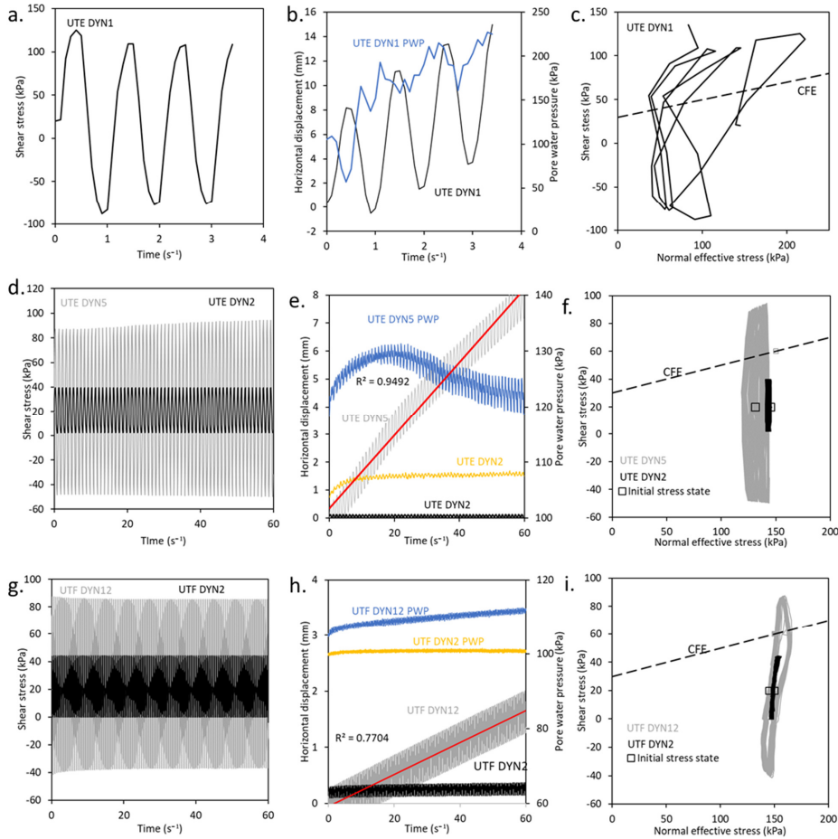
Figure 9: Dynamic shear experiments (a) Dynamic shear stress cycles applied at 1 Hz during experiment UTE DYN1 (b) Displacement and pore-water pressure response measured during experiment UTE DYN1 (c) Sample stress paths in relation to the conventional failure envelope (CFE) during experiment UTE DYN1 (d) Dynamic shear stress cycles applied at 1 Hz experiment UTE DYN2 and UTE DYN5 (e) Displacement and pore-water pressure response measured during experiments UTE DYN2 and UTE DYN5 (f) Sample stress paths in relation to the conventional failure envelope (CFE) during experiments UTE DYN2 and UTE DYN5 (g) Dynamic shear stress cycles applied at 2 Hz during experiment UTF DYN2 and UTF DYN12 (h) Displacement and pore-water pressure response measured during experiments UTF DYN2 and UTF DYN12 (i) Sample stress paths in relation to the conventional failure envelope (CFE) during experiments UTF DYN2 and UTF DYN12.
