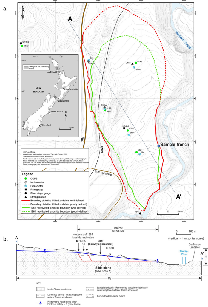
Figure 1: (a) Location of the Utiku landslide in North Island New Zealand, the location of monitoring equipment installed on the landslide in September 2008 and the location of the trench from which samples of the slide surface were taken. (b) Cross section A-A' through the landslide, refer to A) for the location of the section. Note 1: Slide plane formed within a thin (10-20 mm) layer of smectite-rich clay.
