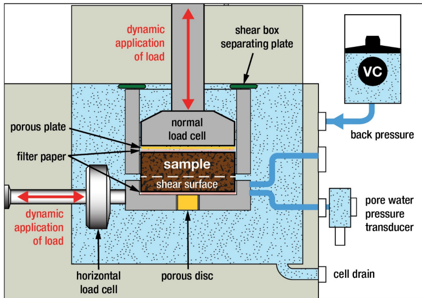
5 Figure 3: Schematic diagram of the dynamic back pressured shear box
