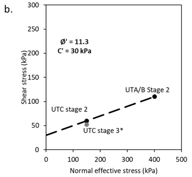
Figure 5: Conventional monotonic drained shear tests (a) stress strain behaviour. (b) monotonic drained failure envelope.
