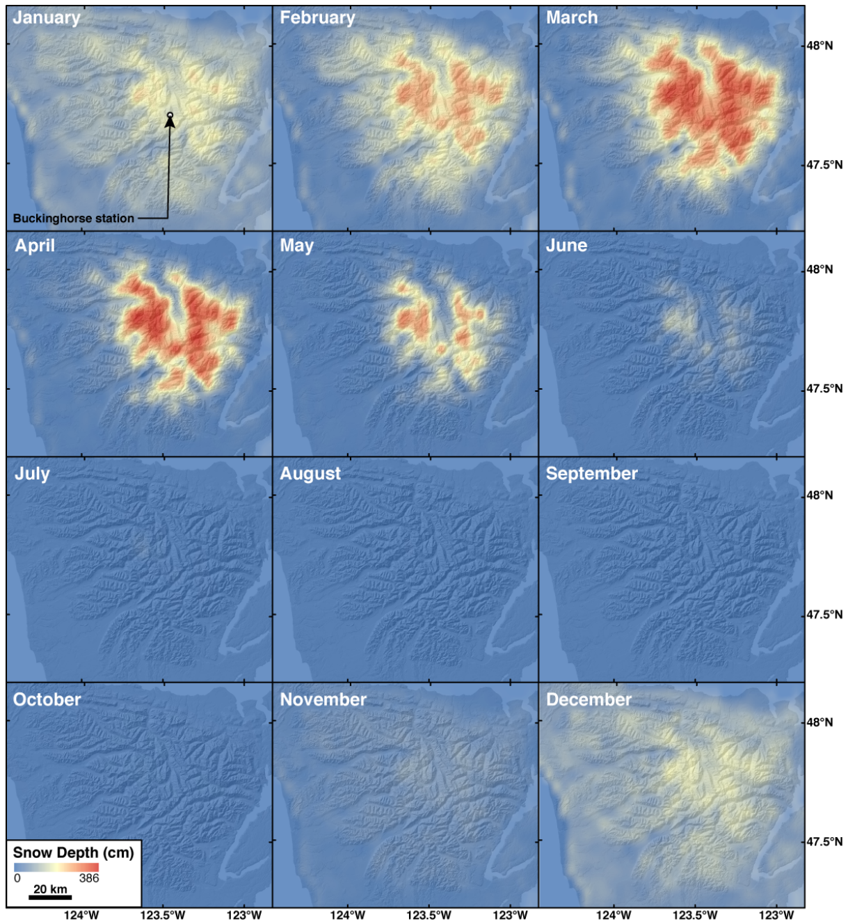
Figure S3. Monthly estimated snow depth map. The dot marks the position of the Buckinghamhorse SNOTEL meteorological
