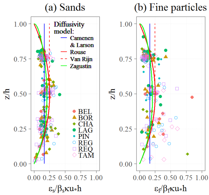
Figure 5: Dimensionless sediment diffusivity values-coefficient derived from the measured concentration profiles.
