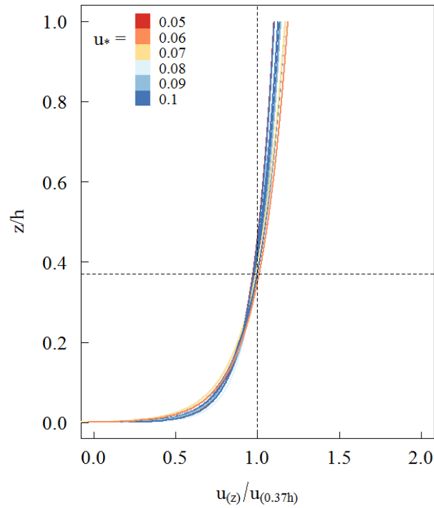
Figure RC2_5: Velocity profiles normalized by the velocity at 0.37 h , at REQ, Ucayali River, for various flow conditions.
