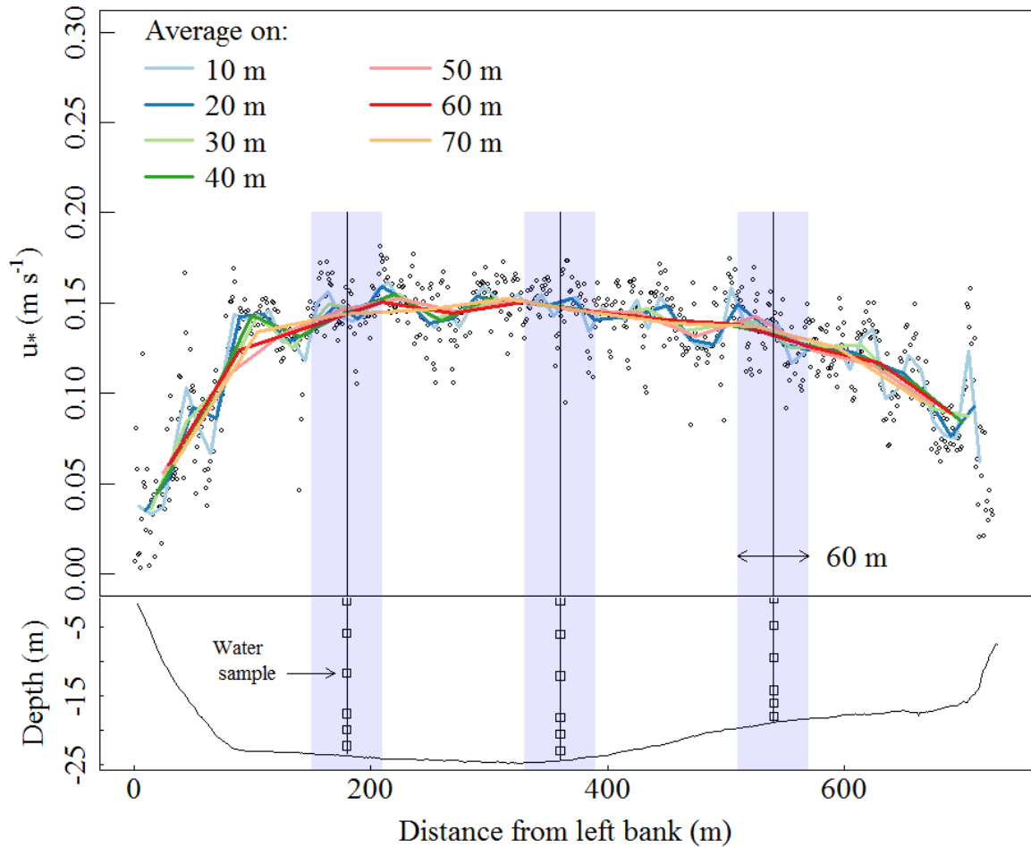
Figure RC2_6: ADCP data analysis at the San Regis station, on the Marañón River (transects measured in April 2012). Bottom screen: bathymetry of the cross-section, with the locus of the sampled concentrations (squares), the vertical sampled (continue lines in black) with the spanwise length of 60 m around each concentration profile position (purple rectangles). Top screen: the shear velocities fitted on each acquisition of a velocity profile (black dots) and their mobile averages over different units of length (color lines).
