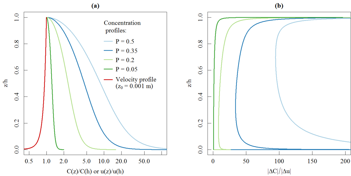
Figure RC2_2: (a) comparison between a typical velocity gradient (red line) and concentration gradient for various Rouse numbers. (b) ratio of concentration to velocity gradient with depth.
