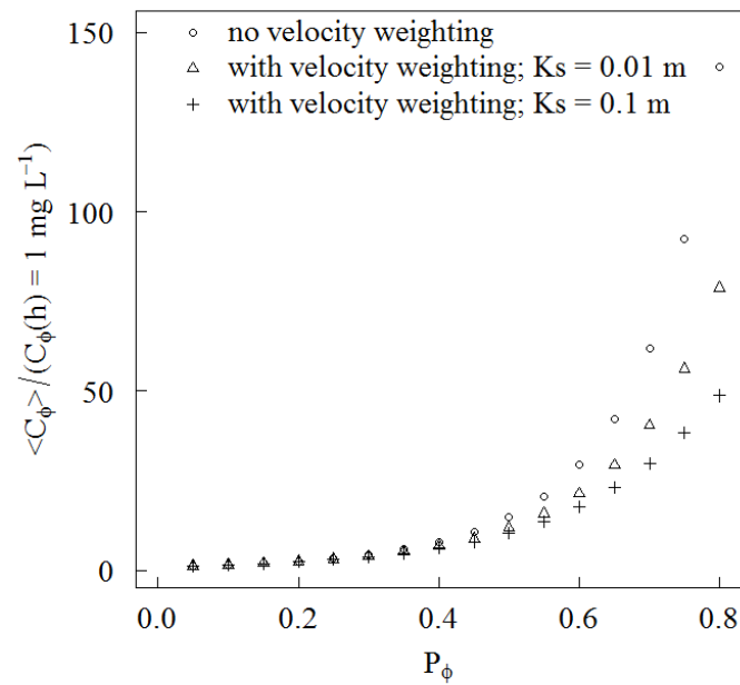
Figure RC2_3: Discrepancy between a mean concentration weighted by velocity distribution and a mean concentration calculated without velocity weighting. Two cases of velocity distributions were considered here: one for K_s = 0.01 \text{ m} (triangles) and another for K_s = 0.1 \text{ m} (crosses).
