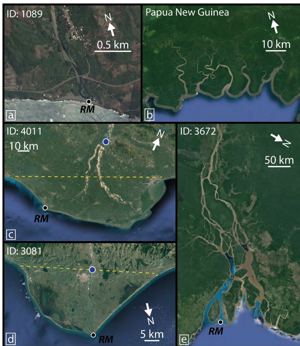
Figure 1. Examples of (a) a river mouth without a delta, (b) headless tidal channels not included in this dataset, (c) a delta with land both upstream and downstream of the regional shoreline vector (marked by dashed line), and location of delta node demarcated with blue dot, (d) a delta distinguished by a shoreline protrusion only, (e) a delta distinguished by a distributary channel network only. RM locations mark the main river channel mouth.
