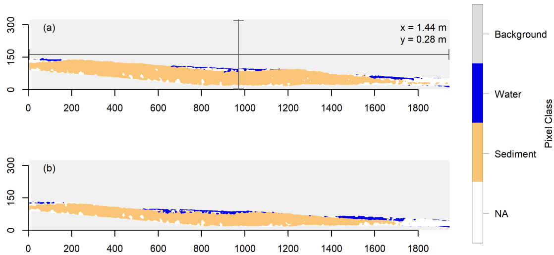
Figure 4. Output after image classification at the onset of output for Exp. 100L using (a) GSD_{broad} ( T = 326 min) and (b) GSD_{narrow} ( T = 149 min). Axes are pixel values of the raster, and real distances are provided for scale.
