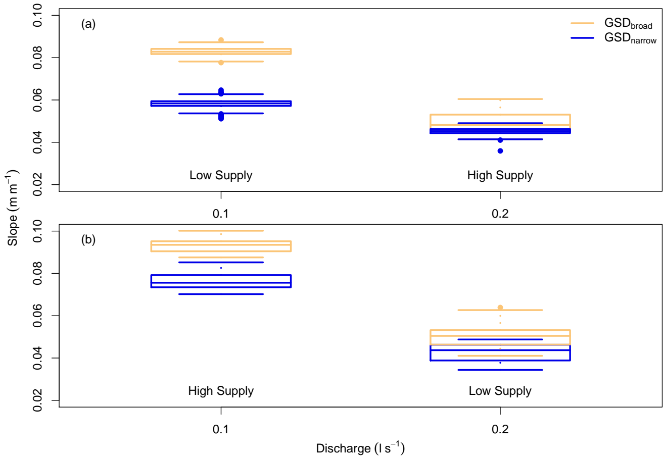
Figure 6. Distribution of slope values from the onset of transport onwards. Plots separate experiments by relative sediment concentrations of (a) 1 and (b) not 1 (i.e., 0.5 or 2). Text indicates sediment feed rate (low supply = 1 \text{ g s}^{-1} , high supply = 2 \text{ g s}^{-1} ).
