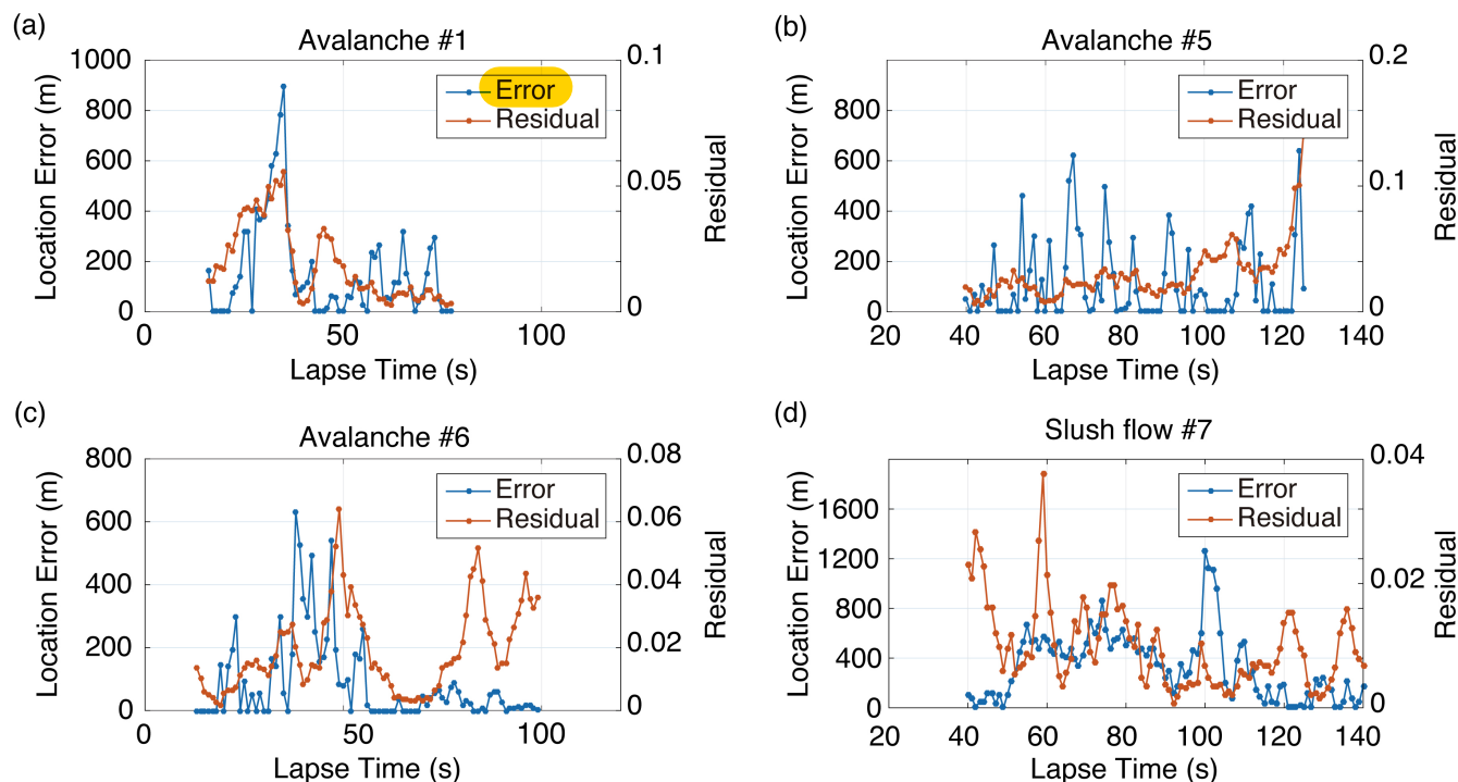
Figure 10. Location errors and residuals estimated as a function of lapse time from the simulation start time of avalanche #1 (a), avalanche #5 (b), avalanche #6 (c) and slush flow #7 (d).
