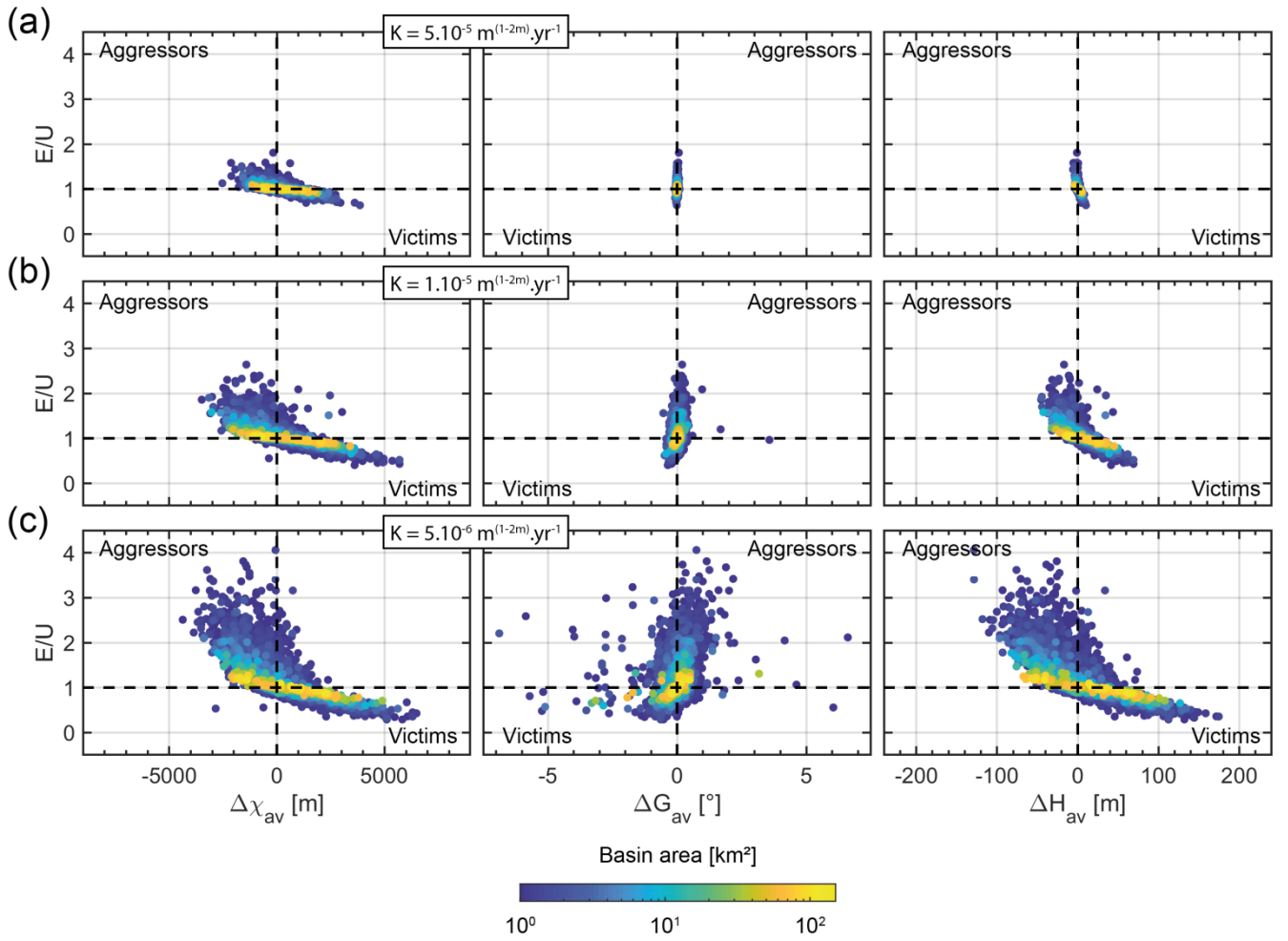
Figure 9: Effect of erodibility. Color scale indicates basin area. Basins of variable sizes, sorted in seven area classes expanding geometrically with a multiplying factor of 2 from 1-2 to 64-128 km 2 , every 0.5 Myr over the time period 5-10 Myr. Basins with a confidence index lower than 50 % are discarded from the analysis. (a) Results with an erodibility coefficient of 5.10^{-5} \text{ m}^{(1-2m)} \cdot \text{yr}^{-1} . (b) Results with an erodibility coefficient of 1.10^{-5} \text{ m}^{(1-2m)} \cdot \text{yr}^{-1} . (c) Results with an with an erodibility coefficient of 5.10^{-6} \text{ m}^{(1-2m)} \cdot \text{yr}^{-1} .
