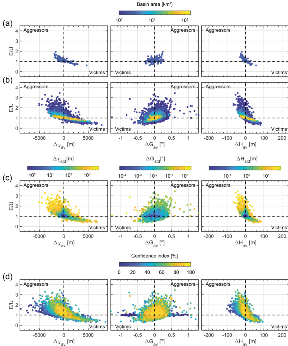
Figure 7: Denudation rates normalized by uplift rate as a function of aggressivity metrics and parameters influencing data dispersion. (a) Basins of 2-4 km² for the reference model after 2.5 Myr of simulation. Color scale indicates basin area. Basins with a confidence index lower than 50 % are discarded from the analysis. (b) Basins of variable sizes, sorted in seven area classes expanding geometrically with a multiplying factor of 2 from 1-2 to 64-128 km², every 0.5 Myr over the time period 2-10 Myr. Color scale indicates basin area. Basins with a confidence index lower than 50 % are discarded from the analysis. (c) Basin of 1-2 km² over the time period 2-10 Myr, color scale indicating the standard deviation of \Delta\chi , \Delta G and \Delta H , respectively. Basins with a confidence index lower than 50 % are discarded from the analysis. (d) Basin of 1-2 km² over the time period 2-10 Myr. Color scale indicates confidence index.
