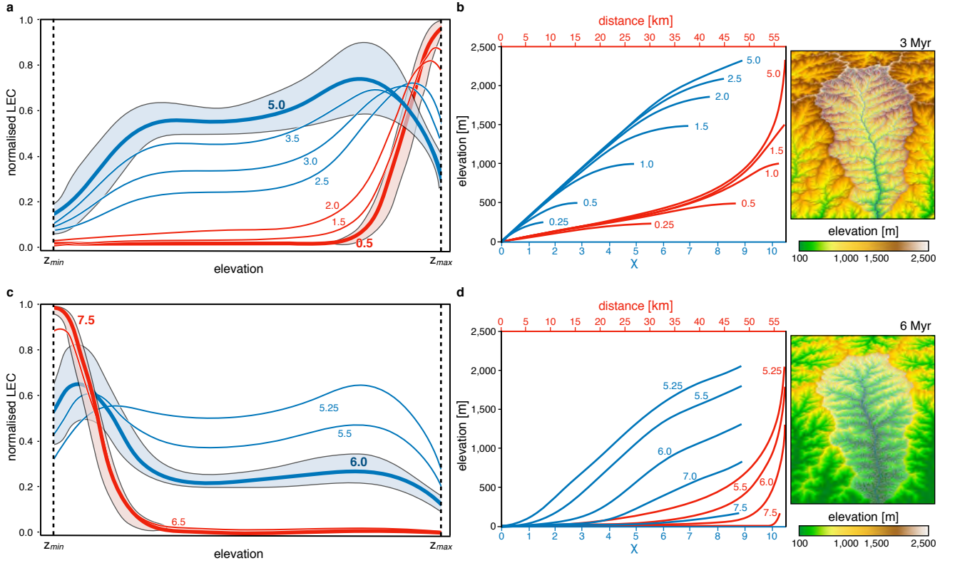
Figure 3. Analysis of uniform precipitation results. a) & b) relate to the mountain building phase (0–5 Myr) and c) & d) to the relaxation phase (5–10 Myr). Plots in a) & c) illustrate the elevational gradients of normalised LEC over time (corresponding numbers in Myr for each lines). Blue/Red lines represent average of normalised LEC within elevational bands. Blue/Red areas are the standard deviation computed based on normalised LEC values as a function of site elevation at 5 & 6 Myr (blue areas) and 0.5 & 7.5 Myr (red areas). For each plots a) & c) , line colours reflect different stages of landscape evolution. In a) change from red to blue marks the disappearance of uplifted plateau. In c) change from blue to red relates to the erosion of 50% of the maximum elevation obtained at steady state. These 2 plots have a moving horizontal scale as z_{min} and z_{max} change with time. b) & d) show main stream temporal evolution for catchment area (region A) defined in Fig. 2a and displayed at 3 and 6 Myr respectively (right panels). For the considered catchment, we show the extracted information from main channel profiles based on \chi -plot analysis (Perron and Royden, 2013) (blue) and longitudinal river profiles (red) over time (associated time in Myr is given for each lines).
