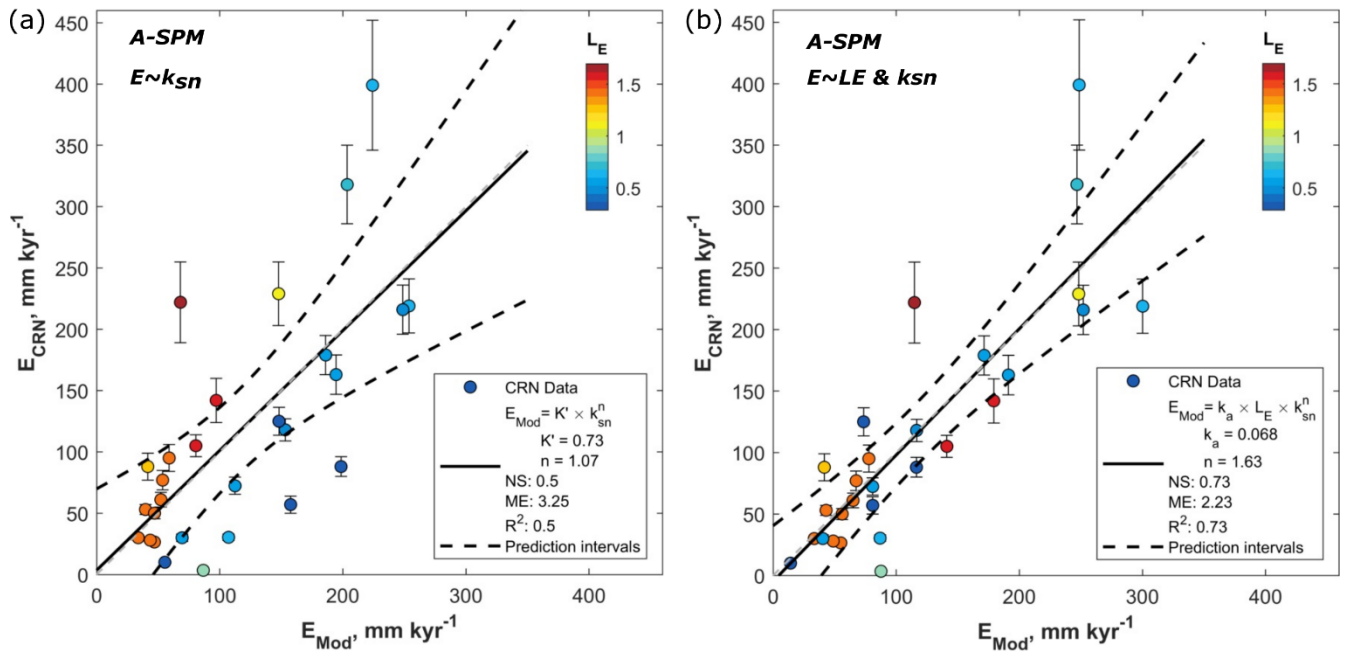
1015 Figure 7 Best fit between CRN-derived erosion rates ( E_{CRN} ) and modelled river incision ( E_{Mod} ) using the area- based Stream Power Model (A-SPM). (a) A-SPM, scenario 1 (cf. Table 4) assuming a uniform lithology. Observations are coloured according to the average lithological erodibility of the catchment ( \bar{L}_E ). Low values for \bar{L}_E represent strong rocks, resistant to erosion. High values for \bar{L}_E represent weak rocks, susceptible to erosion. Modelled erosion rates for catchments consisting of strong rocks (blue colours) are mostly over predicted and plot below the 1:1 line. Modelled erosion rates for catchments consisting of weak rocks (red colours) are mostly under predicted and plot above the 1:1 line. (b) A-SPM, scenario 1020 2 (Table 4) where spatially variable lithological erodibility is explicitly accounted for in the A-SPM. Catchment specific values for \bar{L}_E are listed in Table 2, while the model parameters are listed in Table 4. A complete overview of all best model fits for A-SPM scenarios 1 - 4 is given in Figure S8.
