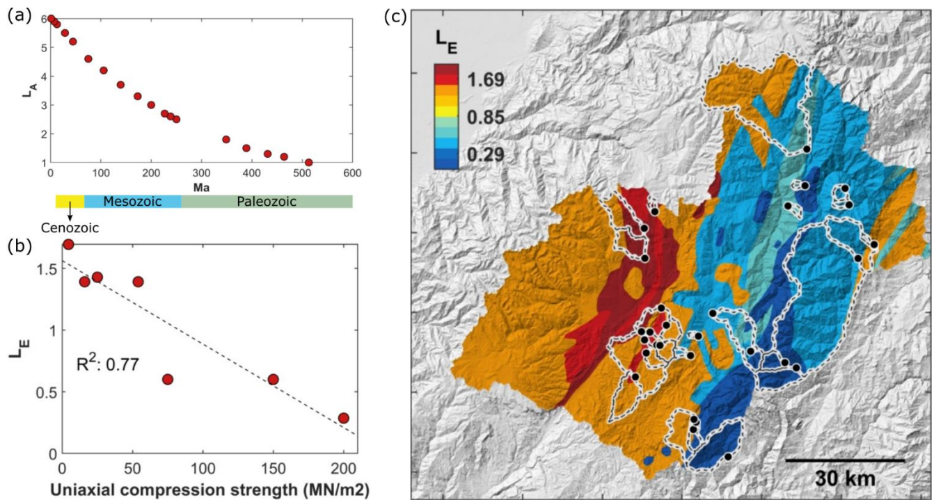
980 Figure 2: Development of empirical lithological erodibility index ( L_E ) and its application to the Paute catchment. (a) Proposed lithological erodibility index based on lithological age ( L_A ). Detailed sub-classifications per lithology can be found in Table S1. (b) Field measurements of uniaxial compressive strength (Basabe R, 1998; Table S4) versus the empirical erodibility index calculated using Eq. 7. Note that two of the nine observations overlap on this plot. (c) Spatial distribution of L_E in the Paute catchment. The underlying topographic map is based on the 30 m SRTM v3 DEM (NASA JPL, 2013). The 985 lithological erodibility map for Ecuador was used to delineate different lithostratigraphic units and is based on the 1M geological map of Ecuador (Egüez et al., 2017 see also Figure S1 ). The map is produced with TopoToolbox (Schwanghart and Scherler, 2014).
