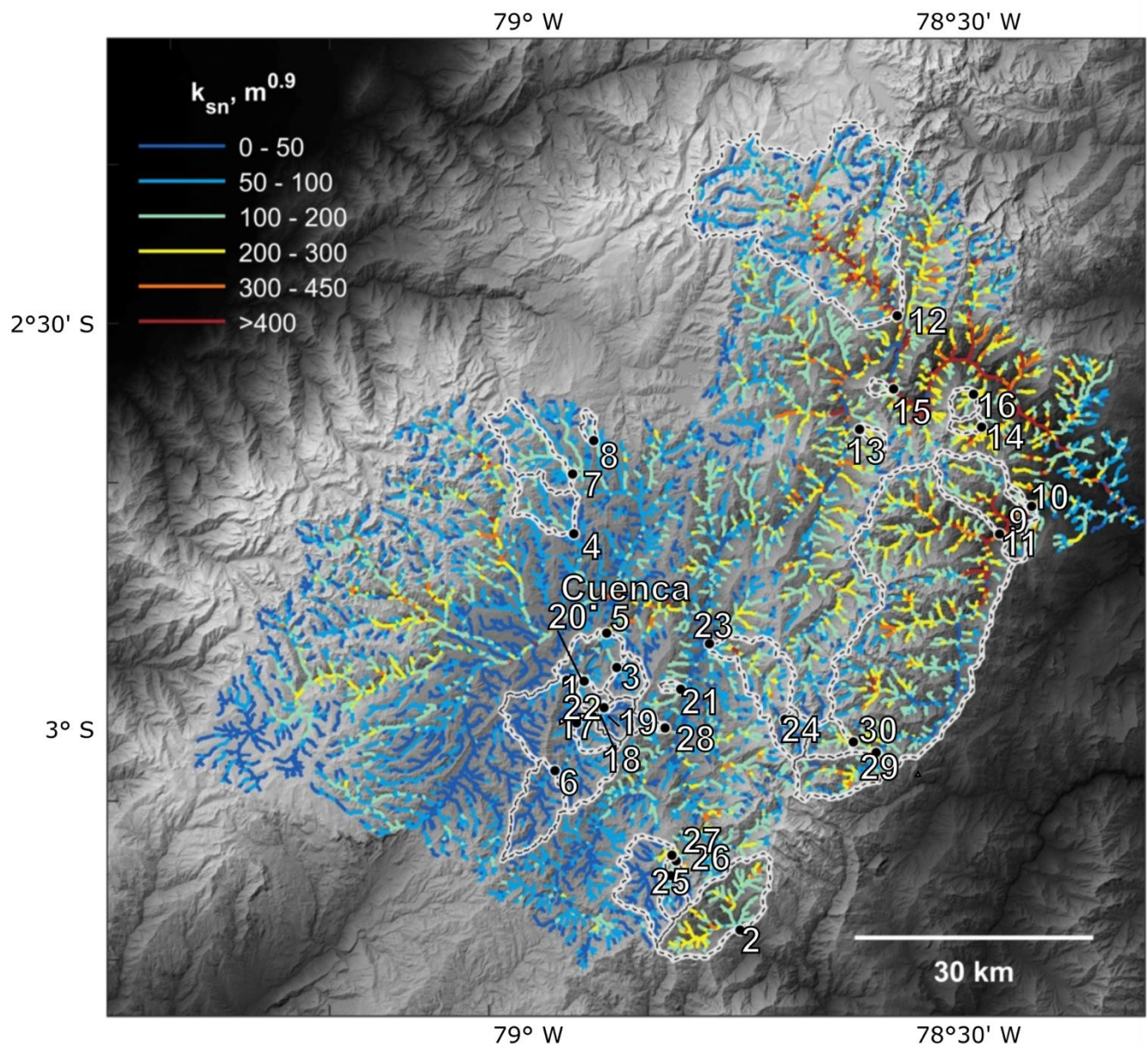
990 Figure 3: Normalized steepness ( k_{sn} ) for the Paute basin. Calculated k_{sn} -values for the Paute basin are overlain with a hillshade map (based on the 30 m SRTM v3 DEM; NASA JPL, 2013). The highest values can be observed in two major knick zones, located in the lower part of the Paute basin. In these zones, topographic rejuvenation started and a transient incision pulse has propagated from East to West (see also Figure S3). The map is produced with TopoToolbox (Schwanghart and Scherler, 2014).
