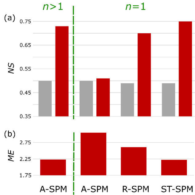
Figure 9: Comparison of model performance of four selected river incision models. (a) Nash Sutcliffe model efficiency ( NS ) for different model scenarios, without (grey bars) or with (red bars) considering lithological heterogeneity. (b) shows the corresponding Model Error ( ME ). The A-SPM model scenario corresponds to the Area-Based Stream Power Model (cf. Figure 7). It performs well when lithological heterogeneity is considered and all parameters are freely calibrated, resulting in a slope-steepness exponent ( n ; cf. Eq. 1) of 1.62 (for a full overview of model parameters, see Table 4). However, for an A-SPM scenario where n is fixed to the theoretically derived value of 1, the model performance strongly deteriorates (see main text). R-SPM represents a model scenario that explicitly incorporates runoff variability (cf. Figure 8a). The ST-SPM scenario also includes an incision threshold (cf. Figure 8b). Both scenarios perform well when n is fixed to 1 and when considering lithological heterogeneity. Overall, the best model performance (highest NS and smallest ME ) is obtained under the ST-SPM scenario where lithological and runoff variability, as well as river incision thresholds are considered.
