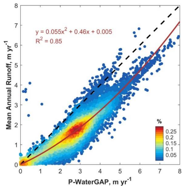
1005 Figure 5: Calibration of the precipitation ( P ) versus runoff curve ( R ). Mean annual runoff versus the mean annual precipitation for all WaterGAP3 pixels in Ecuador ( 0.25^\circ ; 1979-2014; WaterGAP3 data available from earth2observe.eu).
