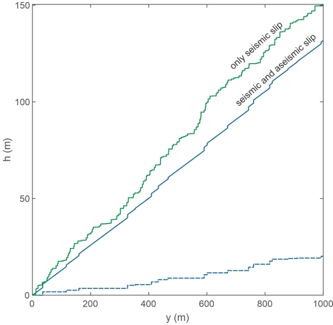
Figure 6. Modeled river profiles considering the “only seismic slip” (green line) and the “seismic and aseismic slip” (blue line) models. For this latter, the contribution of seismic slip is showed (dashed blue line).
