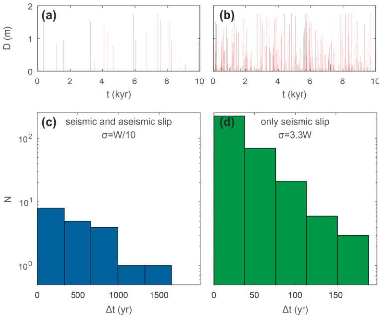
Figure 5. Time distribution of earthquakes rupturing the river. a-b) Co-seismic displacements D at the location of the river as a function of time t for each model. c-d) Distribution of inter-event time \Delta t of earthquakes rupturing the surface at the location of the river.
