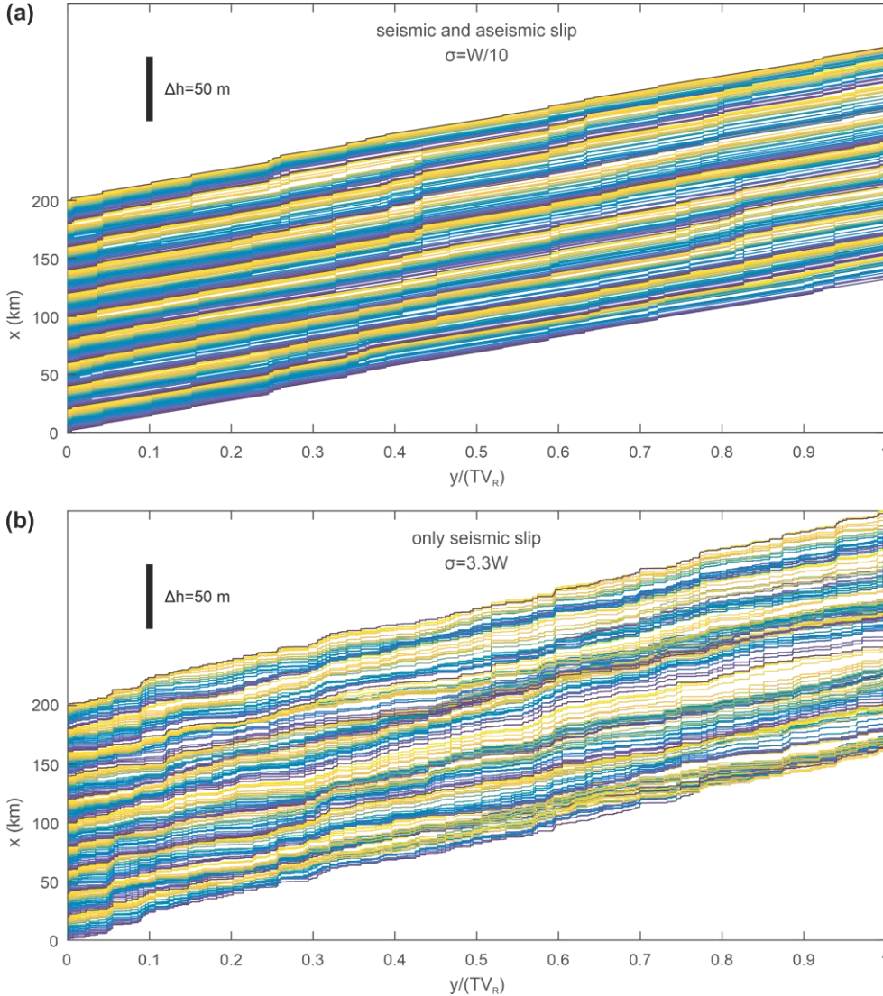
Figure 10. Topography of a set of parallel rivers flowing across-strike the fault. a-b) River profiles of 200 rivers separated by 1 km along the strike of the fault, i.e. the x-direction. River elevation h is given along the same axis, with a scaling factor of 1000. River length y across
