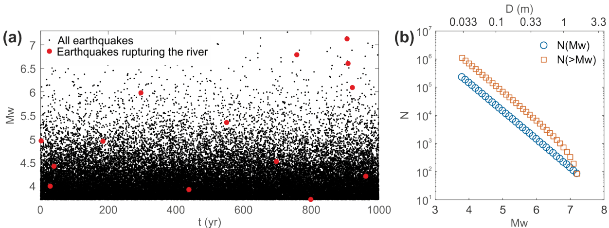
Figure 2. Modeled seismicity and its statistical characteristics. a) Time distribution t of the magnitude Mw of earthquakes during the first 1000 years of one model. Both mainshocks and aftershocks are shown with black dots. Earthquakes with rupture zone extending to the surface and cutting the river, located at the middle of the fault trace, are shown with red dots. b) The cumulative (light red squares) and incremental (light blue circles) Gutenberg-Richter magnitude-frequency distribution of earthquakes for one model. N is the number of events and D is the associated displacement computed using Leonard (2010) scaling law.
