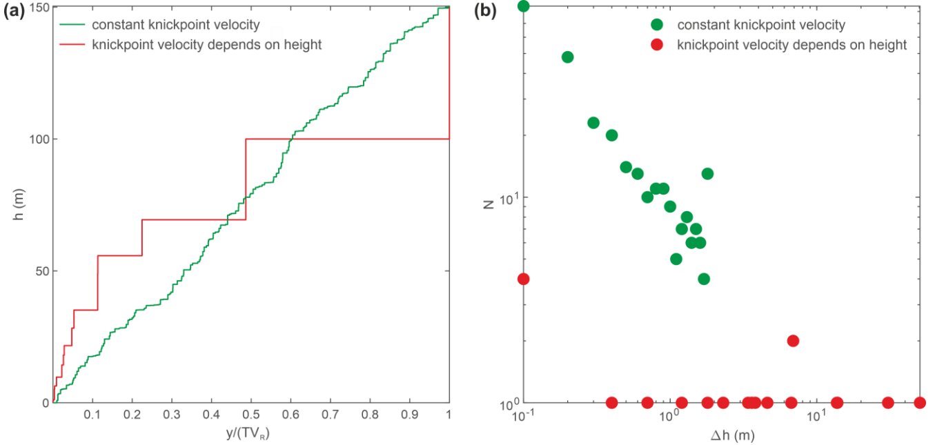
Figure 7. Modeled a) river profiles and b) knickpoint height distribution considering a constant knickpoint velocity (green line and circles) or a velocity depending on knickpoint height (red line and circles) .
