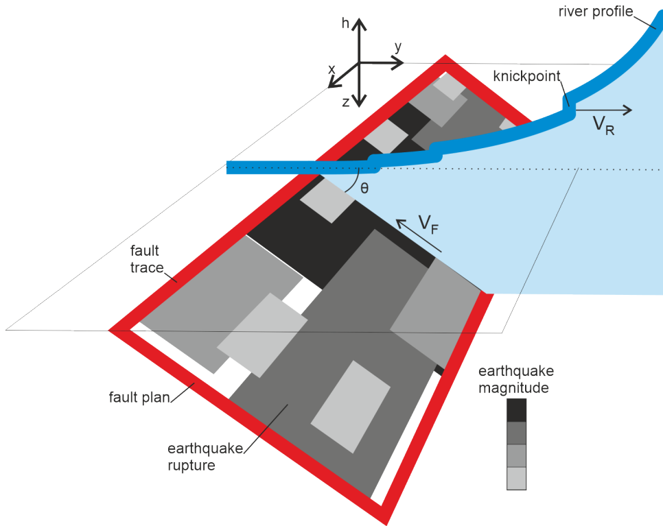
Figure 1. Schematic sketch showing the model setup. The fault plan, dipping with an angle \theta , is represented by a red contour and includes the earthquakes and their ruptures represented by gray box, which color indicates the magnitude. The fault trace is aligned along the x -axis and earthquakes occur at depth z . The river profile is indicated by a blue line along the y -axis and has an elevation h . The river contains several knickpoints. Note that in this paper we only focus on knickpoints occurring in near-fault condition. The rate of fault slip is V_F while knickpoint migrate at a constant velocity V_R .
