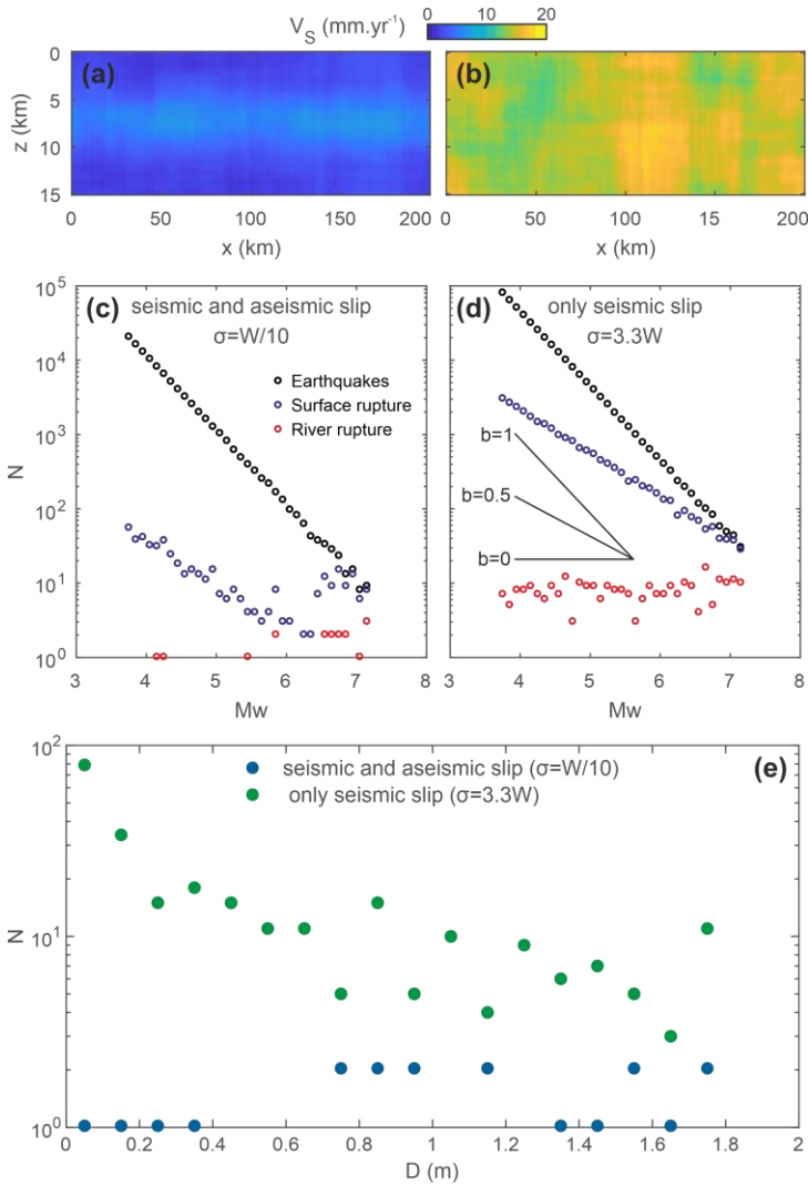
Figure 4. Incremental distribution of earthquake magnitude and displacement in surface and at depth. Maps of averaged fault seismic slip rate V_S on the fault plane for a) the “seismic and aseismic slip” and b) the “only seismic slip” models. The scale of the z -axis is increased compared to the x -axis to enhance readability. c-d) Modeled magnitude distributions of earthquakes on the fault (black circles), earthquakes rupturing the surface (blue circles) and of earthquakes rupturing the river (red circles) for the same models than in panels a and b, respectively. N is here is the incremental number of earthquakes, i.e. N(m) . e) Distributions of displacement for earthquake rupturing the river for the considered models, with green and blue circles representing the “only seismic slip” and the “seismic and aseismic slip” models, respectively.
