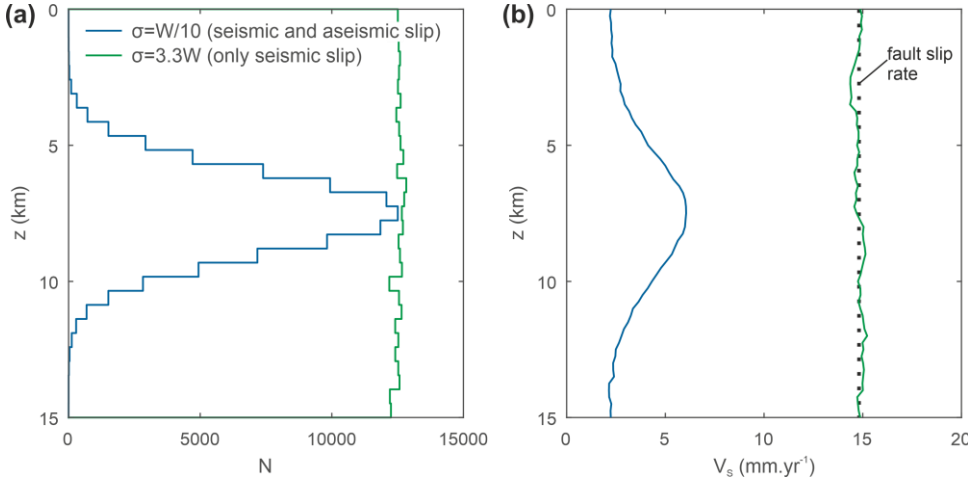
Figure 3. Depth distribution of earthquakes, seismic and aseismic slip. a) Depth-distribution of the number N of mainshocks for the 2 models considered here. The depth distribution is a normal one centered at 7.5 km of depth and with a variance \sigma equals to W/10 (blue) or 3.3W (green). b) Depth-distribution of seismic V_s slip. The vertical black line indicates the averaged fault slip rate of \sim 15 mm.yr -1 , summing seismic and aseismic slip. Aseismic slip rate is simply the difference between the average fault slip rate and seismic slip rate, so that all models share the same total slip rate.
