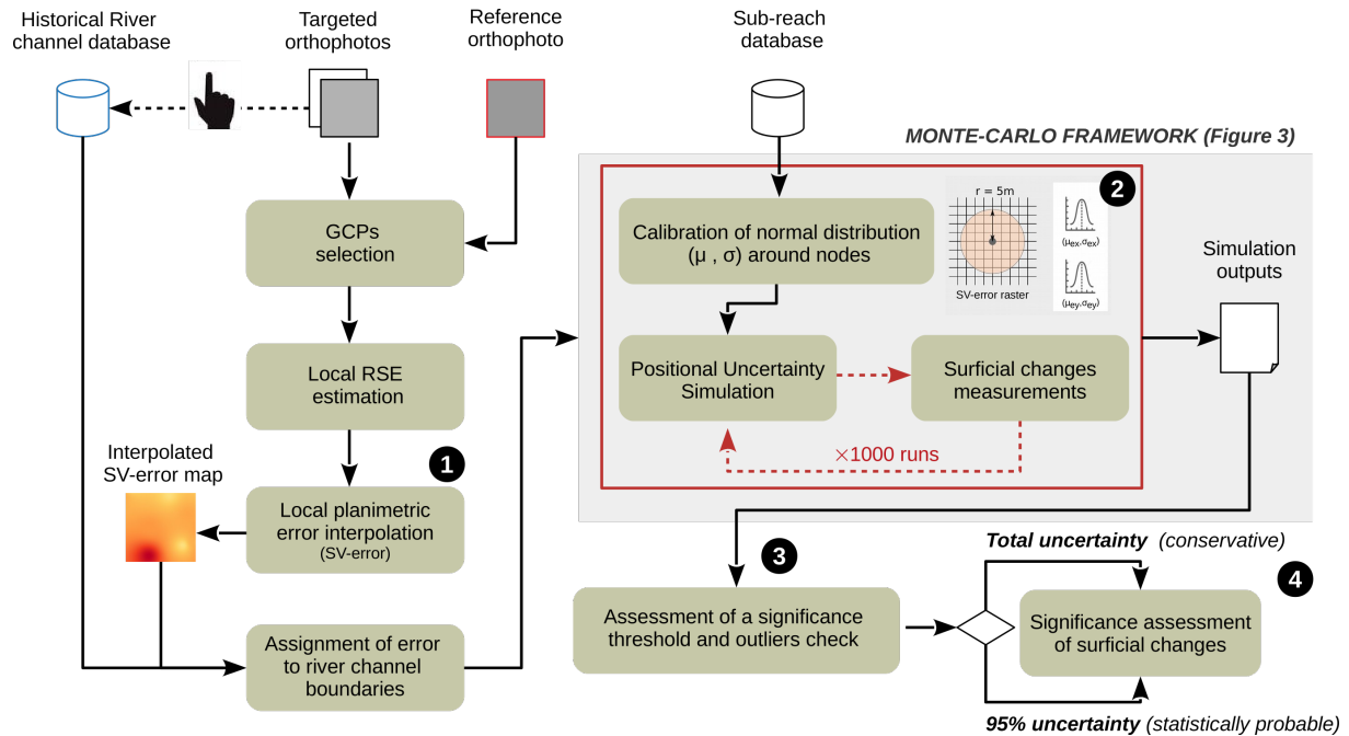
Figure 9. Detailed flow chart of the methodology applied in this study, allowing to assess uncertainty of eroded and/or deposited surfaces using SV-error SV error .
