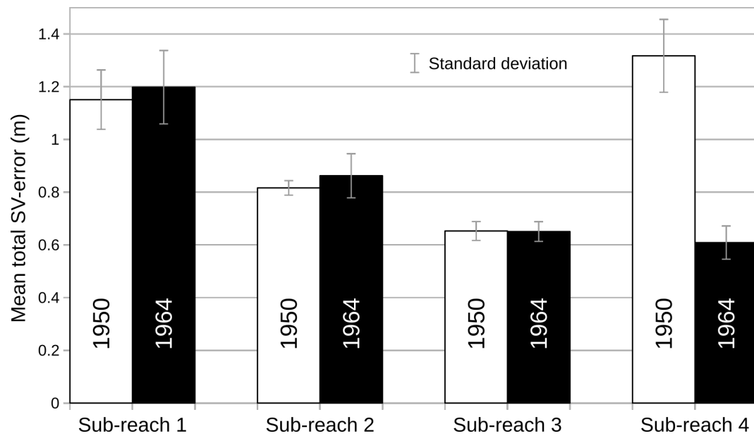
Figure 5. Mean total SV-error SV error for each sub-reach, on both dates.
