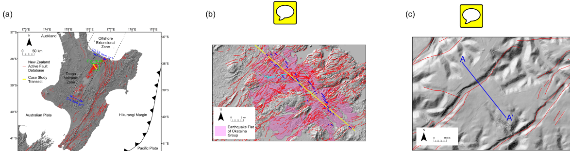
Figure 4. Taupo Volcanic Zone Case Study. Base images of A, B, and C are LiDAR hillshade maps of the North Island and Taupo Volcanic Zone, New Zealand. A) Tectonic features of New Zealand where the green box represents the enlarged image in B. The red fault traces are from the New Zealand Active Faults Database (NZAFD). Active faults have deformed the ground surface of New Zealand within the last 125,000 years. The blue arrow and rate represents geologic extension rates from geodetic and Quaternary fault data (P. Villamor et al., 2017). The yellow line represents the Case Study Transect. B) Fault scarp profiles used in this case study are shown in blue and across the northwest-southeast transect shown in yellow. Mapped faults in the region are shown in red (NZAFD). For simplicity, only the Earthquake Flat Formation of the Okataina Group outcrops is shown from the Geologic Map of New Zealand Project (GMAP). These are the formations that were analyzed in this study. The light blue box represents the extent of part C. C) LiDAR hillshade map to demonstrate the resolution of the DEM and location of profile shown in Figure 2. sualized in Figure 2 and with location shown in Figure 4.
