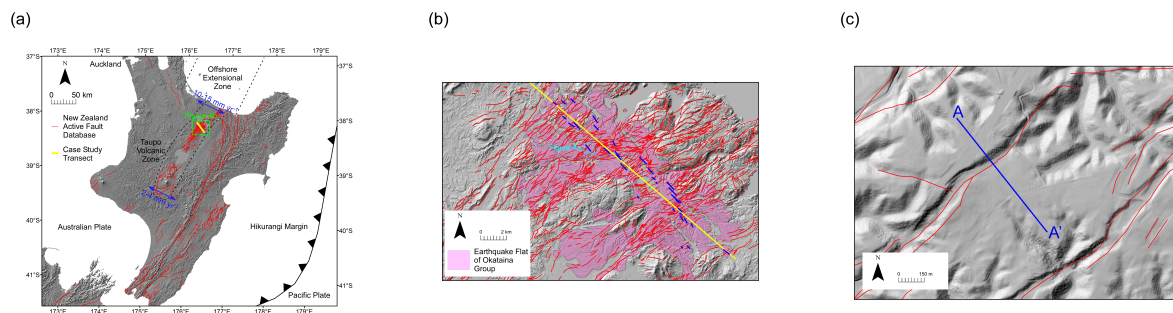
Figure 4. Taupo Volcanic Zone Case Study. Base images of (a), (b), and (c) are LiDAR hillshade maps of the North Island and Taupo Volcanic Zone, New Zealand. a) Tectonic features of New Zealand where the green box represents the enlarged image in (b). The red fault traces are from the New Zealand Active Faults Database (NZAFD). Active faults have deformed the ground surface of New Zealand within the last 125,000 years. The blue arrow and rate represents geologic extension rates from geodetic and Quaternary fault data (P. Villamor et al., 2017). The yellow line represents the Case Study Transect. b) Fault scarp profiles used in this case study are shown in blue and across the northwest-southeast transect shown in yellow. Mapped faults in the region are shown in red (NZAFD). For simplicity, only the Earthquake Flat Formation of the Okataina Group outcrops is shown from the Geologic Map of New Zealand Project (GMAP). These are the formations that were analyzed in this study. The light blue box represents the extent of part (c). c) LiDAR hillshade map to demonstrate the resolution of the DEM and location of profile shown in Figure 2 and with location shown in Figure 4.
