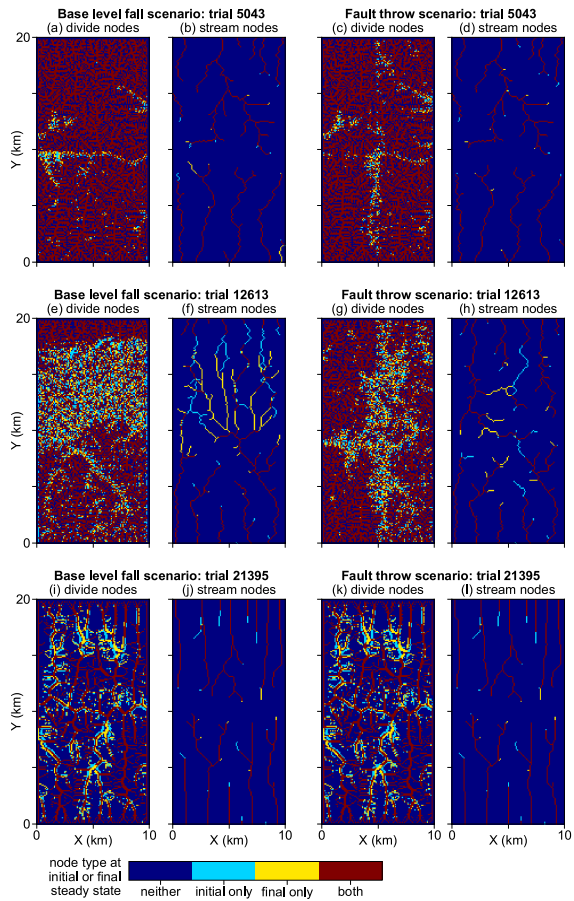
5 Figure 8. Landform change of exemplary trials. This figure illustrates landform change model responses of the trials discussed in Sect. 4 and labelled in Fig. 7. The colour of grid cells symbolises landform type at the initial and final steady state in the model. Blue areas were not the landform type (divide or stream) in a given subplot at the times of either steady state. Red areas were the subplot landform type in both steady state times. Cyan and yellow areas were the subplot landform type in the initial and final steady state, respectively. The parameter values of these trials and all other trials are provided in Lyons et al. (2019).
