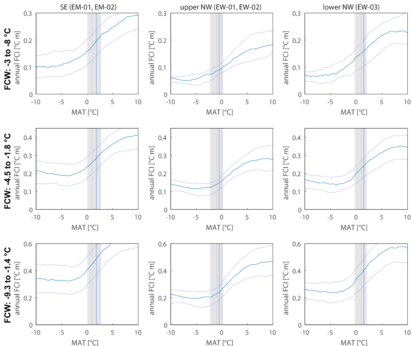
850 Figure B1: \overline{FCI} sensitivity to different frost cracking windows (FCW) for the frost cracking model, with standard model inputs from Andersen et al. (2015) in the upper row, and two windows from Draebing et al. (2017b) in the middle and lower row, respectively. These are dependent on the mechanical bedrock properties and were originally calculated for anisotropic slaty paragneisses. Shaded area corresponds to reconstructed historical temperature range; vertical bars indicate modern mean, min. and max. MAT conditions and curves represent the corresponding dT_a and dT_d conditions. Note the different y-axis scale for the \overline{FCI} of each row.
