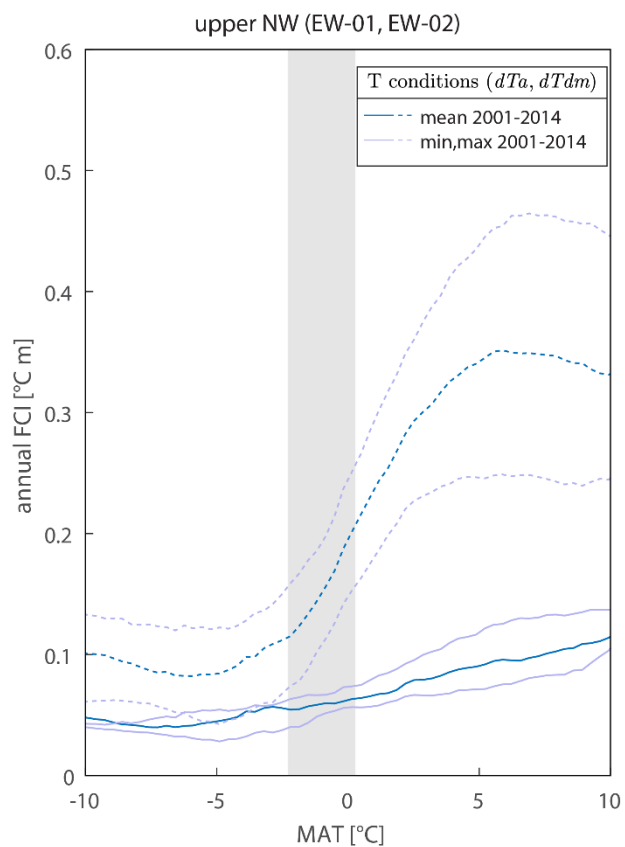
Figure B2: \overline{FCI} sensitivity to thermal conductivity of bedrock ( k_r ). Modelled results for \overline{FCI} results with k_r = 1.2 \text{ W m}^{-1} \text{ K}^{-1} (dashed lines) and k_r = 6.5 \text{ W m}^{-1} \text{ K}^{-1} (solid lines), representing upper and lower thresholds for thermal conductivities compiled for various lithologies (Schön, 2015). Model set up to standard conditions of Andersen et al. (2015) for all other input variables. The shaded area corresponds to the reconstructed historic temperature range.
