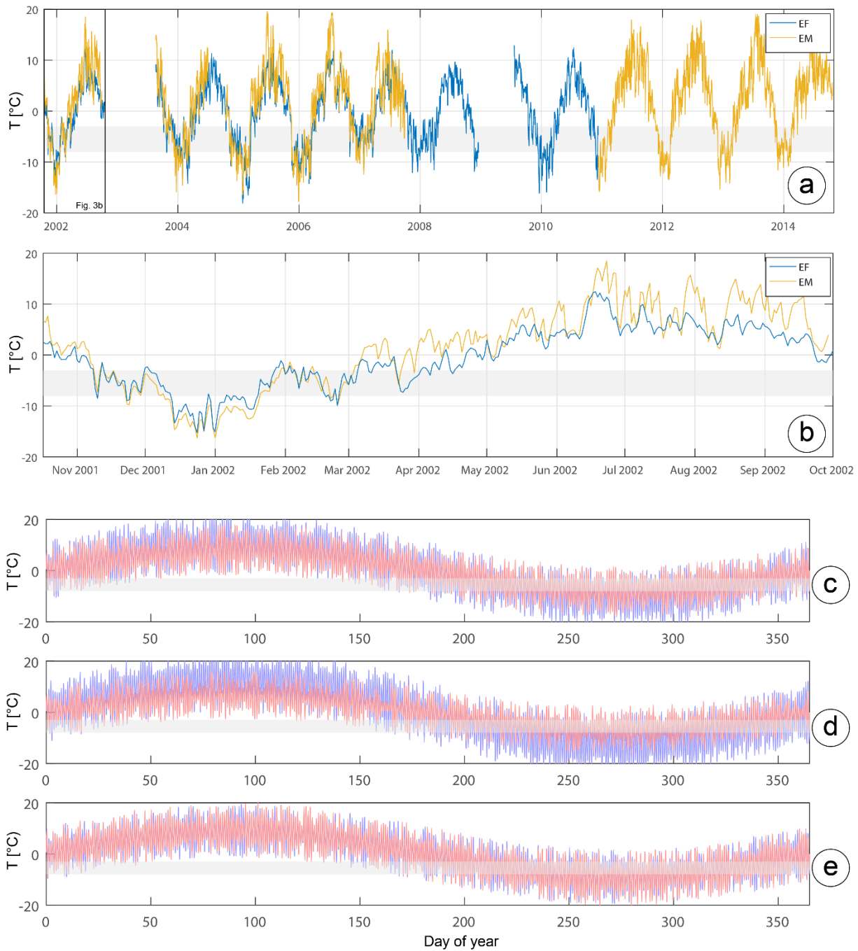
Figure 3: (a) Complete daily averaged PERMOS (2019) temperature data for the upper NW (EF) and the SE sites (EM). (b) Daily averaged hydrological year 2002, which Data displayed in panels a and b were used in this study to estimate dT_a and dT_d . For modern min, mean and max estimations only complete years were used. Synthetic temperature curves which were used for the frost cracking model for the upper NW (blue) and SE (red) sites for modern mean (c), modern minimum (d) and modern maximum conditions (e). Shaded area corresponds to the frost cracking window of -3 to -8 °C. See text for discussion.
