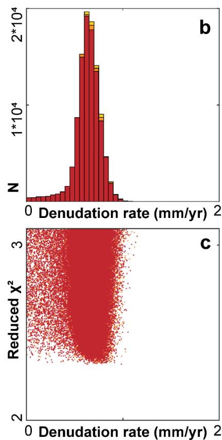
Figure A1: Analysis of cosmogenic ^{10}\text{Be} at site EW-01. (a) Measured ^{10}\text{Be} concentrations plotted against the Monte Carlo (MC) solution space (light colors) and the best-fit profiles. (b) Denudation rate histogram from the MC modelling for 10^5 model profiles and (c) corresponding reduced chi-square ( \chi^2 ) values. Different model setup results are superimposed (for discussion see text).
