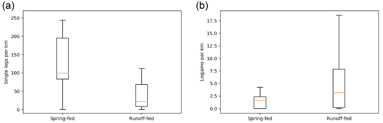
Figure 4. Boxplot representing the number of (a) single logs and (b) logjams identified per km via satellite imagery on spring-fed and runoff-fed streams.
