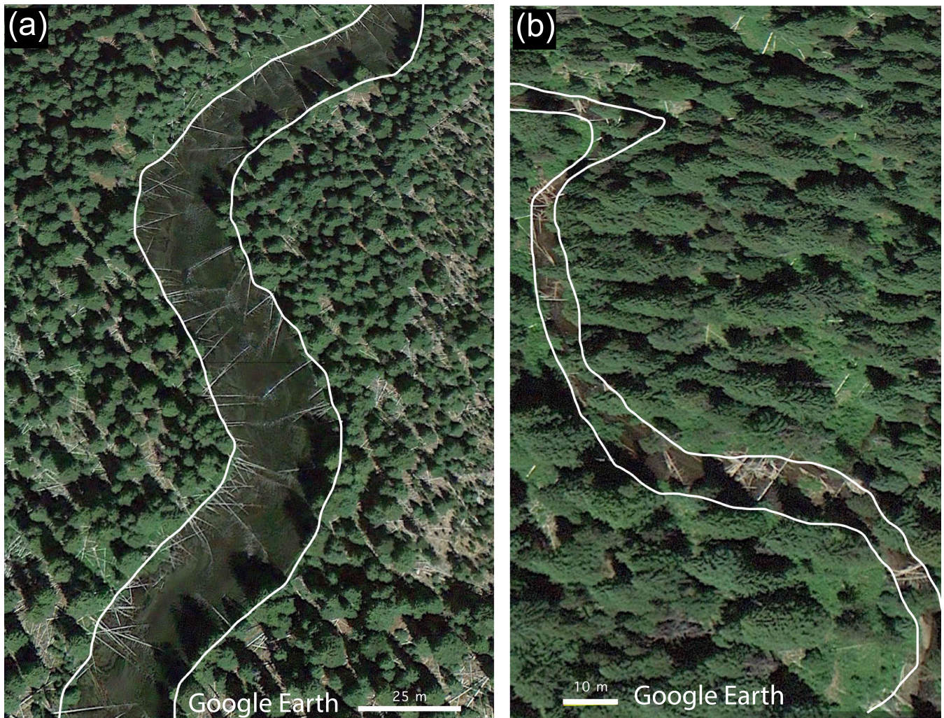
Figure 3. Google Earth Pro high-resolution imagery showing (a) Cultus River ( q_{95} = 2.8 \text{ m}^3/\text{s} ) and (b) Cultus Creek ( q_{95} = 2.3 \text{ m}^3/\text{s} ). Stream channels are outlined in white, and flow direction is down from the top of the image in both panels. These images are representative of the general wood dynamics in the two streams, where most of the wood in (a) is single logs, and most of the wood in (b) is in logjams, so little of the wood in panel (b) would contribute to the histogram shown in Figure 2 (b).
