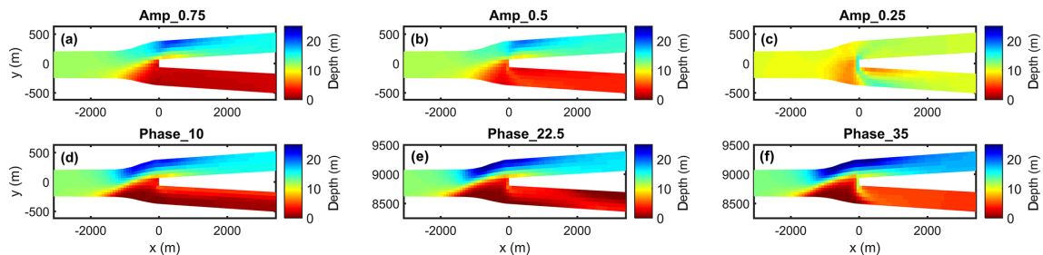
Figure A2. TS6 Final depth for Case 2. For the amplitude difference scenario (a–c), the downstream branch imposed by low tides is the bottom branch, while for the phase difference scenario (d–f) the bottom branch is the downstream branch imposed by delayed tides.
