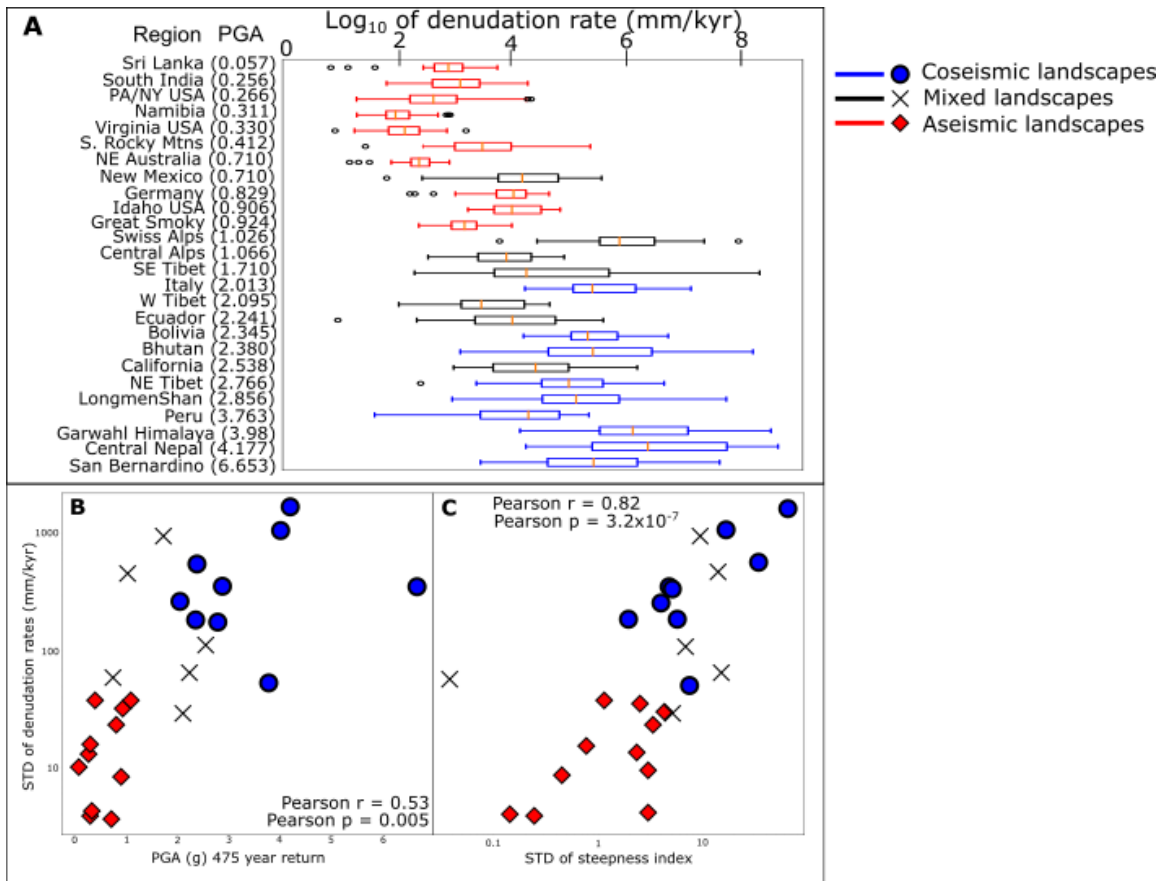
650 Figure 6. Reanalysis of detrital cosmogenic radionuclide derived denudation rates for mountain belts around the world compiled by Harel et al (2016), in the context of peak ground acceleration and tectonic environment. (A) A box plot indicating the median (central orange line), quartiles (end of box) and the range ('the whiskers') of denudation rates in the analysed localities ordered by their average seismicity (in brackets), defined as the maximum Peak Ground Acceleration of a 475-year return period (PGA). Points indicate values outside the range, \pm 1.5IQR . (B) Standard deviation (STD) of denudation rates for each mountain belt against seismicity represented by the 475-year return Peak Ground Acceleration ( ms^{-2} ). (C) Standard deviation of denudation rates for each mountain belt compared to the standard deviation of steepness indexes. The areas of highest variability are found in steep, tectonically active mountain ranges.
