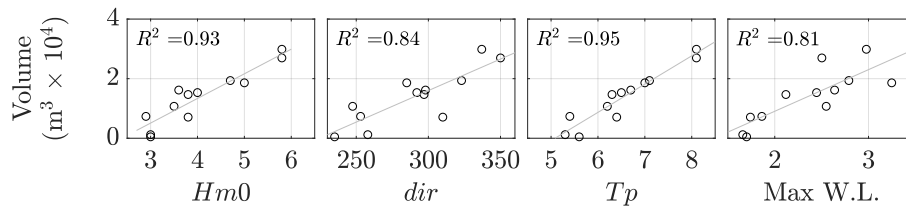
Figure 9. Scatter plot for the initial boundary conditions used for each scenario ( Hm0 , Tp , dir and maximum water level) against total volume deposited onto the sand flat.
