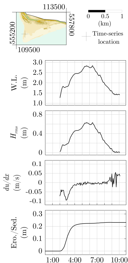
Figure 13. Time series of hydrodynamic and morphological characteristics extracted from scenario k.
