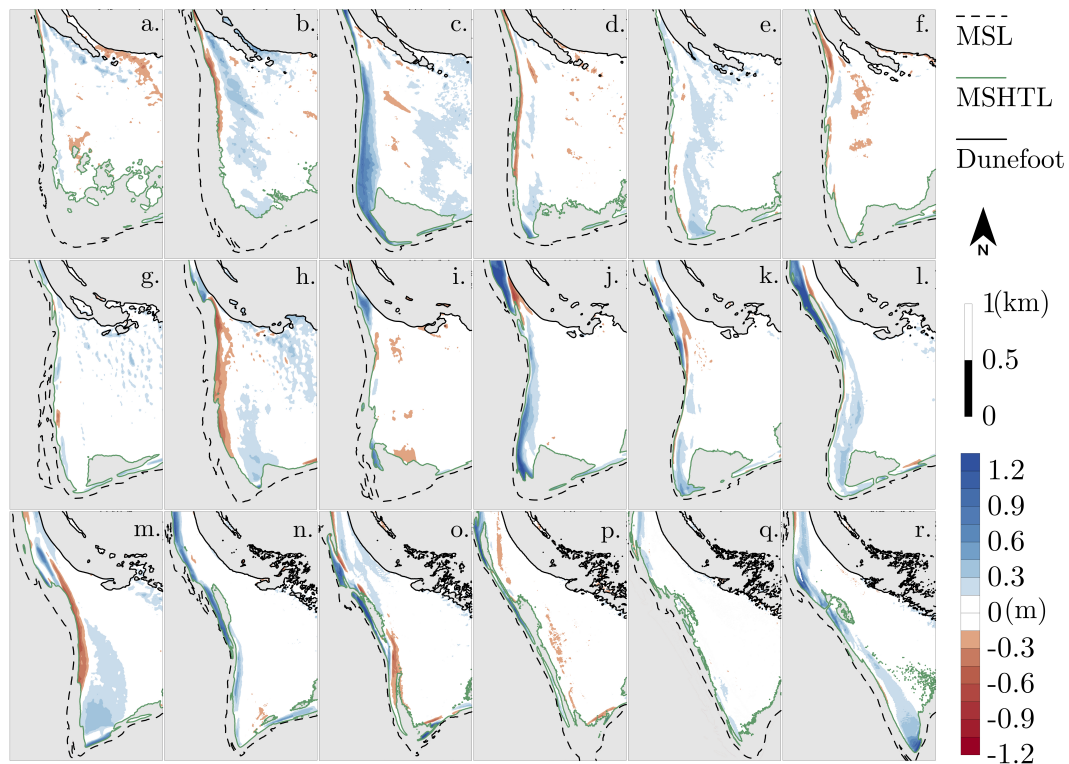
Figure 5. Difference maps for the periods between 1997 and 2017 focusing on the supra-tidal area. Letters refer to the specific years from which the subplots were calculated: 1998-1997 (a.), 1999-1998 (b.), 2001-1999 (c.), 2003-2001 (d.), 2004-2003 (e.), 2005-2004 (f.), 2006-2005 (g.), 2007-2006 (h.), 2008-2007 (i.), 2009-2008 (j.), 2010-2009 (k.), 2011-2010 (l.), 2012-2011 (m.), 2013-2012 (n.), 2014-2013 (o.), 2015-2014 (p.), 2016-2015 (q.) and 2017-2016 (r.). Most plots show a one-year difference, with exception of plots c. and d. which represent the difference between 1999-2001 and 2001-2003, respectively, due to the absence of surveys in the years 2000 and 2002.
