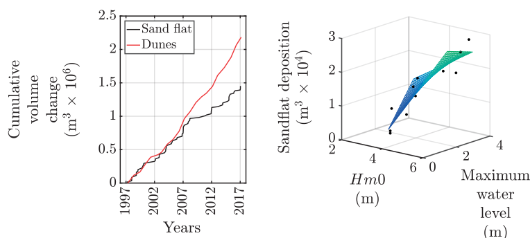
Figure 15. Left: Cumulative volume changes from the dunes using LiDAR data (Dunes) and estimated sand flat deposition using regression model as predictor (Sand). The regression model has been built using simulation results with maximum water level at the boundary and wave height as predictors for deposition. Right: Scatter plot of the regression model used with regression surface.
