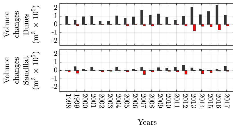
Figure 7. Annual volume changes for the sand flat and dune area considering only cells where elevation change was greater than 0.16 meters (approximately the maximum possible error based on the allowed error for each LiDAR survey.)
