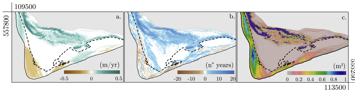
Figure 6. a - Average annual elevation change based on LiDAR data from 1997 up to 2017. Dashed lines show the average position of the MSHTL. b - Net number of years where accretion/erosion occurrences from the difference maps were greater than 0.16 meters. Negative values mean that the location had more erosive years than accretive, whereas positive values mean that the location had more accretive years than erosive. c - Variance of the elevation.
