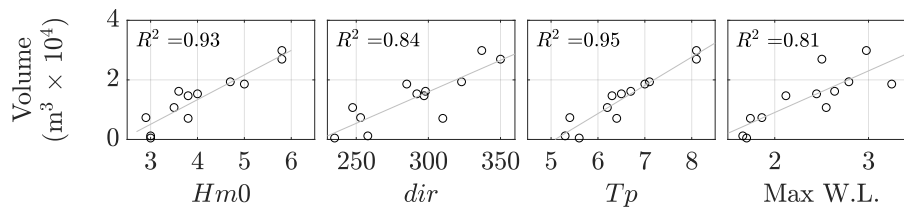
Figure 10. Scatter plot for the initial boundary conditions used for each scenario ( Hm_0 , Tp , dir and maximum water level) against total volume deposited onto the sand flat.
