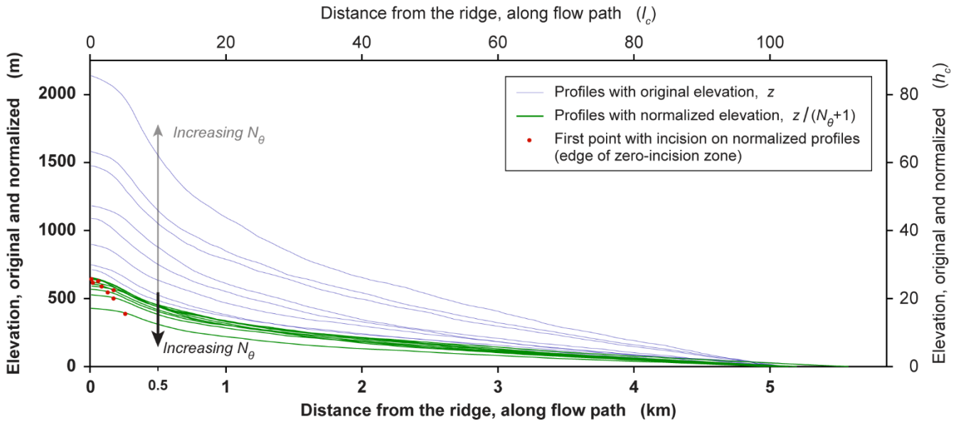
5 Figure 10: Equivalence of elevations that are normalized by N_\theta + 1 . Green lines show the profiles of Fig. 9 (shown again here with light blue lines), normalized by dividing by N_\theta + 1 . The normalized profiles largely collapse on each other. Along each profile, this tendency becomes stronger in the downstream direction, where the distance from the zone of zero incision grows (the edges of zero-incision zones are indicated by red dots). As N_\theta increases, the normalized profile elevations generally decrease slightly, whereas the original profile elevations increase substantially (see Table 5, which gives elevations, original and normalized, at a distance of 0.5 km from the ridge, which is roughly the location of the black arrow in this figure).
