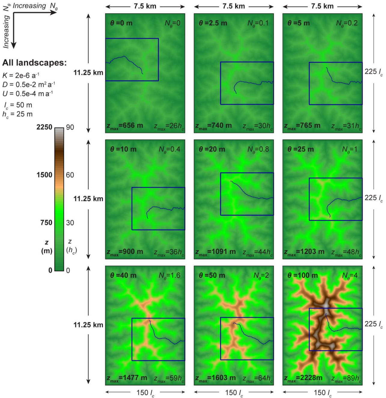
Figure 6: Increase of relief as the incision-threshold number N_\theta increases. Steady-state elevation maps of the nine landscapes of Sect. 3.2 (parameter values in Table 4) are plotted using a single elevation color scale, facilitating visual comparison of elevations across landscapes. The blue lines show the longest flow path of each landscape and the blue rectangles mark the regions that are magnified in Figs. 5, 7, and 8. The landscapes are arranged such that N_\theta increases from left to right and from top to bottom. By comparing the colors of the maps, we observe that landscapes with higher N_\theta values have greater relief (see also the maximum elevation of each landscape, displayed at the bottom of each map).
