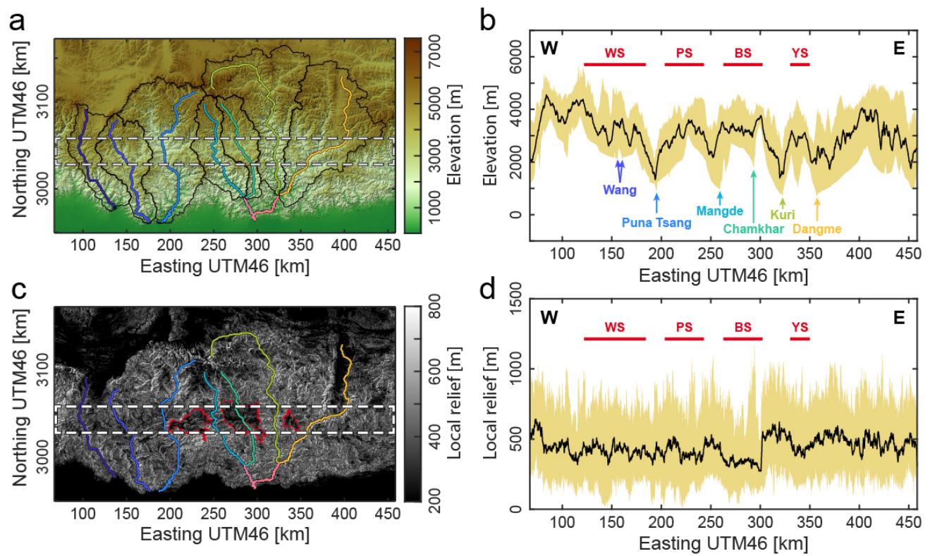
Figure 10: Topography and relief along the hinterland of the Bhutan Himalaya, where low-relief surfaces are located. WS: Wang Surface; PS: Phobjika Surface; BS: Bumthang Surface; YS: Yarab surface. a) Topographic map of the Bhutan Himalaya from ALOS World 3D – 30m (AW3D30) DEM data. Main drainage basins are delineated by black lines and associated main rivers are color-coded (color-code as in Figure 1). The dashed rectangle locates the swath profile represented in b). b) Topographic swath profile along the Bhutan hinterland, with elevations taken within the band illustrated in Figure 10a. Location of major rivers and of low-relief regions are reported.
