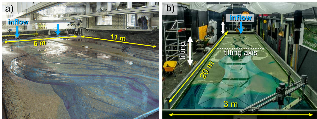
Figure 2. The flume setups of the two scale experiments tested in this study. (a) The Eurotank flume was used to simulate meandering and braided rivers in parallel on the left and right part of the flume, respectively (Van Dijk et al., 2013a). Water colour was converted to blue for visual comparison with (b) the second scale experiment in the tilting flume the Metronome that was used to simulate estuaries (Leuven et al., 2018). The flume is tilted over the short central axis, which steers flood and ebb flows that favour ample sediment transport in both tidal directions.
