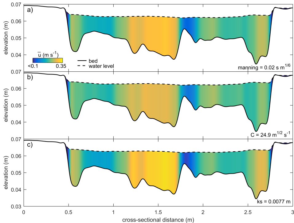
Figure 11. Effect of different hydraulic roughness predictors on the distribution of depth-averaged flow velocity \bar{u} for (a) a constant Manning, (b) a constant Chezy C and (c) a constant grain roughness k_s (White-Colebrook). The cross-section is from the experimental estuary by Leuven et al. (2018) at x = 15.3 m at maximum tilt in the ebb direction. Cross-sectional flow velocities were iterated for C and k_s assuming the same total discharge and water levels as modelled in this study with Manning.
