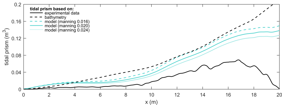
Figure 10. Tidal prism along the estuary based on experimental data, bathymetry and the model scenarios. Measured flow velocities were converted to depth-averaged velocities using Eq. (7). Tidal prism based on bathymetry (black dashed line) was computed as the cumulative volume of water along the estuary between high and low water levels imposed at the weir (i.e. with an amplitude of 4 mm) (cf. Braat et al., 2018); this calculation ignores effects of friction and river inflow.
