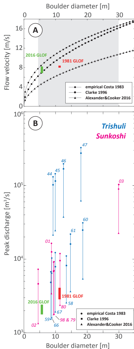
815 Figure 3: A- Theoretical flow velocities required to move boulders of a given diameter with explanatory input parameters (channel 820 bed slope 0.03, rock material density 2700 kg/m 3 , fluid density 1500 kg/m 3 ) according to the parametrisations and models of Costa (1983), Clarke (1996) and Alexander and Cooker (2016). The grey shaded area indicates range of boulder intermediate diameters mobilised during the 2016 and 1981 GLOF events in the upper Sunkoshi (Cook et al., 2018; Xu, 1988). The Clarke (1996) method is plotted with a channel bed slope adjusted to Cook et al. (2018) which is the gradient of the Sunkoshi reach at the location of boulder movement (0.0245). B- Estimated peak-paleo-discharges required to move the studied boulders according to the three models that were used for paleo-discharge calculations. Green and red rectangles are bounded by upstream and downstream estimates of observed boulder movements for the 2016 and 1981 GLOF events in the upper Sunkoshi (Cook et al., 2018; Xu, 1988).
