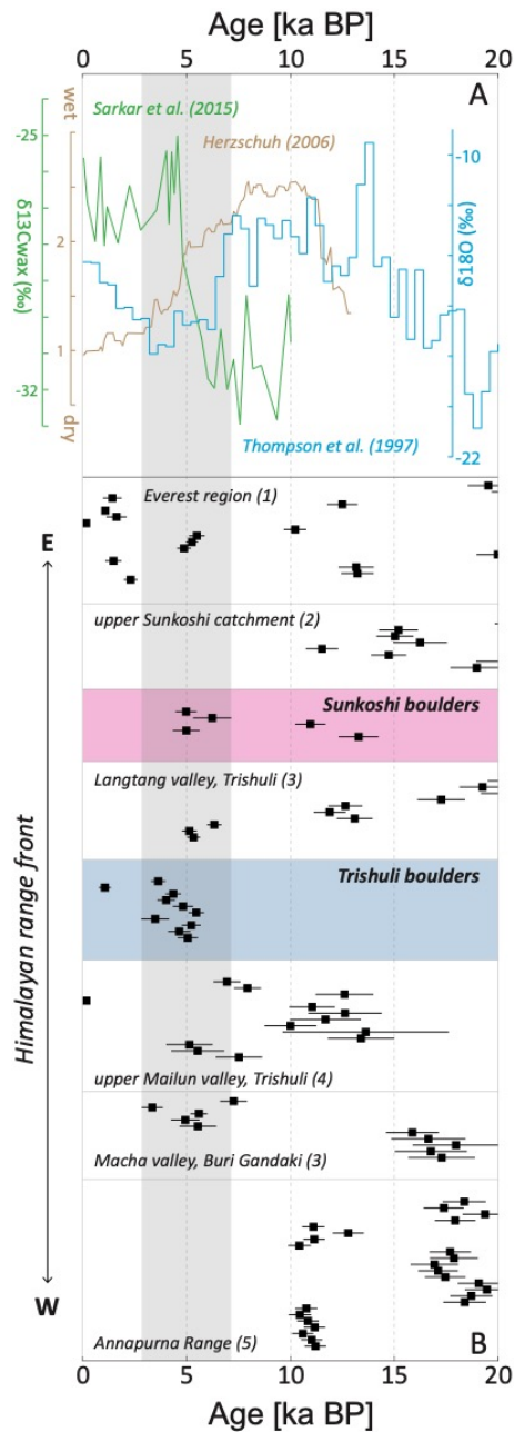
840 Figure 6: A- Climate proxy data: \delta^{18}\text{O} ice core measurements recovered on the Qinghai-Tibetan Plateau, China by Thompson et al. (1997); mean effective moisture index compiled from multiple paleoclimatic records in Indian monsoon dominated Asia by Herzschuh (2006); \delta^{13}\text{C}_{\text{wax}} (‰) vs VPDB lipid biomarker record from Lonar Lake central India by Sarkar et al. (2015). These proxies suggest a major climatic shift affecting monsoonal precipitation and consequently glacial dynamics on the south facing front at around 5 ka BP in the central Himalaya. B-: Boulder exposure ages in alignment with moraine deposits dated in the central Himalayan study region and recalculated consistently for better comparison: (1) Finkel et al. (2003), (2) Schaefer et al. (2008), (3) 845 Abramowski et al. (2003), (4) Gayer et al. (2006), (5) Pratt-Sitaula et al. (2011). 1\sigma uncertainties are given with horizontal bars. Realm of boulder ages around 5 ka BP is accentuated with grey shading.
