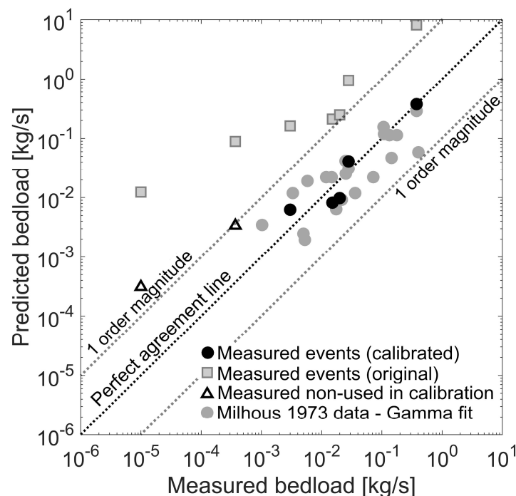
300 Figure 6: Comparison between measured and predicted bed load transport rate for different methods and data sets. Five events ( Q \geq 0.99 \text{ m}^3/\text{s} ) were used when calibrating Equation 8 (Eq. 8) (black circles). Triangles represent the estimated bed load using Equation 8 (Eq. 8) for two low flow events ( Q < 0.64 \text{ m}^3/\text{s} ) that were not used for calibration. The equation of Parker and Klingeman (1982) applied locally to the complete shear stress distributions is shown as reference (squares). Additionally, a synthetic spatial shear distribution based on equation 2 and the
