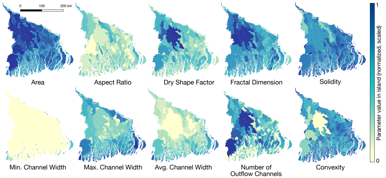
Figure 3. Map view of metrics after they have been normalized and scaled . The metrics are Each metric is normalized using a logarithmic normalization, and is shown scaled between 0 and 1.
