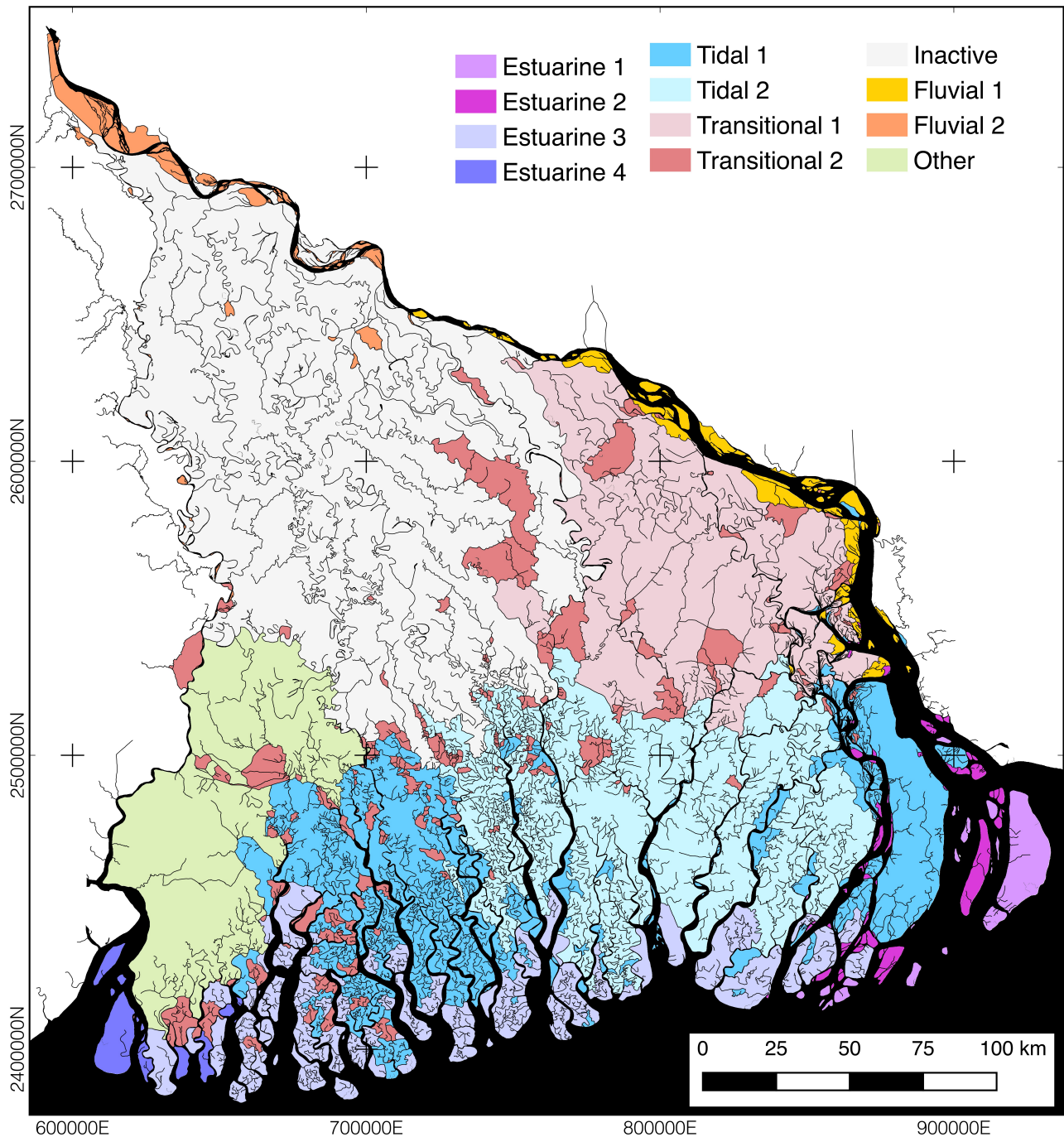
Figure 5. Delta Island classification -The as a result of the hierarchical agglomerative clustering method, using a geographic constraint so that only adjacent islands are can be grouped. Each island in the GBMD is classified into 14 twelve individual clusters belonging to 6. The twelve individual clusters are further grouped into six main classes using a dendrogram (Fig. 6). The six main groups include estuarine (purples), tidal (blues), transitional (pinks), inactive (gray), fluvial (oranges) and other (green).
