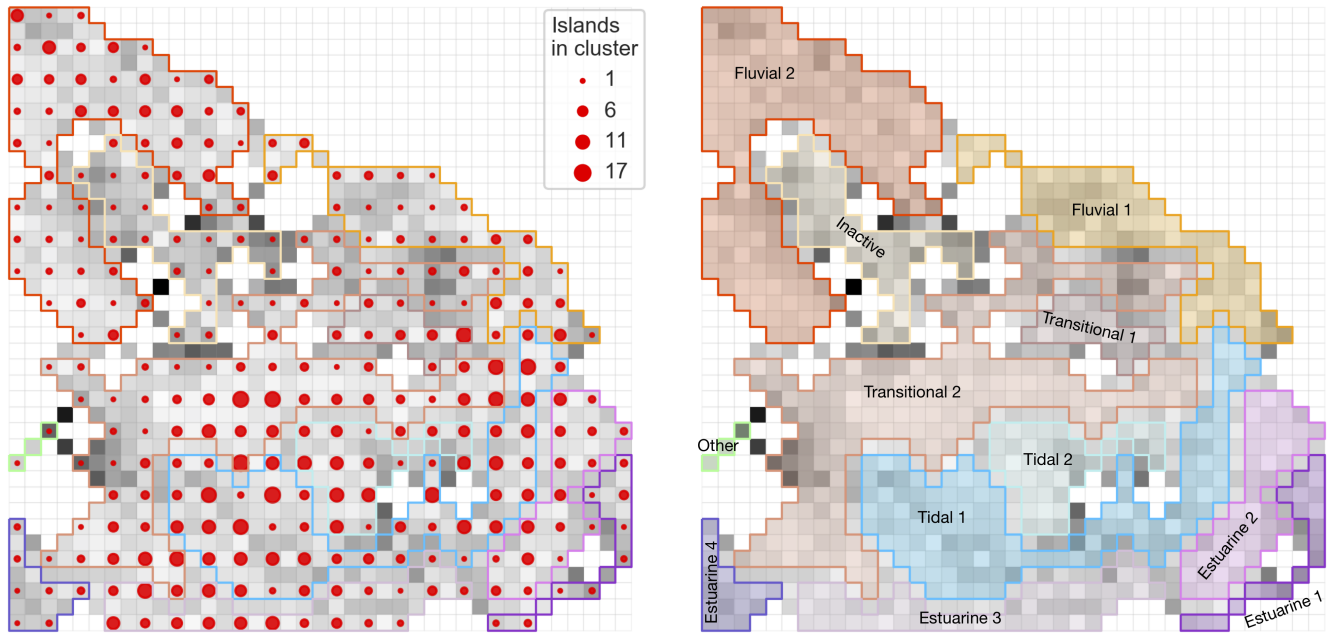
Figure 7. U-matrix. Islands are clustered into their The U-matrix (unified distance matrix) visualizes the number of adjacent islands within a node. Larger dots represent a greater number of islands, as determined by the GeoSOM method. Smaller dots represent a smaller number of islands. The colored outlines and shaded areas correspond to the six main classes or groups.
