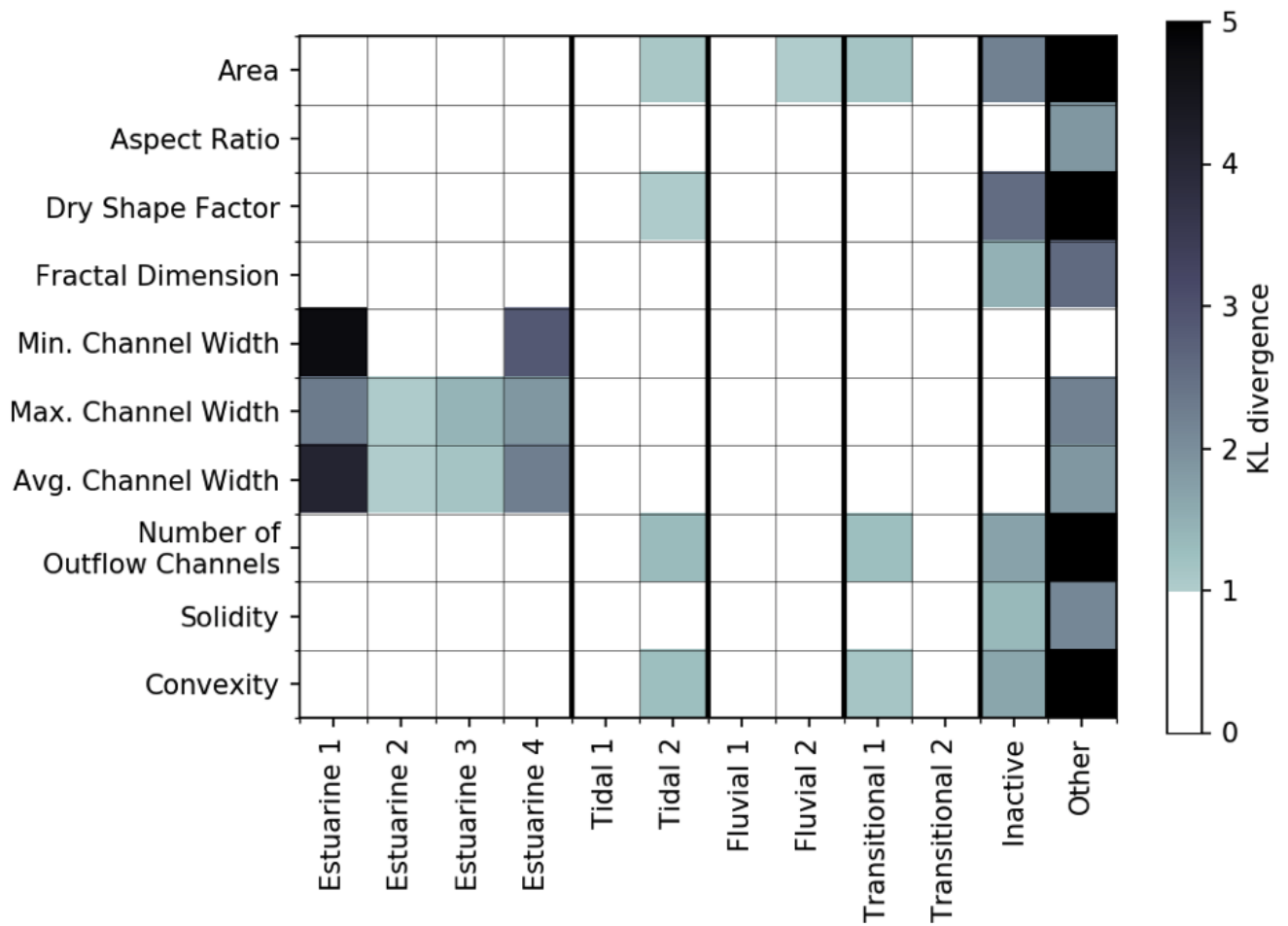
Figure 9. Kullback-Leibler divergence between the distribution of parameter values for islands of each class and all other islands for each variable. A value greater than +one indicates that the variable differentiates the population of islands in that class from those in other classes. A value less than +one shows that the distribution of values of that variable for that island class are similar to values for other islands.
