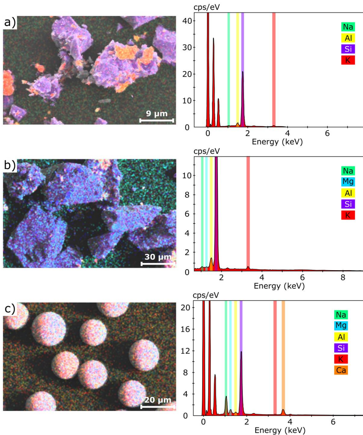
735 Figure 2: SEM qualitative analysis of the material composition. On the left is the BackScattered-Electron (BSE) imaging, while on the right the Energy-Dispersive Detector (EDS) spectrum. A qualitative composition is presented for a) silica powder, b) crushed quartz and c) glass microbeads. PVC powder has not been analyzed, due to its complex composition.
