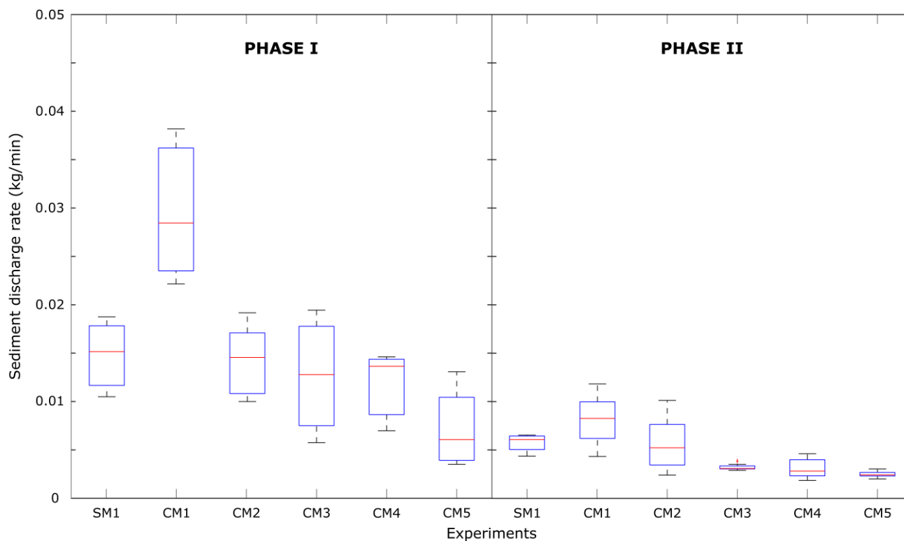
765 Figure 10: Box plot of sediment discharge rate for phase I and phase II. The red lines indicate the median, and the bottom and top edges of the blue box indicate the 25 th and 75 th percentiles, respectively. The black markers outside the box cover the data point at < 25 th and > 75 th percentile that are not considered outliers.
