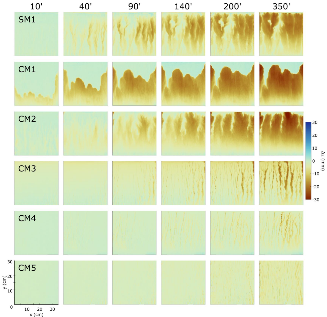
760 Figure 9: Erosion evolution for the experiments, here represented by the cumulative difference in elevation ( \Delta z ) of the same point at consecutive times. Time is indicated in columns. Each row corresponds to a model, where the mix adopted is indicated in the first panel of each row. The color coding is shown by the color bar on the right. Negative values correspond to erosion, positive ones to sedimentation (almost no sedimentation for these models).
