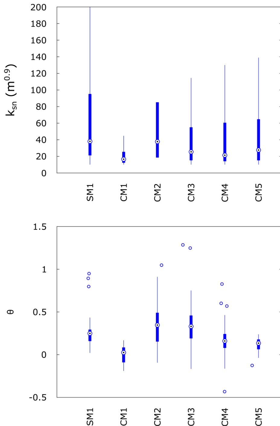
Figure 12: Steepness ( k_{sn} ) and concavity index ( \theta ) for the experiments. We use \theta_{ref} = 0.45 for computing k_{sn} . The black dots indicate the median, while the bottom and top edges of the blue box indicate the 25 th and 75 th percentiles, respectively. The thin blue lines cover data <25 th and >75 th percentiles that are not considered outliers, and the outliers are indicated by the blue empty dots.
