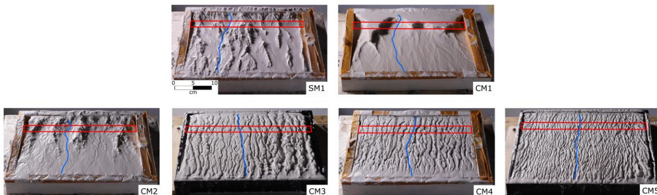
745 Figure 5: Pictures of the models at 200 min from the beginning of the experiment. The red box is the trace of the swath profiles shown in Fig. 6. The blue line indicates the stream, for every experiment, analyzed in Fig. 7.
