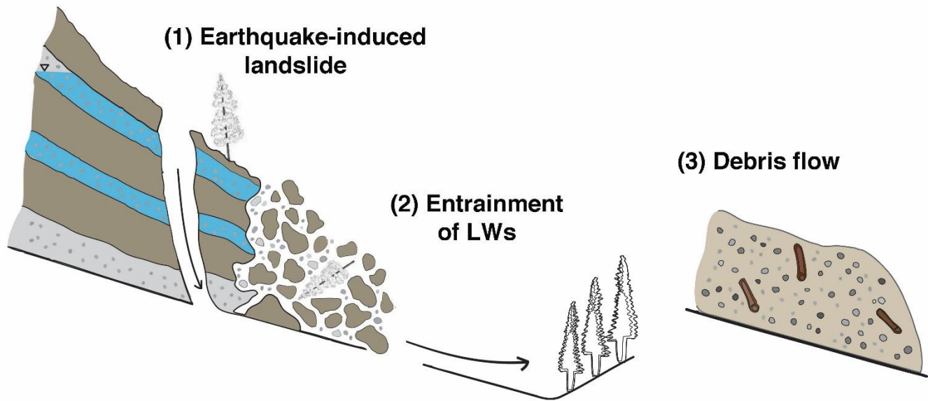
Figure 12: Conceptual model of transformation of earthquake-induced soil slips into debris flows at Popocatépetl volcano: (1) the earthquake produces the collapse of the saturated slope composed of a mix of ash and pumice; (2) the landslide impacts on the opposite side of the valley entraining a large amount of Large Woods (LWs) and (3) evolves into a debris flow due to the high water content of the material. The simplified stratigraphy in (1) reflects the one observed at the scar of Huitzilac landslide (see Figure 6c).
