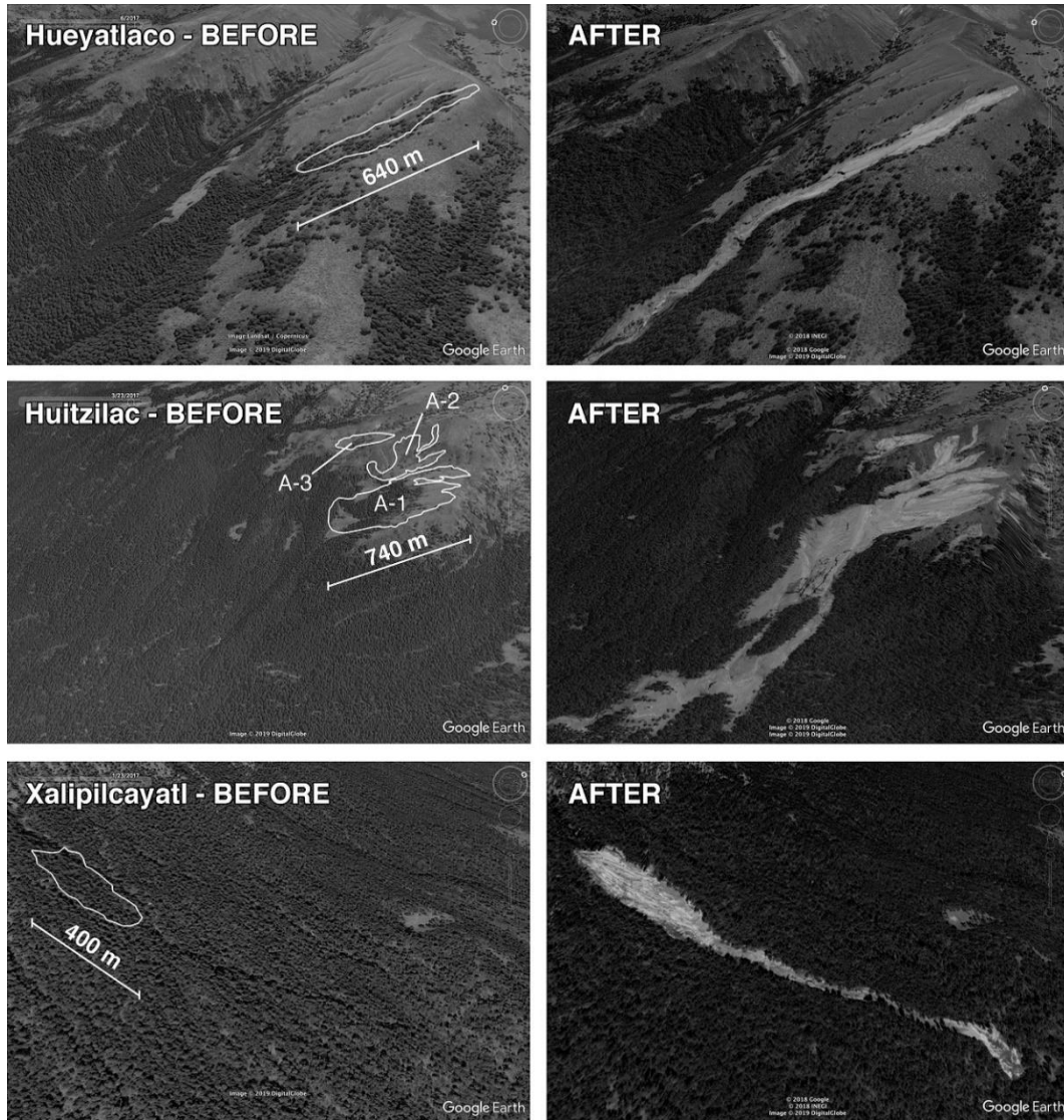
Figure 7: Major landslides that occurred in the headwaters of Hueyatlaco, Huitzilac and Xalipilcayatl ravines. Comparison of 3D views on the detachment areas before and after the landslides. Images from Google Earth (©Google 2018, ©INEGI 2018 and ©DigitalGlobe 2019).
