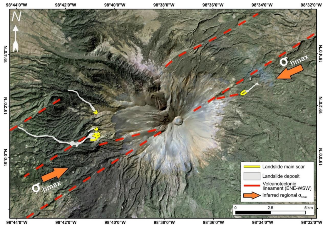
Figure 11: Simplified tectonic setting of the Popocatepetl area and location of the main landslides earthquake-induced landslides that occurred on 2017. Background image: ©DigitalGlobe/ESRI 2019.
