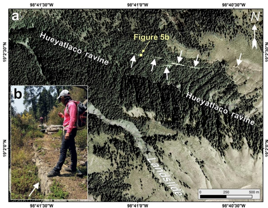
Figure 5: (a) Rectilinear extensional fractures and small normal faults opened parallel to Hueyatlaco ravine ( white arrows ), background image: Pléiades 1A image acquired on 13 November 2017. (b) Detail of the normal displacement of about 50 cm ( white arrow ).
