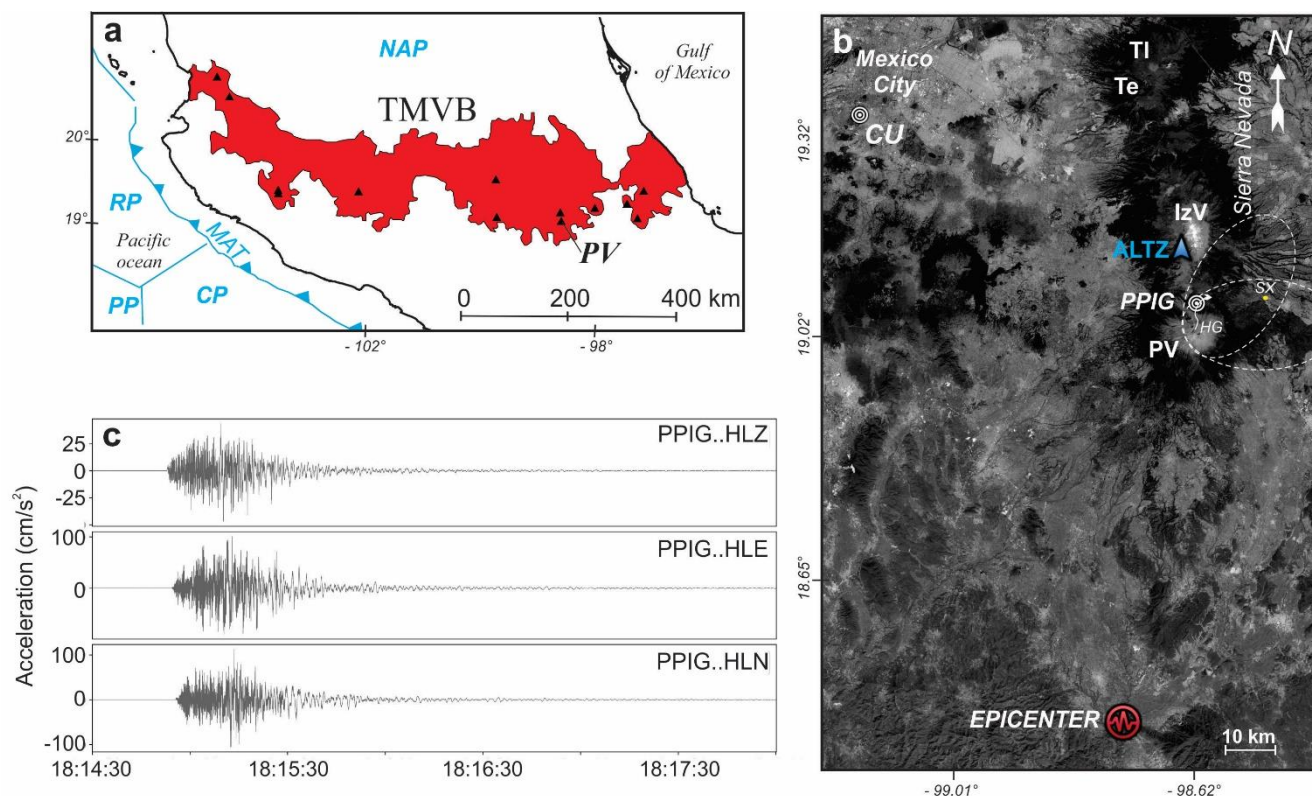
Figure 1: (a) Plate tectonic settings of Central Mexico ( CP Cocos Plate , MAT Middle American Trench , NAP North America Plate , PP Pacific Plate ) and location of Popocatepetl volcano (PV) in the Trans-Mexican Volcanic Belt (TMVB). (b) Details of the area affected by the M7.1 Puebla-Morelos earthquake and location of the seismic station CU and PPIG and of the rain gauge ALTZ (background image Landsat/Copernicus from Google Earth: ©Google 2020, ©INEGI 2020). (c) Strong motion recorded at station PPIG (SSN-UNAM) during the Puebla-Morelos earthquake on 17 September 2017.
