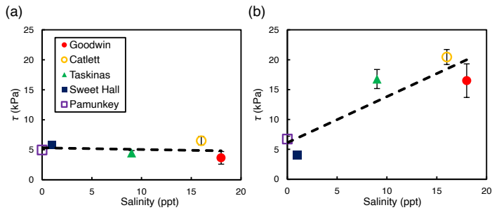
420 Figure 3: Relationship between salinity and shear strength ( \tau ) for edge sites (a) and interior sites (b). Each point represents the depth-averaged shear strength value for the upper 30 cm of the soil profile, where error bars represent the standard error associated with 10 replicate profiles for each site and location. Only the interior sites yielded a significant relationship between shear strength and salinity ( R^2 = 0.81 ; p = 0.04 ).
