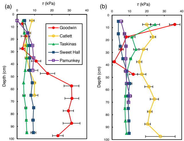
415 Figure 2: Average shear strength ( \tau ) profiles for marsh edge (a) and marsh interior (b) locations at each study site. Each profile represents the average of 10 replicate profiles, where error bars represent standard error.
