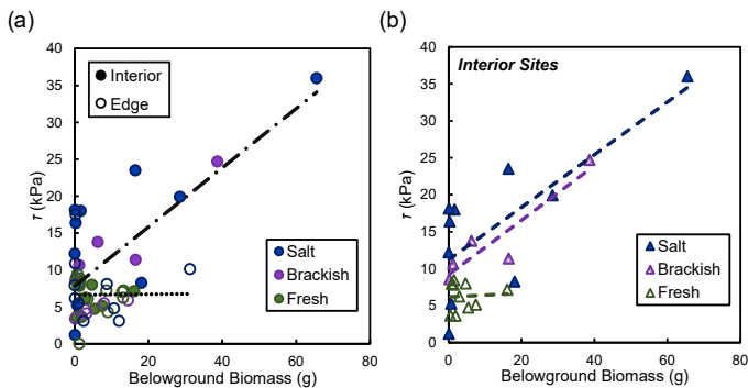
430 Figure 5: (a) Shear strength ( \tau ) compared to live belowground biomass for edge (open circles) and interior (closed circles) locations, broken down by salinity type (salt = Goodwin and Catlett, brackish = Taskinas, fresh = Sweet Hall and Pamunkey). Each point represents a biomass measurement with its associated shear strength value at concurrent depths in the soil profile. Only the relationship between belowground biomass and shear strength in the interior was significant ( R^2 = 0.58 ; p = 1.09e- 435 5). (b) Relationships between belowground biomass and shear strength ( \tau ) from (a) for interior sites only, broken down by salinity type (same as (a)). Only the relationships between salt ( R^2 = 0.57 ; p = 0.012 ) and brackish ( R^2 = 0.86 ; p = 0.025 ) sites were significant.
