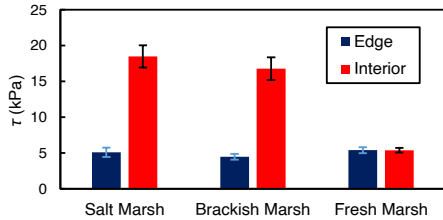
425 Figure 4: Average shear strength ( \tau ) values for marsh edge and interior locations. Salt marsh locations are Goodwin Islands and Catlett Islands, brackish marsh location is Taskinas Creek, and freshwater marsh locations are Sweet Hall Marsh and the Pamunkey Indian Reservation. Each column represents the depth-averaged shear strength for the upper 30 cm of soil of each marsh type. Error bars represent the standard error of 10 replicate shear strength profiles for each marsh type.
