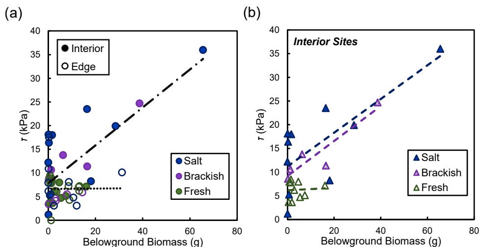
415 Figure 5: (a) Shear strength ( \tau ) compared to live belowground biomass for edge (open circles) and interior (closed circles) locations, broken down by salinity type (salt = Goodwin and Catlett, brackish = Taskinas, fresh = Sweet Hall and Pamunkey). Each point represents a biomass measurement with its associated shear strength value at concurrent depths in the soil profile. Only the relationship between belowground biomass and shear strength in the interior was significant ( R^2 = 0.58 ; p = 1.09e-5 ). (b) Relationships between belowground biomass and shear strength ( \tau ) from (a) for interior sites only, broken down by salinity type (same as (a)). Only the relationships between salt ( R^2 = 0.57 ; p = 0.012 ) and brackish ( R^2 = 0.86 ; p = 0.025 ) sites were significant. 420
