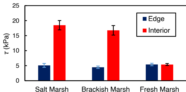
410 Figure 4: Average shear strength ( \tau ) values for marsh edge and interior locations. Salt marsh locations are Goodwin Islands and Catlett Islands, brackish marsh location is Taskinas Creek, and freshwater marsh locations are Sweet Hall Marsh and the Pamunkey Indian Reservation. Each column represents the depth-averaged shear strength for the upper 30 cm of soil of each marsh type. Error bars represent the standard error of 10 replicate shear strength profiles for each marsh type.
