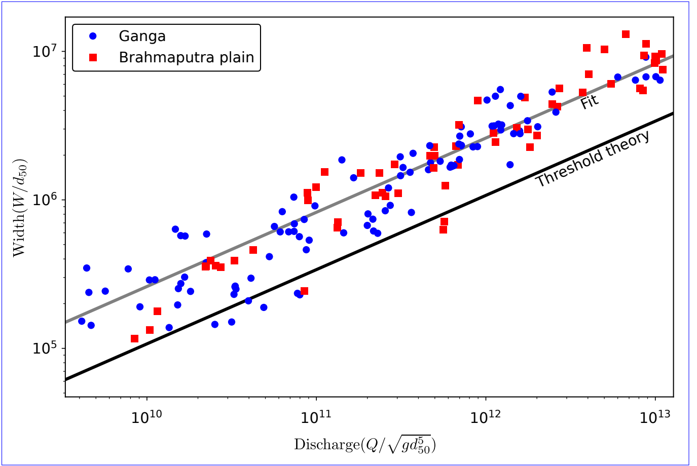
Figure 2. Width of the individual threads of the Himalayan Foreland rivers as a function of water discharge (after: Gaurav et al. (2017)). The solid line (dark) is the prediction from threshold theory and the solid line (light) is obtained by fitting the prefactor of the threshold relation (Eq.4) to the data while keeping the theoretical exponent.
