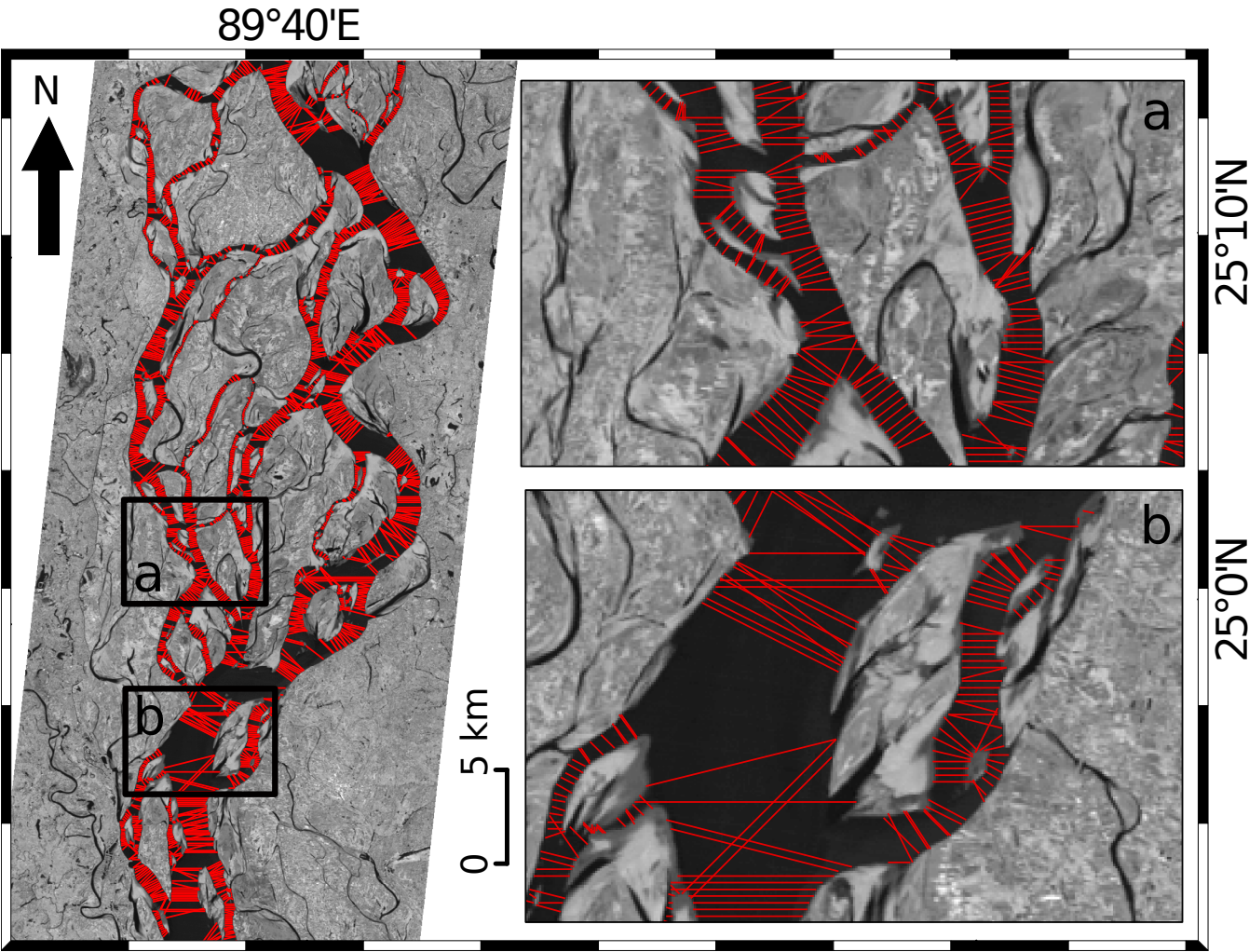
Figure 5. Width of the individual threads estimated across different transects along a reach of the Brahmaputra river from Landsat satellite image. Windows (a) and (b) illustrate the regions of valid and erroneous transects at different places in the river (image source: Landsat-TM, 29 November 2013).
