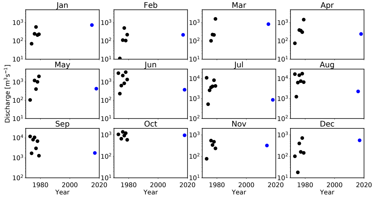
Figure 2: Time series of discharge of the Indus River (circle in black) measured at the ground station (Kotri). Circle in blue is the discharge estimated from satellite images.
