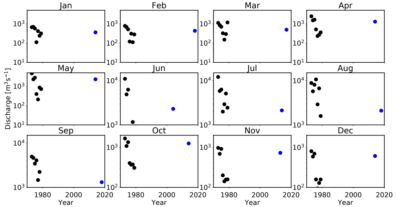
Figure 3: Time series of discharge of the Chenab River (circle in black) measured at the ground station (Panjnad). Circle in blue is the discharge estimated from satellite images.
