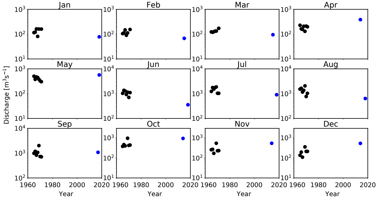
Figure 4: Time series of discharge of the Teesta River (circle in black) measured at the ground station (Anderson bridge). Circle in blue is the discharge estimated from satellite images.
