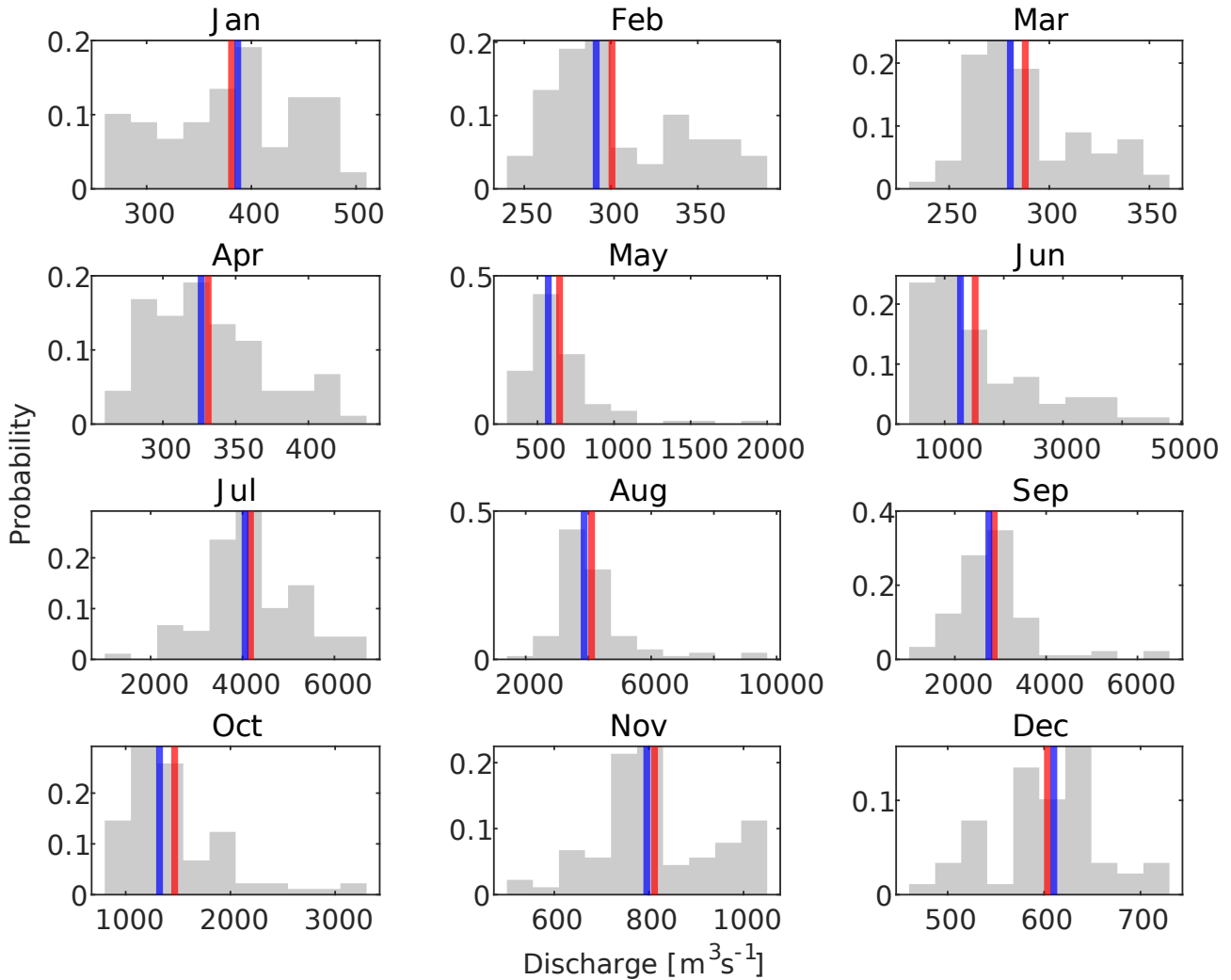
Figure 6: Histogram of daily discharge of the Kosi River measured at the Bhimnagar barrage in 2011, 2013, and 2014. Vertical lines in red and blue are the mean and median values of the probability distribution.
