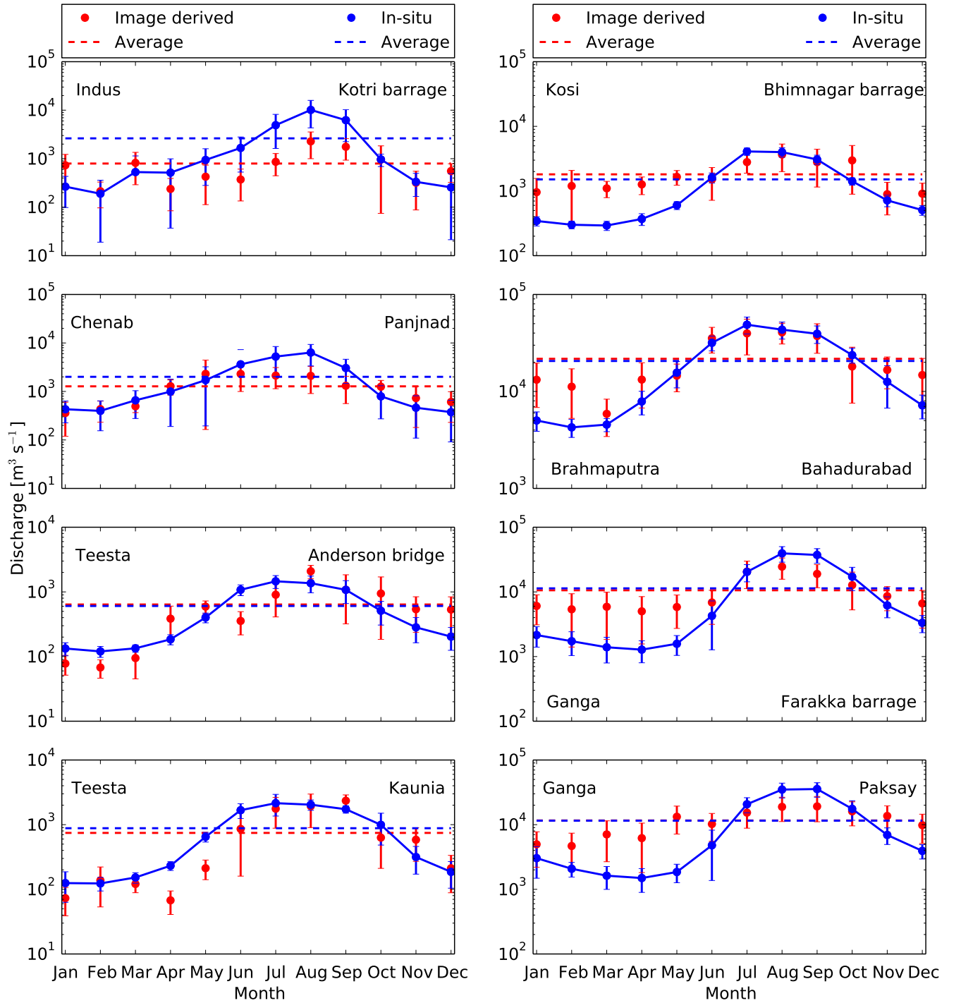
Figure 9. Hydrograph of satellite derived river discharge against their monthly average discharge recorded at the gauging station. Dotted red and blue lines are the annual average discharge obtained from satellite images and in-situ measurement respectively.
