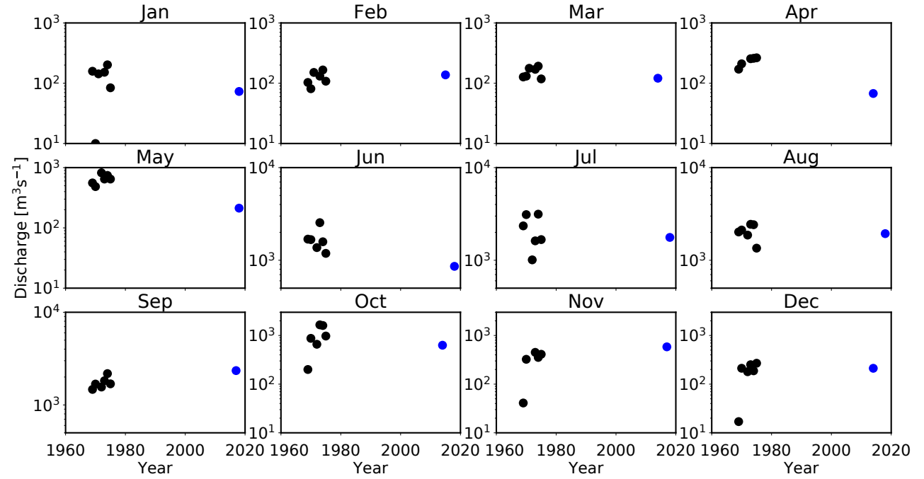
Figure 5: Time series of discharge of the Teesta River (circle in black) measured at the ground station (Kaunia). Circle in blue is the discharge estimated from satellite images.
