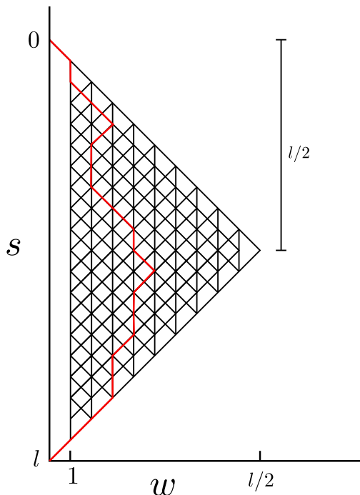
Figure 1: Conceptual diagram showing all possible paths of the width function for a watershed of length, l . The red line is one realization. The ensemble of paths is symmetrical about l/2 and the boundary condition is illustrated by no paths reaching w = 0 before l .
