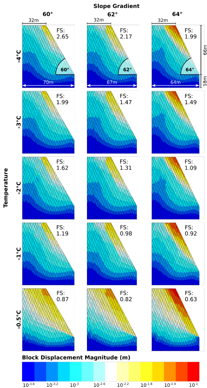
465 Figure 7: Numerically calculated block displacements (on the log scale) for a simplified rock slope geometry with exemplary inclinations of 60°, 62° and 64°, and five temperatures between -4 and -0.5 °C.
