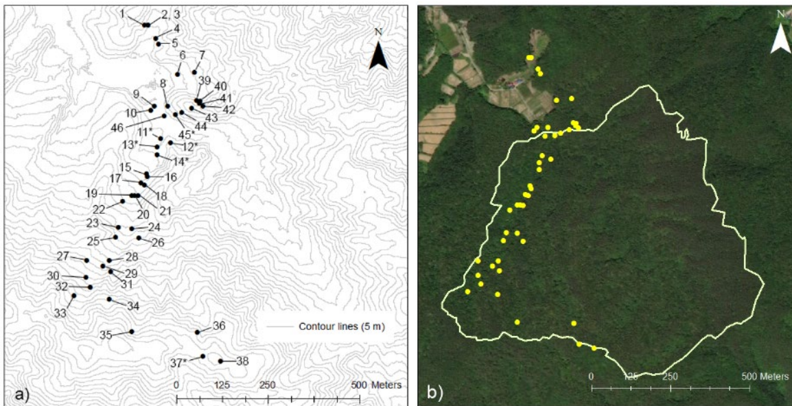
105 Fig. 3. Study site topography and aerial images. a) Numbered sample locations where multi-year samples were collected at the locations marked by * and contour lines are at 5-m intervals (Basemap: ESRI). b) A large basin enclosing the longest slope (Basemap: ESRI).
