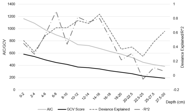
c) Model performance indices for Model A in Table 7.
