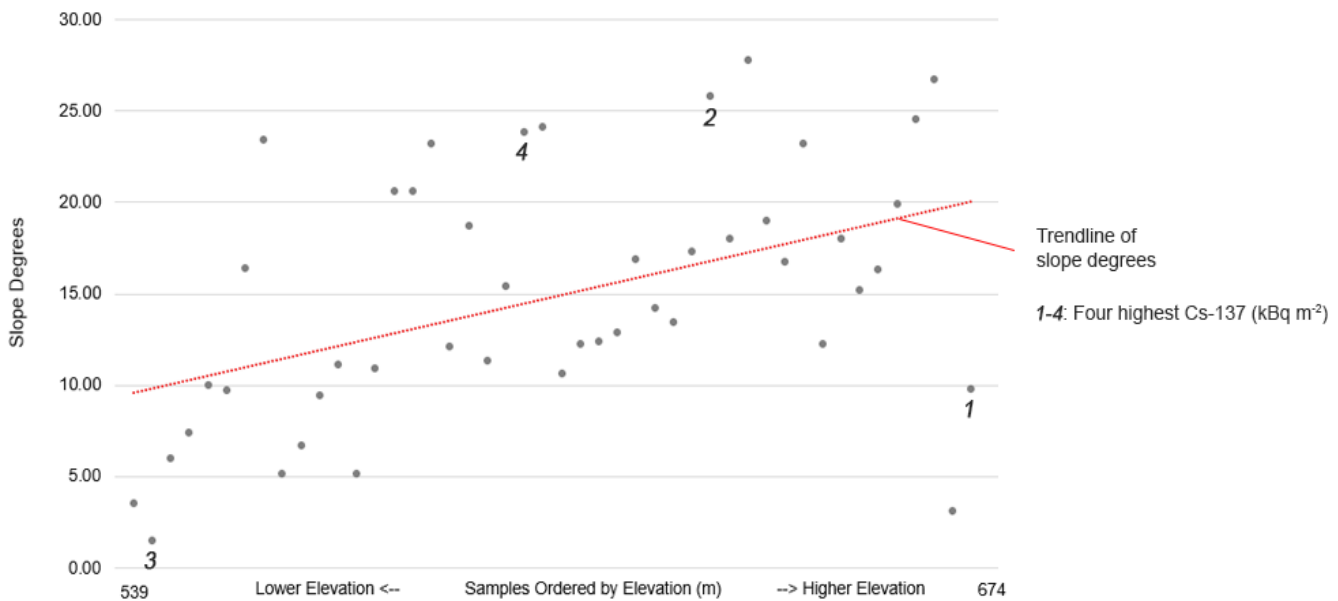
295 Fig. 8. Slope (degrees) of sampling points along the elevation (m). The numbers 1-4 correspond to the same numbers in Fig. 7.
