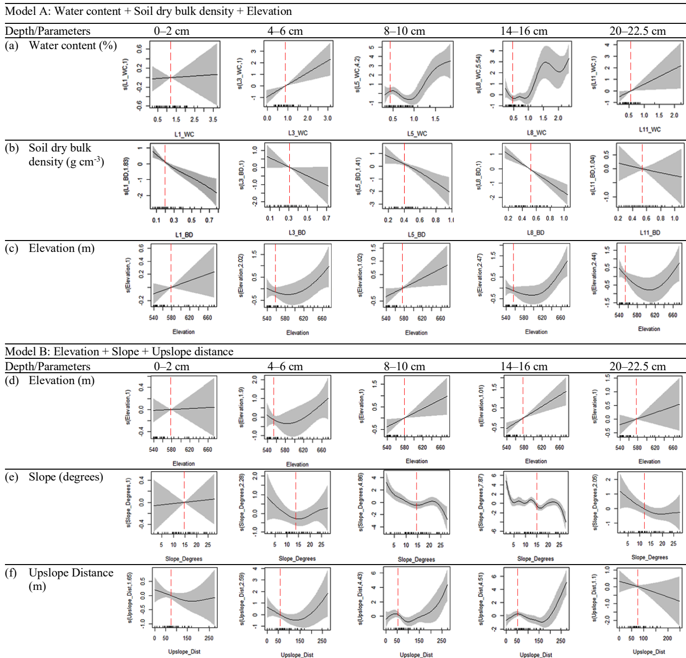
Fig. 13. GAM smooth function outputs at five depth layers for the parameters in the two best performing models. The x-axis on each plot is the model predictor and its real value range. The y-axis is the smoothing parameter, s(\text{covariate}, \text{degree of freedom}) . Vertical red dashed lines indicate a point at which the smoothing parameter is the zero residual point.
