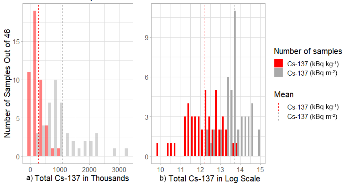
245 Fig. 4. Distribution of mass-based total Cs-137 in a core sample. (a) A unit of each bin is 200 k. (b) Distribution of total mass depth Cs-137 in a core sample in a log scale (red: Cs-137 \text{kBq kg}^{-1} ; grey: Cs-137 \text{kBq m}^{-2} ).
