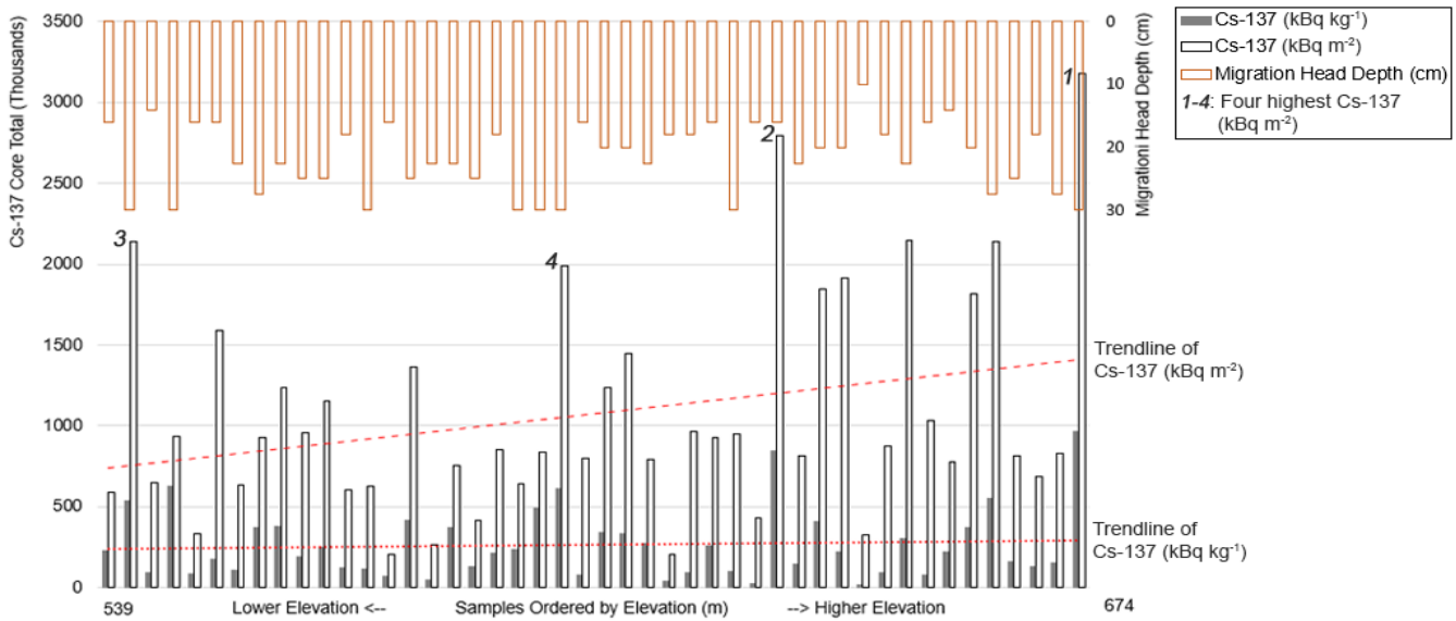
290 Fig. 7. Core total Cs-137 in both units along the elevation (m). Numbers 1-4 indicate the samples with the four highest Cs-137 concentrations in \text{kBq m}^{-2} . Migration head depths (cm) are the depths at which Cs-137 concentrations decreased to 100 \text{ Bq kg}^{-1} in a core sample.
