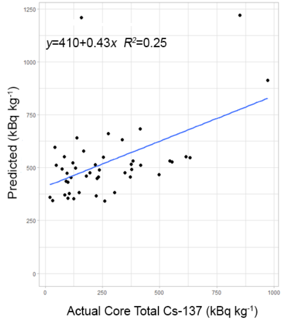
b) A scatter plot of the actual core total Cs-137 and the predicted Cs-137, using Model B setting in Table 7.
