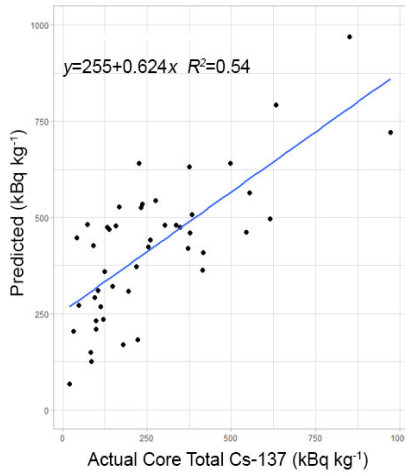
a) A scatter plot of the actual core total Cs-137 in and the predicted Cs-137, using Model A setting in Table 76.
