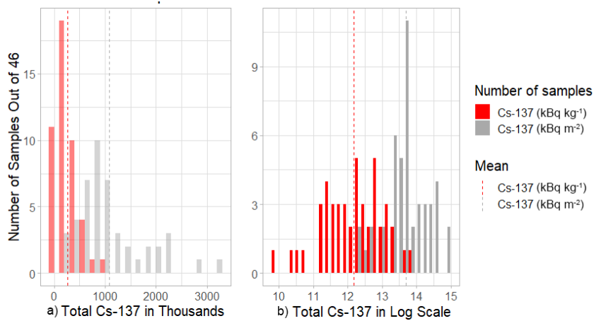
Fig. 4. Distribution of mass-based total Cs-137 in a core sample. (a) A unit of each bin is 200 k. (b) Distribution of total mass depth Cs-137 in a core sample in a log scale (red: Cs-137 kBq kg -1 ; grey: Cs-137 kBq m -2 ).
