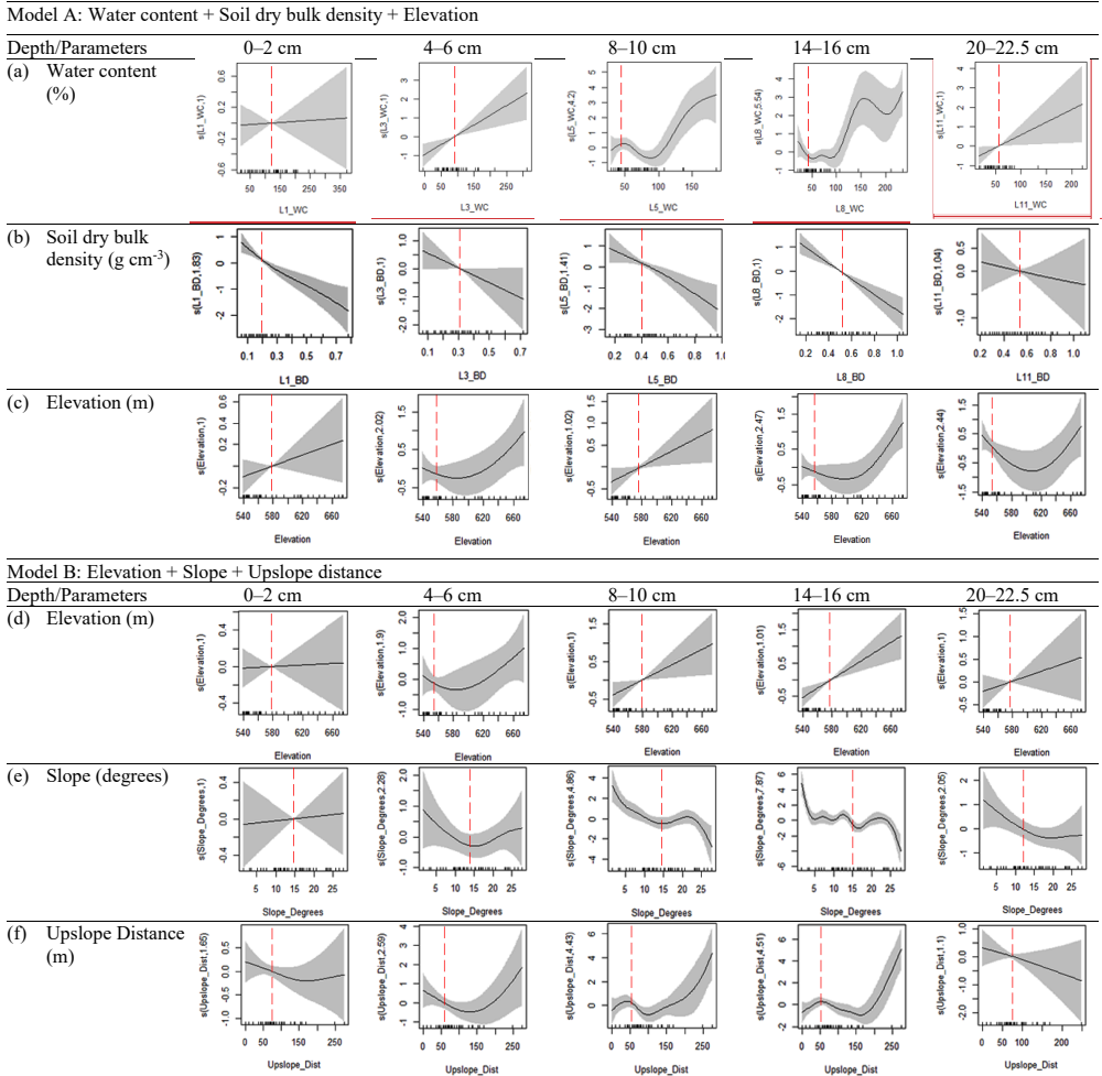
Fig. 13. GAM smooth function outputs at five depth layers for the parameters in the two best performing models. The x-axis on each plot is the model predictor and its real value range. The y-axis is the smoothing parameter, s(\text{covariate, degree of freedom}) . Vertical red dashed lines indicate a point at which the smoothing parameter is the zero residual point.
