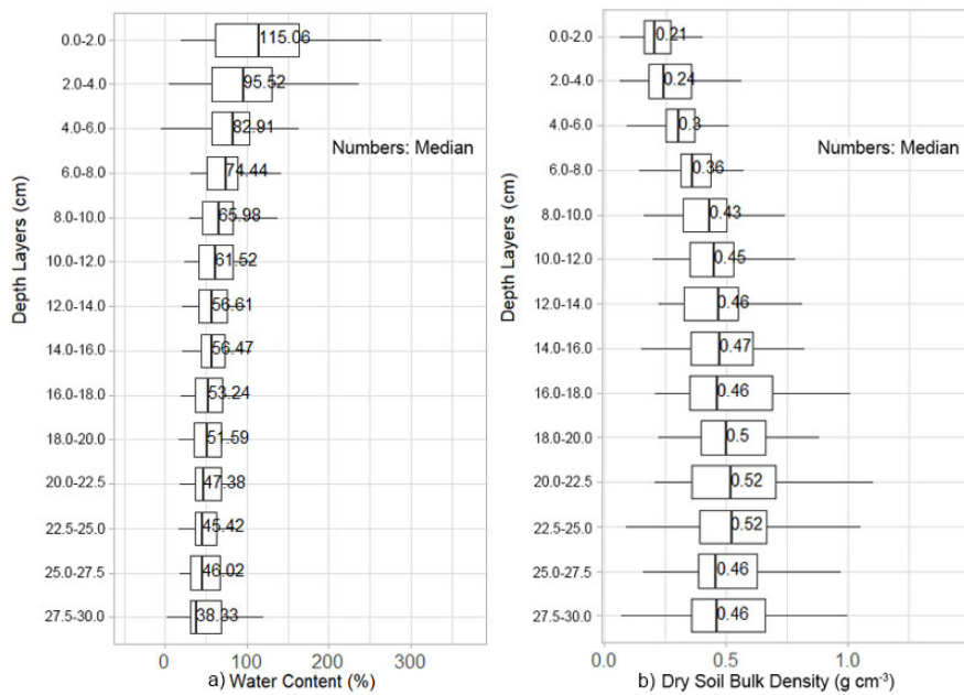
Fig. 6. Depth profiles of (a) water content (%) and (b) soil dry bulk density ( \text{g cm}^{-3} ).
