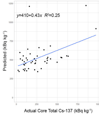
b) A scatter plot of the actual core total Cs-137 and the predicted Cs-137, using Model B setting in Table 76.
