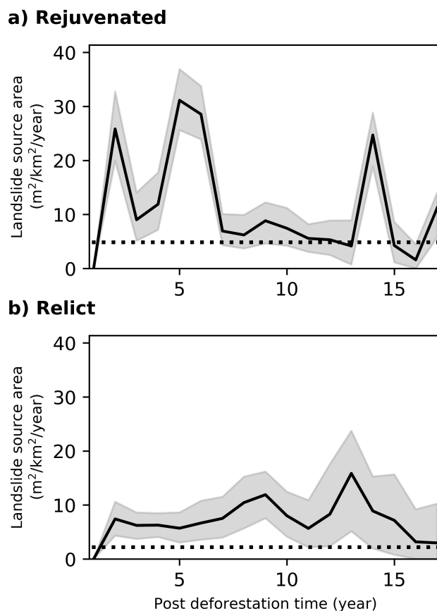
Figure A1. Deforestation-induced landslide wave in different geomorphic contexts. Overall landslide source area ( LS_s , \text{m}^2 \text{ km}^{-2} \text{ year}^{-1} ) in function of time elapsed since deforestation. The grey area represents the 90 % confidence interval, derived from 100 iterations of LS_s calculations (Section 3.2.4). The dotted line shows the overall erosion rates in the different contexts. a) Rejuvenated —Landslide response to deforestation in rejuvenated landscapes, characterized with 193 landslide instances. The irregular curve suggests that we need more landslide observations , in order to better characterize the deforestation-induced landslide wave, we need more landslide and deforestation observations and over a larger area . b) Relict —Landslide response to deforestation in relict landscapes, characterized with 181 landslide instances. The dotted line represents the background erosion rate in relict landscapes.
