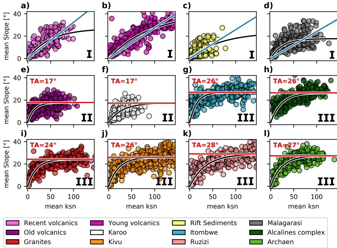
Figure 8. Threshold slope analysis for the different lithostratigraphical units in the NTK Rift. Based on Each point represents a first order river catchment over which we averaged the trends of the landscape-slope gradient S versus the and normalized river steepness index k_{sn} . The black curves represent the S = f(k_{sn}) relationship is presented by the black curve on each subplot; fitted to Eq. (2), both averaged over first-order river catchments. a)→d) Category I Young lithostratigraphy for which no clear threshold angle is observed. e)→f) Category II Young lithostratigraphy with a low threshold angle of ca. 17^\circ . g)→l) Category III Older rocks with higher observed threshold slopes of 24-28^\circ .
