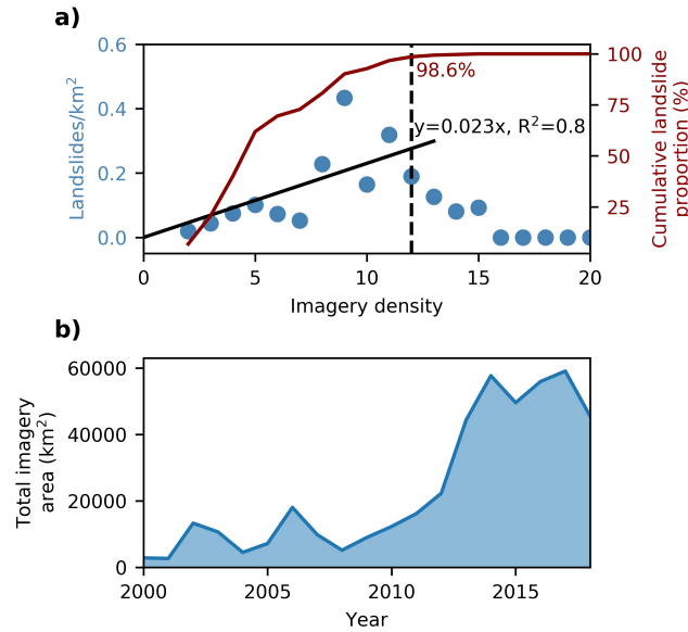
Figure 9. Visualization of the imagery bias in © Google Earth. a) Imagery-range The impact of imagery density (the number of available images in © Google Earth) on the number of observed landslides. We only show the results for the rocks of Category III (Section 4.1). b) Imagery Therefore, major cities that are characterized by a high imagery density like Bukavu, Bujumbura, and Goma are excluded from this figure. c) a) Impact of the imagery density on the number of observed landslides. d) The number of landslides seems to increase linearly with imagery density up to 12 images. The cumulative landslide proportion for a certain value shows the % of the landslide inventory contained in areas with an imagery density equal or lower than that value. b) The evolution of imagery availability between 2000 and 2018.
