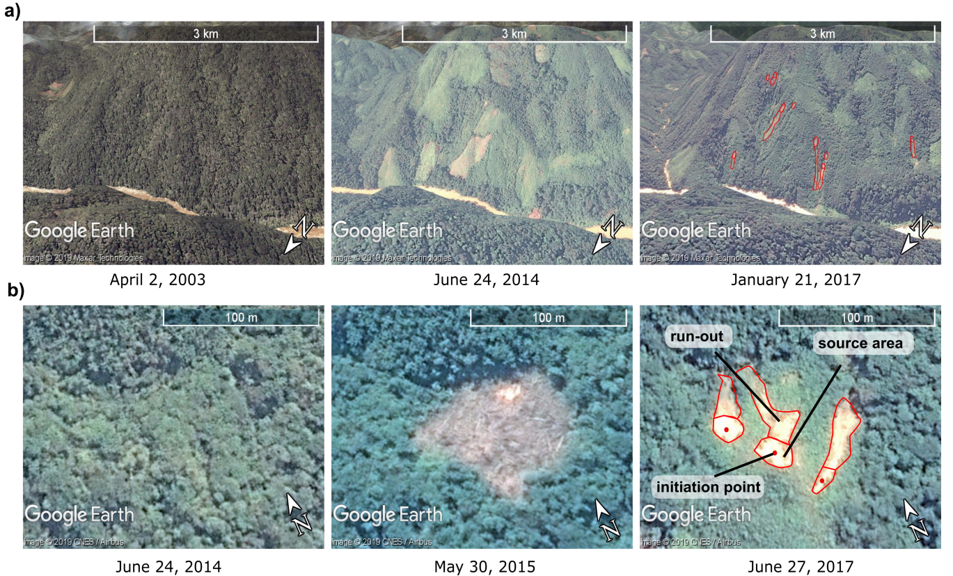
Figure 4. Examples of deforestation followed by landsliding. a) Landslide event North-north of Butezi, DRC (28.296984° E, 2.843201° S; image ©2019 Google Earth). b) Landslide event in Matala, DRC (28.360656° E, 2.645874° S; image ©2019 Google Earth).
