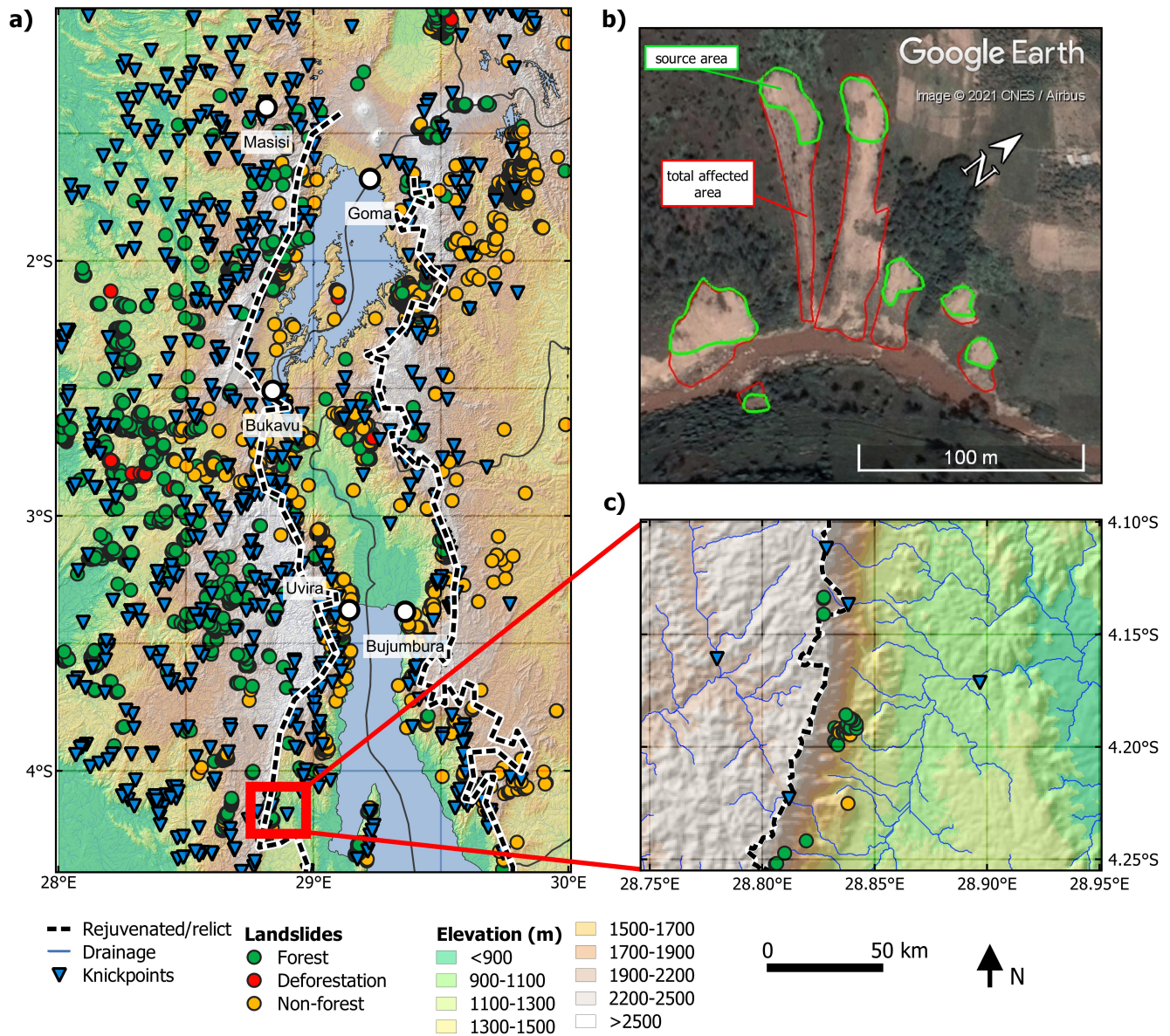
Figure 7. Landslide and knickpoint inventory for the NTK Rift. a) We identified 7994 7,994 shallow recent landslides and 834 knickpoints that occurred either in forest, of which non-forest or after deforestation, and 673 were considered non-stationary knickpoints . These knickpoint knickpoints were used to separate the rejuvenated landscapes between the Rift shoulders from the surrounding relict landscapes ( black-and-white line ). b) Example of shallow landslides in Rwanda (29.7909 °E, -1.7151 °S) and the delineation of their total area (red) and source area (green). c) Example of the Rift shoulder west of Lake Tanganyika. The method for delineating the rejuvenated landscapes is specified in Section 3.1.2.
