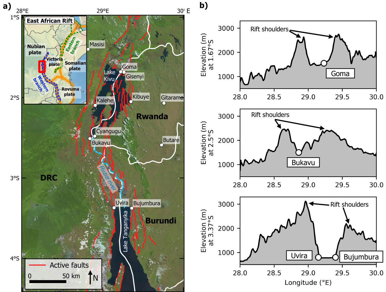
Figure 1. Overview of the NTK Rift. a) Extent of the studied area and active faults (Delvaux and Barth, 2010)). LANDSAT-8 imagery is used as background (USGS, 2018). b) The transects of the elevation at different latitudes illustrate the elevated Rift shoulders, being the result of tectonic uplift. The four most populous cities of the NTK Rift (Goma, Bukavu, Uvira, Bujumbura) are located in between the Rift shoulders.
