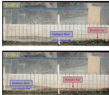
Figure 1. boulder bar obstructs the outburst flow to the river bed lower reaches
