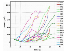
Figure. 6 Volumes of boulder bars. Notation: UV i , MV i , DV i , MUV i , MDV i represent the volume of the boulder bar near the upstream reaches, the boulder bar near the middle reaches, the boulder bar near the downstream reaches, the boulder bar near the middle-upstream reaches, and the boulder bar near the middle-downstream reaches, respectively. For example, UV1 means the volume of the boulder bar near the upstream reaches of the T1 test.
