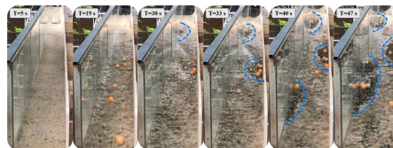
Figure. 3 The riverbed morphology at six different moments during the boulder bars' formations and growths process for the T7 experiment. The boulder bars in the figure are marked with blue dotted lines.
