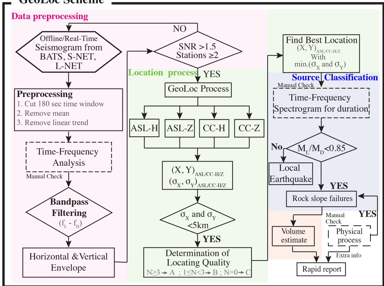
Figure 2. Flowchart of the GeoLoc scheme, including data preprocessing, location process, source classification, and volume estimate. All steps are automatic, except the steps with grey background rectangular dashes which involved manual check in this research. f_L and f_H are the lower and upper band of the bandpass filtering. (X, Y)_{ASL/CC-H/Z} is the best location form the ASL or CC with horizontal or vertical components. (\sigma_X, \sigma_Y)_{ASL/CC-H/Z} are those location uncertainties based on the relative fitness over 0.95. -N is the number of results from methods_ with components (total: N=4 ) whose location error less than 5 km threshold. The result with minimum location error defines the best location.
