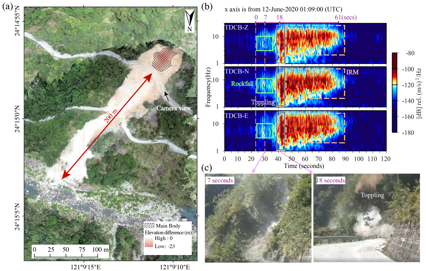
520 Figure 7. The field photo, spectrograms, and time-lapse photos from the video of recent RSF on the 12 th of June 2020. (a) Field photo of the event. The gradient red color scale is the elevation difference between DEM originating from Lidar in 2012 and, the digital surface model (DSM) derived from drone survey after the event. The main body is considered the elevation difference larger than 3m. The black arrow indicates the camera view, and the red arrow is the distance between the road and river bed. (b) The spectrograms of three components. The upper left corner of the spectrograms is the station name with the components. The green, white with black lines, and orange rectangles are the spectrogram features of the physical process corresponding to rockfall, toppling (T phase), and complex process of the rock interaction with slope (IRM phase), respectively. The purple axis below spectrograms vertical purple dashed line indicates the time points from the video. (c) Time-lapse photos from the video corresponding to the physical process of rockfall (Left panel) and toppling (Right panel). The seconds shown in the top-left corner indicate a time tag in the video.
