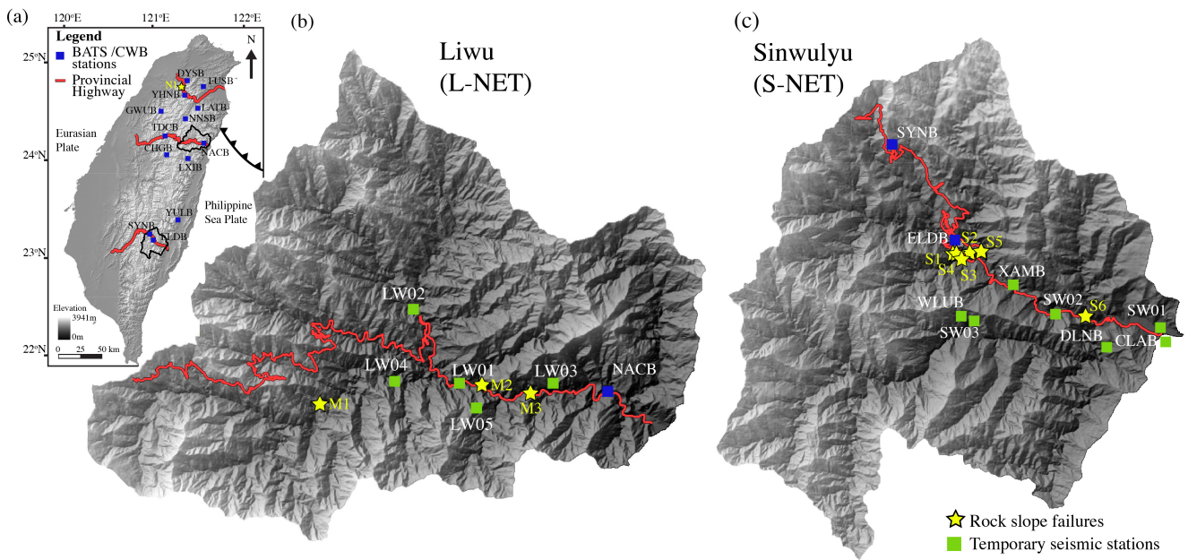
465 Figure 1. Research area and distribution of seismic stations and ten rock slope failures (RSFs, yellow star). (a) Topographic map of Taiwan shows three provincial highways (red lines) and BATS/CWB stations (blue square). (b) Liwu catchment, the east flank of the central provincial highway, and the temporary seismic network (L-NET, green-pink square). (c) Sinwulyu catchment, the east flank of the southern provincial highway, and the temporary seismic network (S-NET, pink-green square). The data of Digital Elevation Model (DEM) of Taiwan and two catchments are from Government Open Data Platform, Taiwan.
