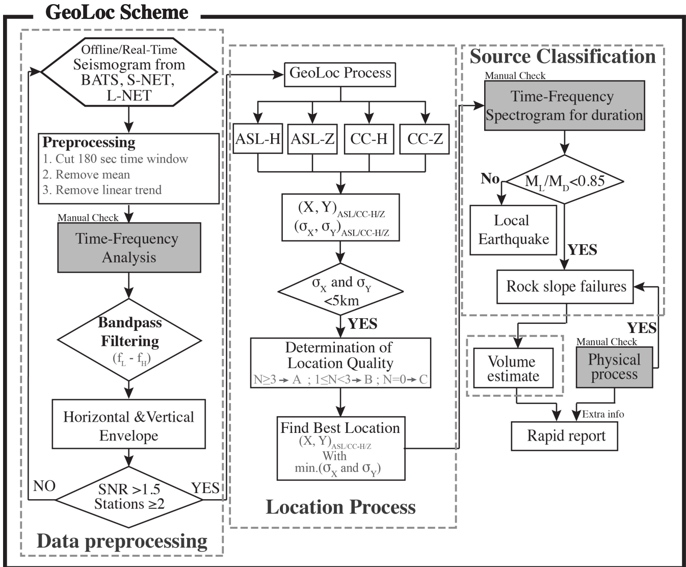
470 Figure 2. Flowchart of the GeoLoc scheme, including data preprocessing, location process, source classification, and volume estimate. All steps are automatic, except the steps with grey background which involved manual check in this research. f_L and f_H are the lower and upper band of the bandpass filtering. (X, Y)_{ASL/CC-H/Z} is the best location form the ASL or CC with horizontal or vertical components. (\sigma_X, \sigma_Y)_{ASL/CC-H/Z} are those location uncertainties based on the relative fitness over 0.95. N is the number of results from methods with components (total: N=4 ) whose location error less than 5 km threshold. The result with minimum location error defines the best location.
