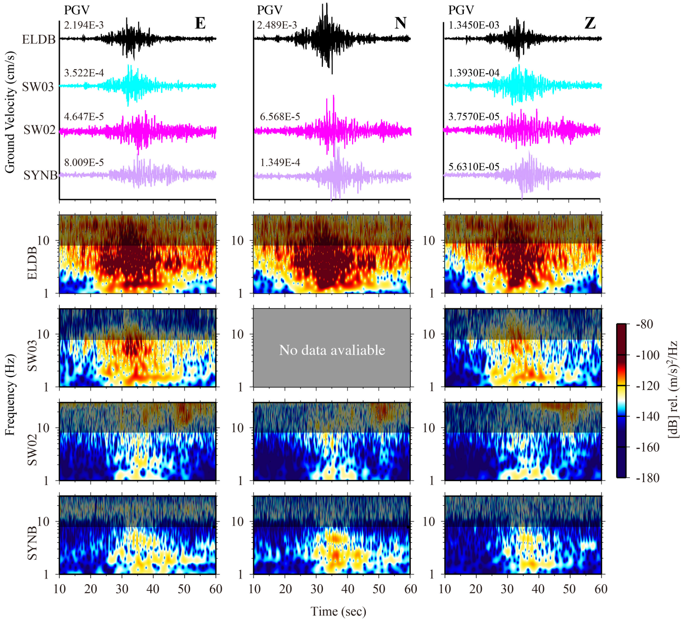
Figure 3. Recorded waveform and spectrogram of Event S4. The value next to the waveform is the peak ground velocity (PGV) for each signal. The bright area of the spectrogram is the range of the bandpass filter (1-8Hz, f_L to f_H ), which should cover the signals of all stations recorded during the event.
