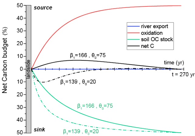
Figure 4: The modelled transient C budget of eroded organic carbon (partitioning between a CO 2 source or sink) over a seismic cycle of 270 years duration. Red lines are the CO 2 source from oxidation of the mobilized OC. Green lines indicate CO 2 sequestration by the re-establishment of the soil OC stocks in the landscape, which is based on a model of above ground biomass accumulation. a. The case where only OC oxidation is accounted for. The parameters controlling the shape of the soil OC stock model are explored, and determine whether landsliding is a net C source (solid black line) or net sink (solid dashed line). b. The case where OC oxidation and fluvial export are both active. Here, the parameters controlling the physical export of sediment ( t_0 and t_{con} ) are explored. Solid lines correspond to t_0 = 100 yr and t_{con} = 50 yr, and result in a short-term C source but long-term sequestration. Dashed lines correspond to t_0 = 20 yr and t_{con} = 10 yr, and result in net sequestration over the entire seismic cycle.
