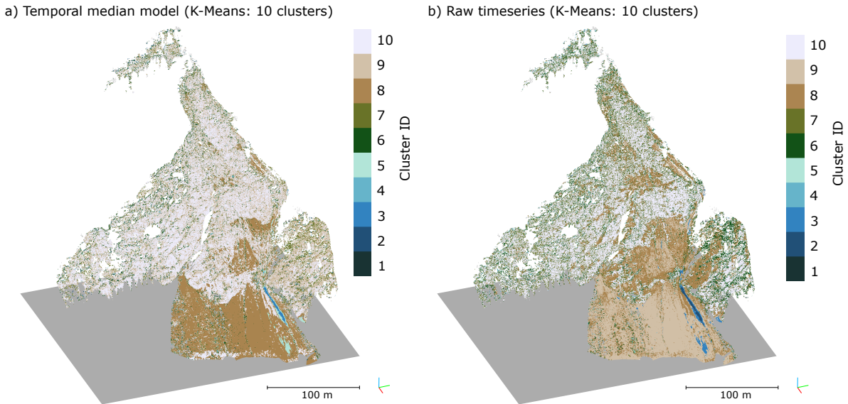
Figure 12. Comparison of clustering results from time series estimated using different state-of-the-art methods. a) Temporal median model (window size of 96 hours), and b) the raw time series. The cluster numbers are assigned by point count, Cluster 10 being the largest cluster.
